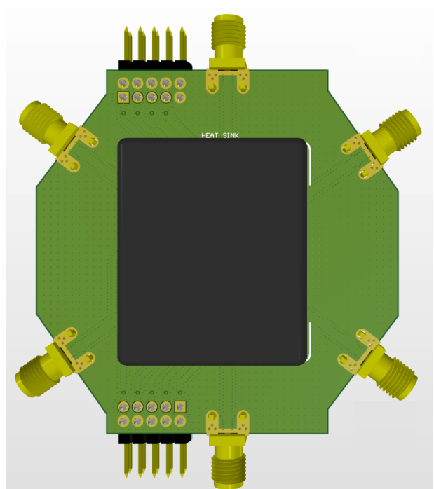
Bottom View
