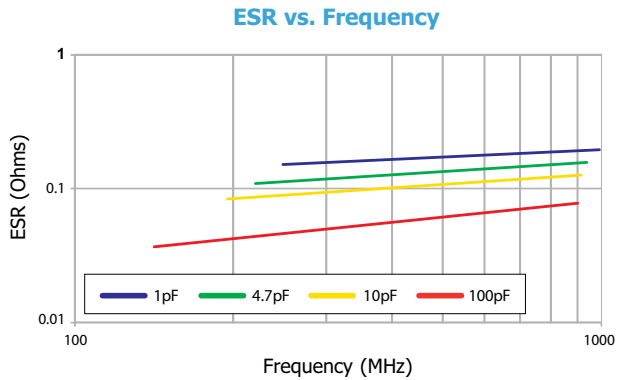
TYPICAL PERFORMANCE DATA — CHIP SIZE 0805 HIGH Q
