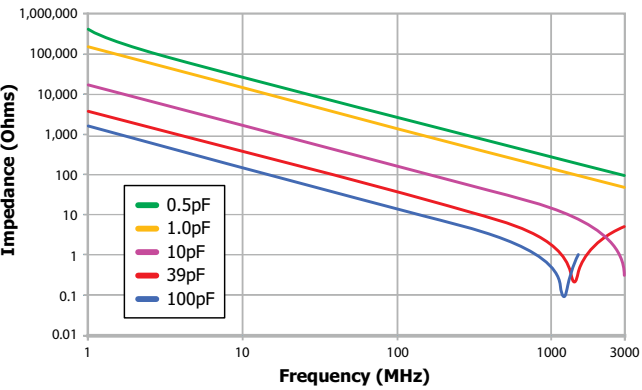
Q Series — Impedance vs. Frequency — Case Size 0505
