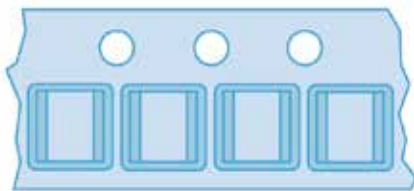
Orientation of 182 & 2225 components
