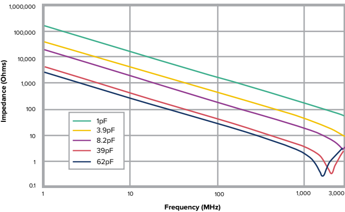
0805 H SERIES ESR vs. FREQUENCY
