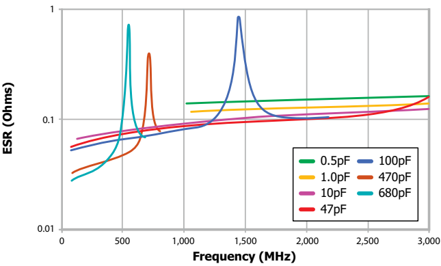
Q Series — ESR vs. Frequency — Case Size 1111
