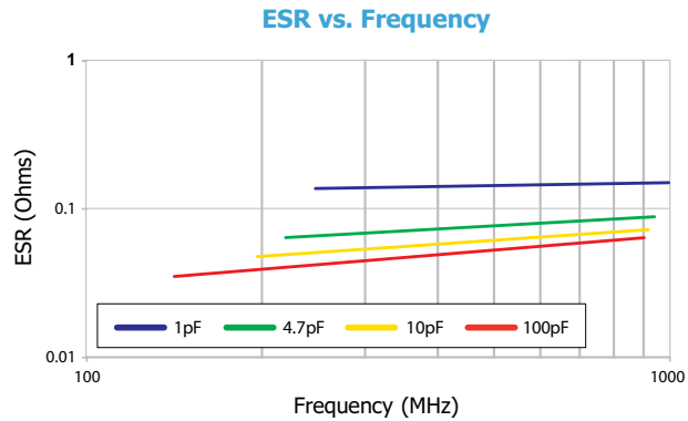
TYPICAL PERFORMANCE DATA — CHIP SIZE 1111 HIGH Q
