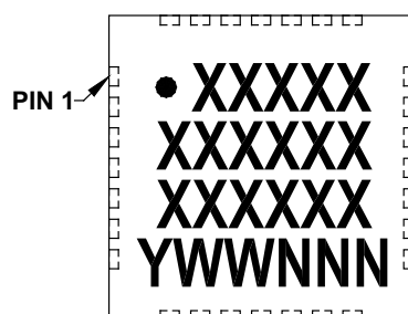
28-Lead VQFN (4x4mm)
