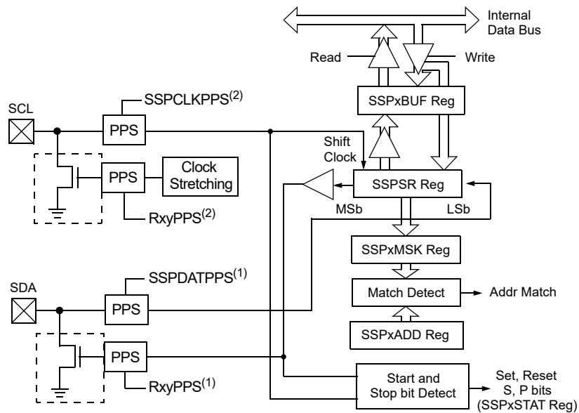
FIGURE 31-3: MSSP BLOCK DIAGRAM (I 2 C CLIENT MODE)
