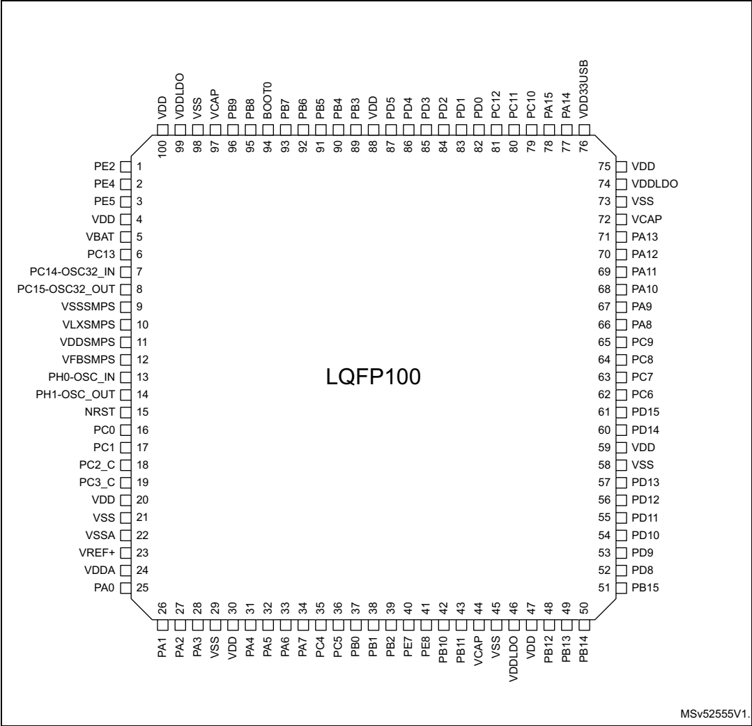
Figure 6. LQFP100 pinout
