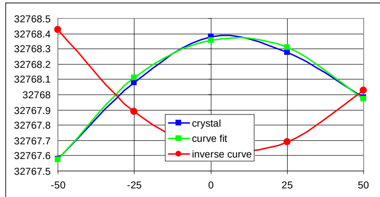
Figure 30: Crystal Compensation
