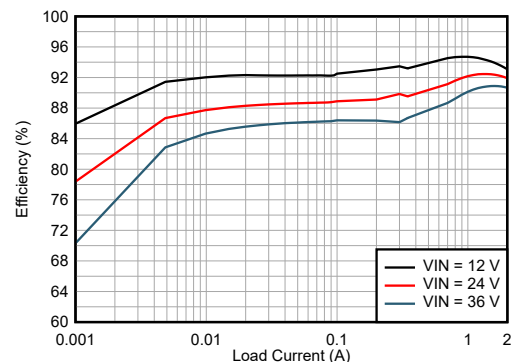
Efficiency: V_{\text{OUT}} = 5 \text{ V} (Fixed), 1 MHz
