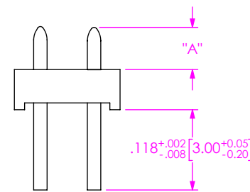
SHEAR VIEW FOR 05 & 06 LEAD STYLE
