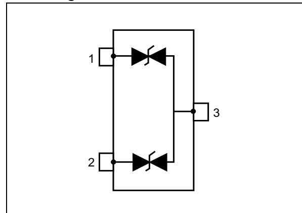
Figure 1. Functional schematic
