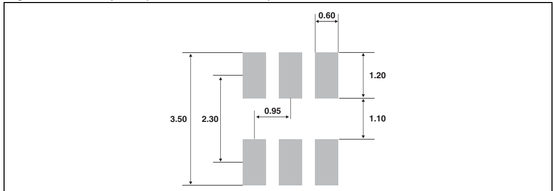
Figure 10. Footprint (dimensions in mm)
