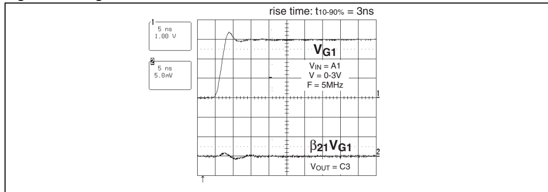
Figure 9. Digital crosstalk
