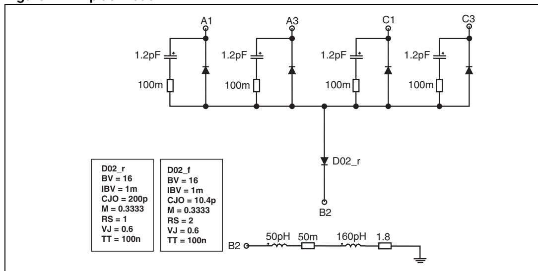
Figure 11. Aplac model
