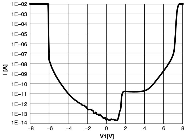
Figure 9. IV Characteristics
