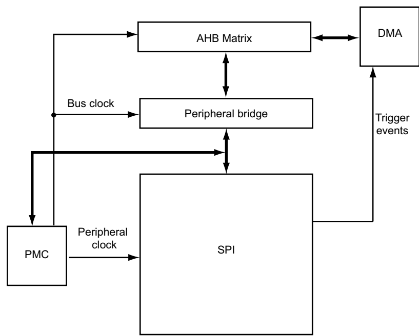
Figure 39-1: Block Diagram
