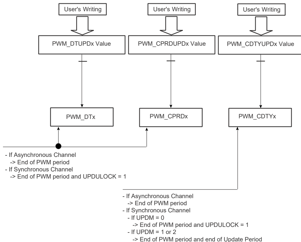
Figure 47-17: Synchronized Period, Duty-Cycle and Dead-Time Update
