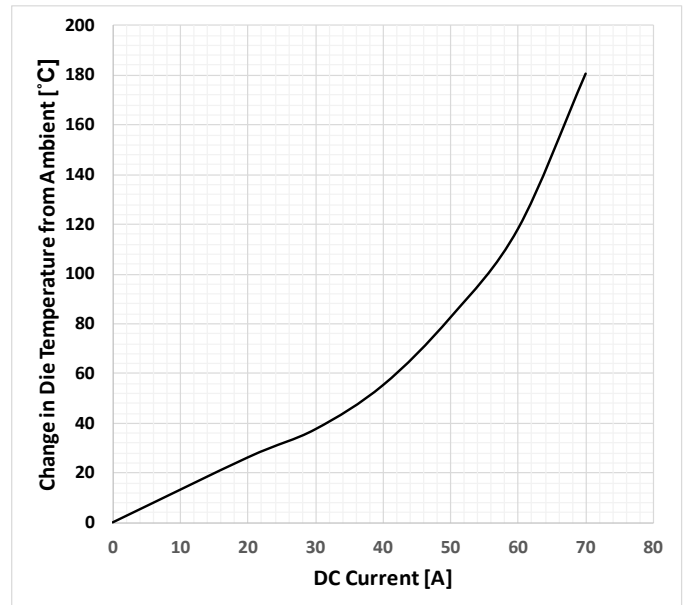
Figure 21: Self Heating in the LA Package Due to Current Flow
