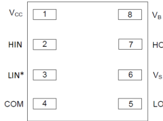
Top View: V-DFN3035-8
