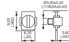
Screw + clamp
