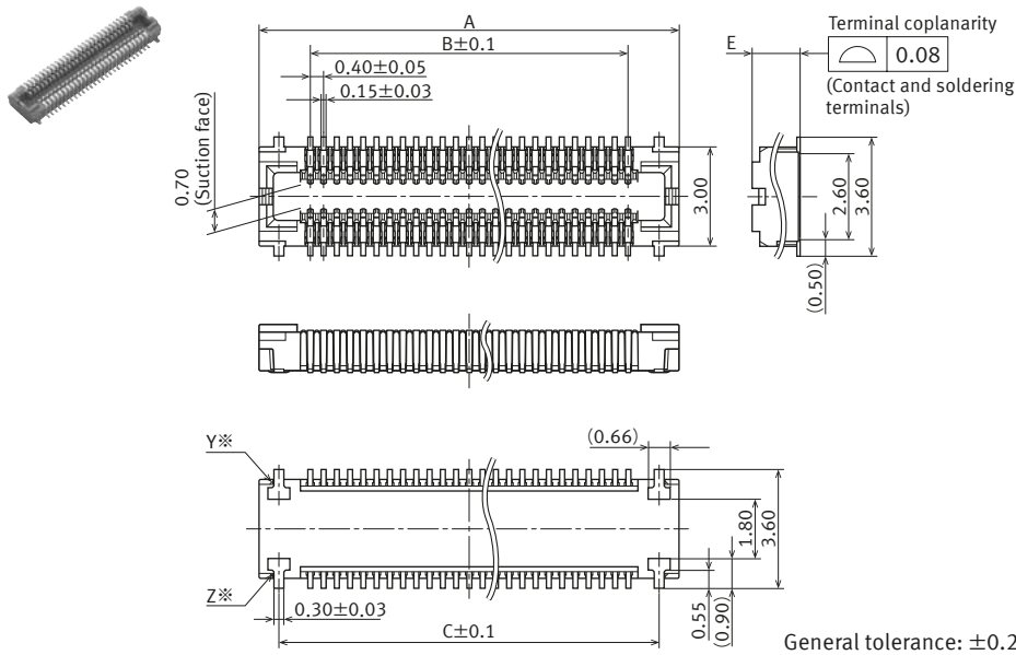
External dimensions
