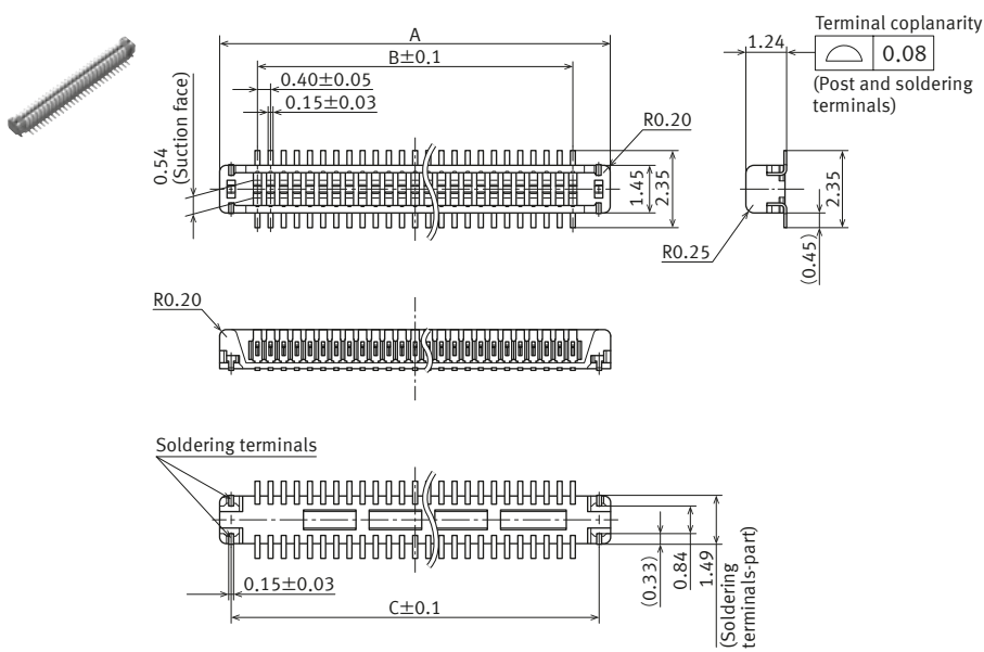
External dimensions
