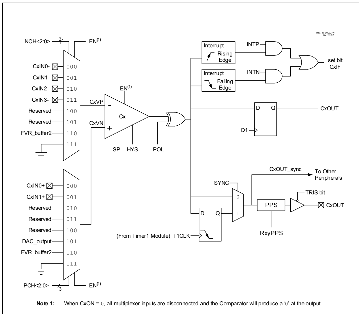
FIGURE 39-2: COMPARATOR MODULE SIMPLIFIED BLOCK DIAGRAM
