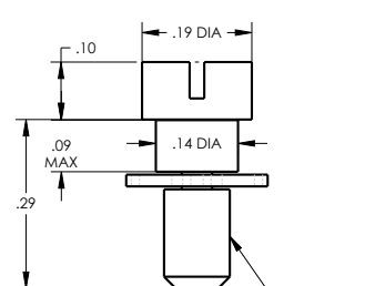
#4/40 M83513/05-13
