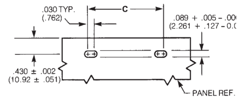
Figure 3: Edgeboard Mounting
