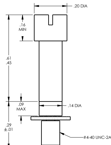
#4/40 M83513/05-16
