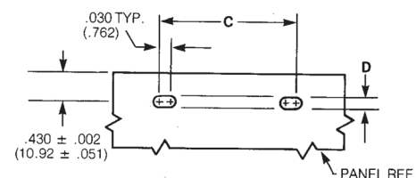
Figure 3: Edgeboard Mounting
