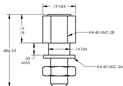
#4/40 M83513/05-17
