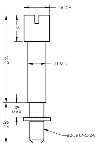
#2/56 M83513/05-06
