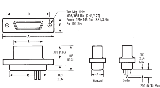
Plug
