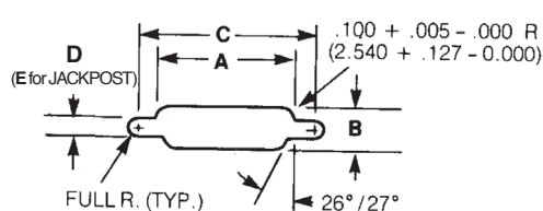
Figure 2: Rear Mounting
