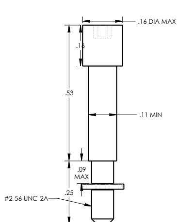
#2/56 M83513/05-05
