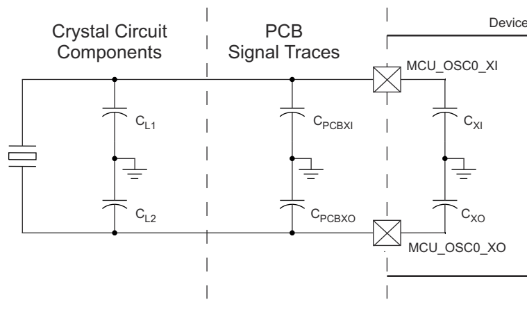
Figure 7-18. Load Capacitance
