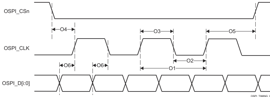
Figure 7-106. OSPI0 Switching Characteristics – Tap DDR, No Loopback
