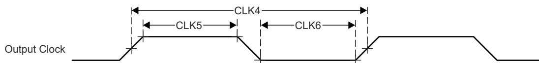
Figure 7-15. Clock Switching Characteristics
