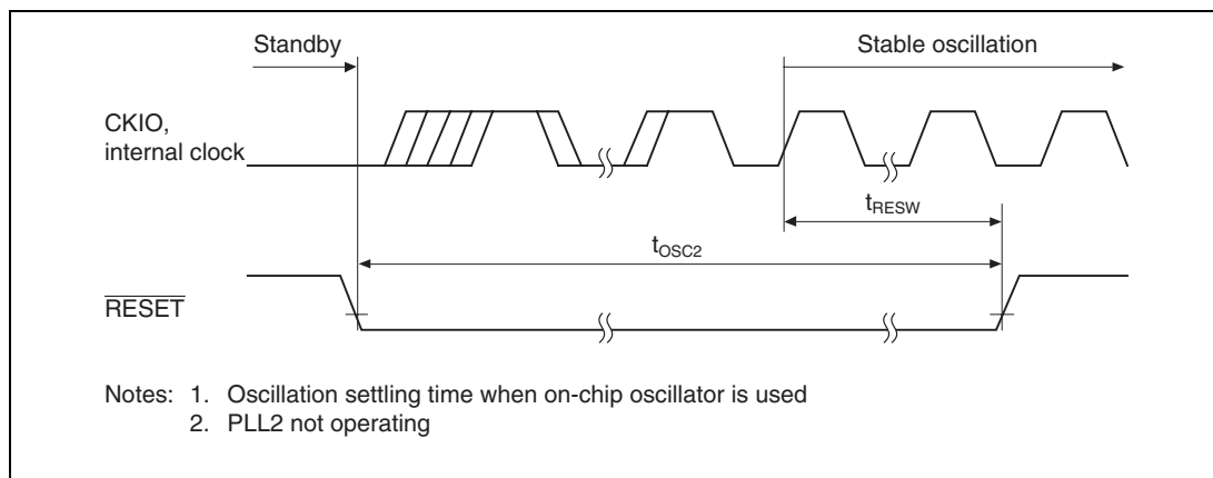
Figure 22.4 Standby Return Oscillation Settling Time (Return by \overline{RESET} )
