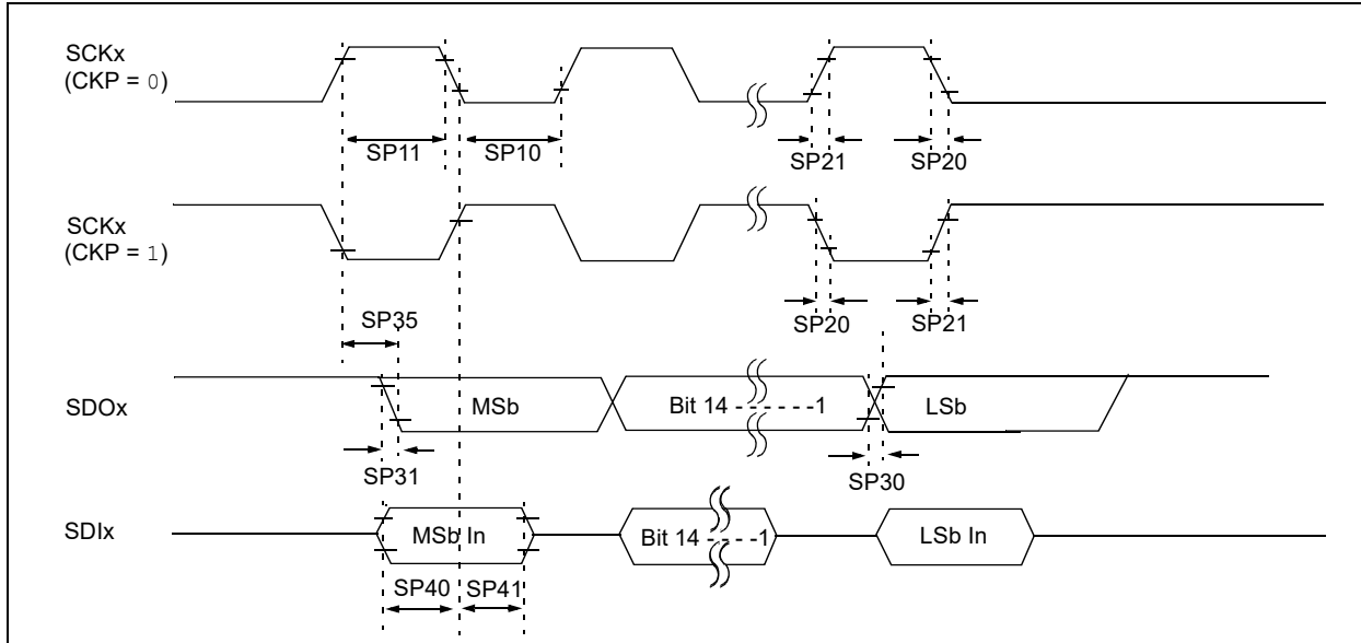
FIGURE 36-10: SPIx MODULE MASTER MODE (CKE = 0) TIMING CHARACTERISTICS
