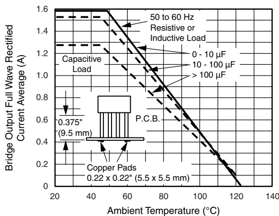
Fig. 2 - Derating Curves Output Rectified Current for B250C1500G...B380C1500G
