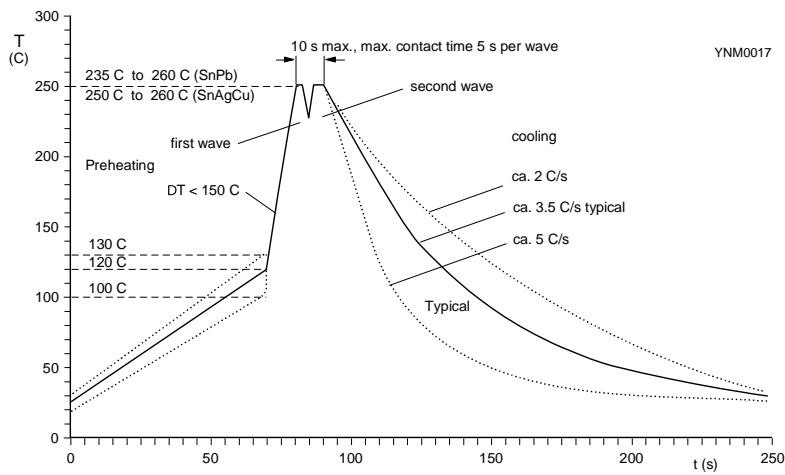
Solid line: Typical process Dotted lines: Process limits
