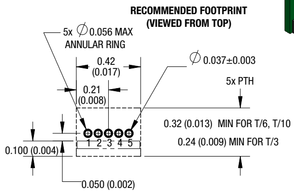
Figure 2. OKR Series Component locations are typical.
