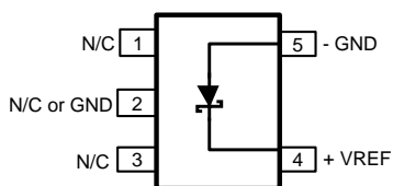
SOT-23 Package (Top View)
