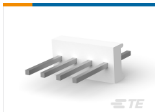
TE Part #1-640456-7 PCB Header: Polyester, Vertical, Unshrouded, No Mating Alignment
