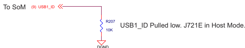
Figure 4-30. USB1 ID Setting for HUB
