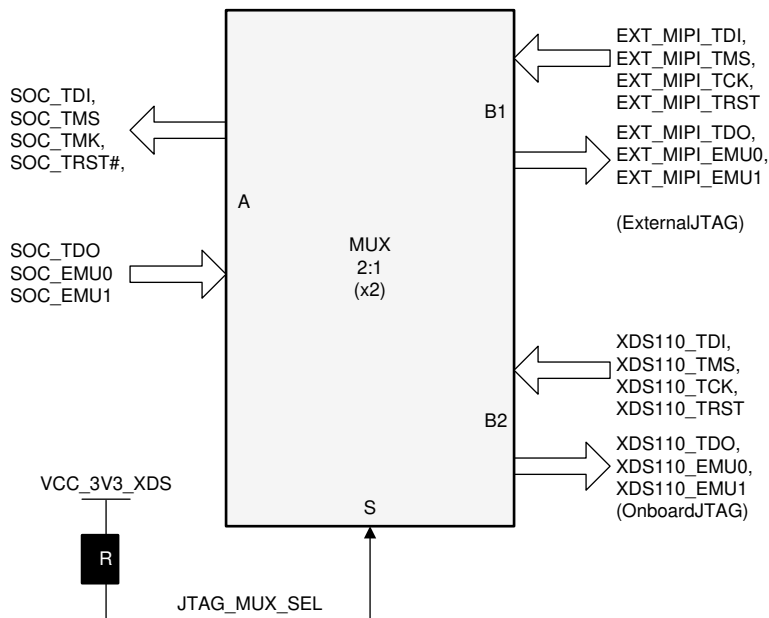
Figure 3-8. JTAG Mux
