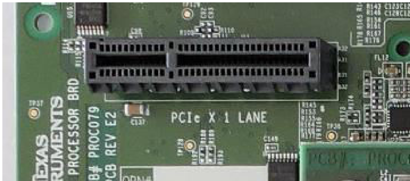
Figure 4-19. PCIe Interface for SERDES0
