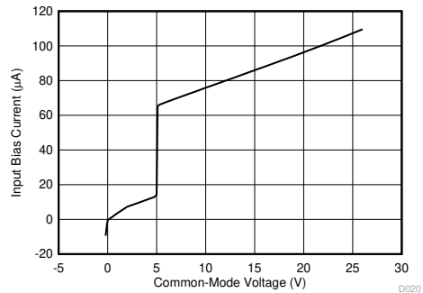
Figure 6-20. Input Bias Current vs. Common-Mode Voltage
