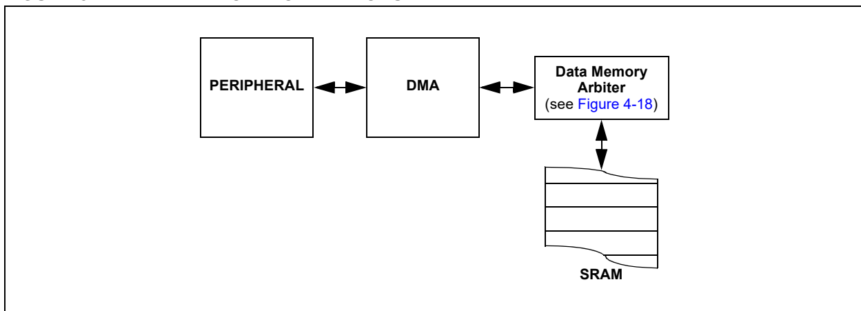
FIGURE 8-1: DMA CONTROLLER MODULE
