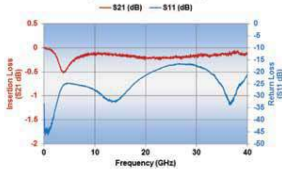
P21BN300MA4282 Opti-Cap Typical Performance (Reference 50 Ohm System)
