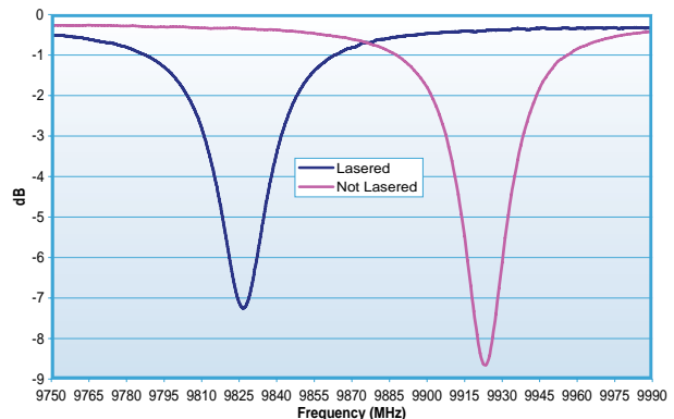
9.9GHz Resonator - Before & After Laser
