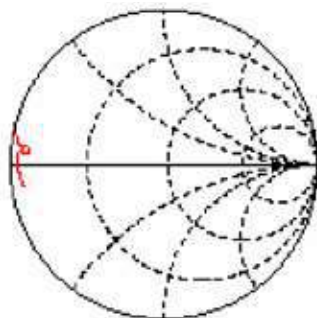
Typical S11 Frequency Range: 1.0 to 20 GHz Reflection Coefficient: 50 \Omega Normalized
