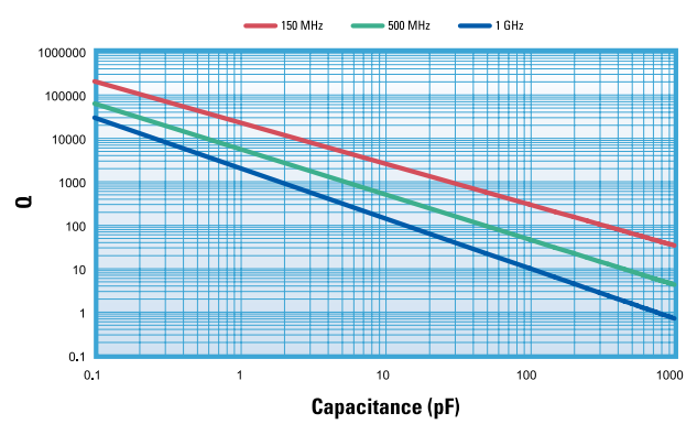
Q vs Capacitance DLI C17 AH Series
