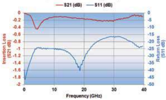
P21BN300MA3976 Opti-Cap Typical Performance (Reference 50 Ohm System)
