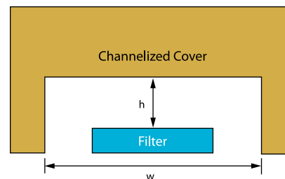
Housing dimensions critically affect performance
