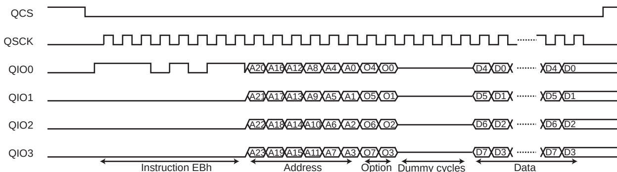
Figure 41-8. Instruction Frame
