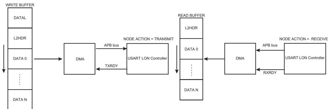
Figure 45-63. DMAM = 1
