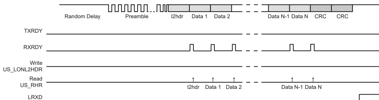
Figure 45-62. Rx Frame
