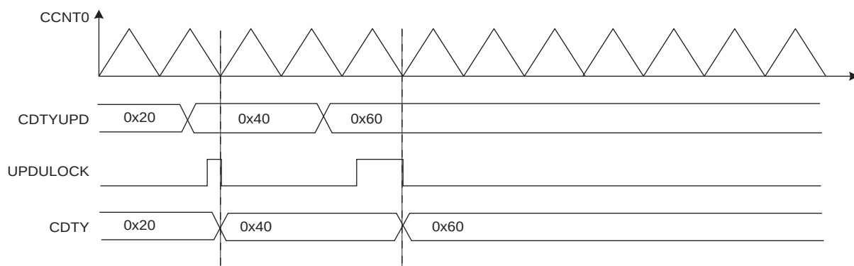
Figure 50-19. Method 1 (UPDM = 0)
