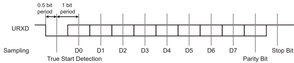
Figure 46-4. Character Reception
