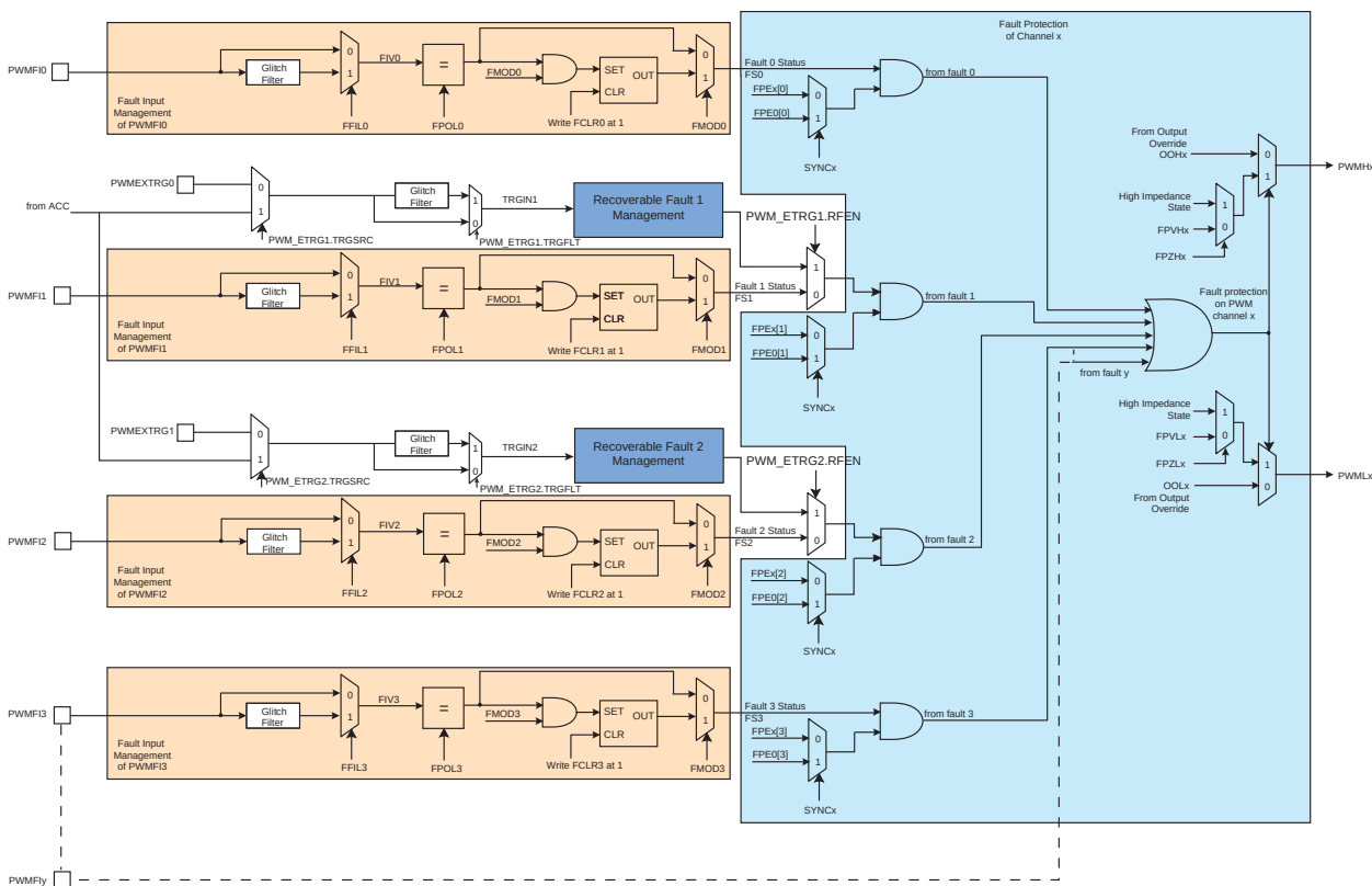
Figure 50-16. Fault Protection
