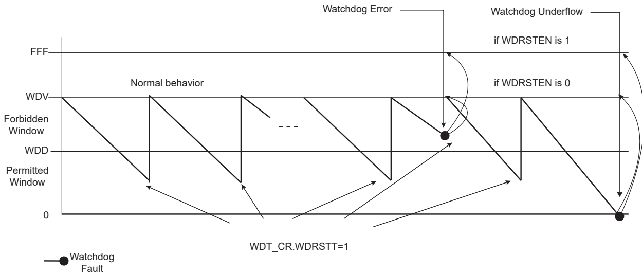
Figure 24-2. Watchdog Behavior
