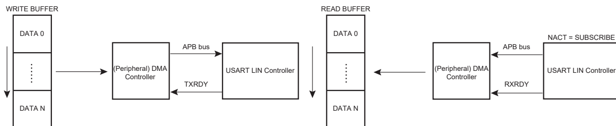
Figure 45-53. Client Node with DMAC
