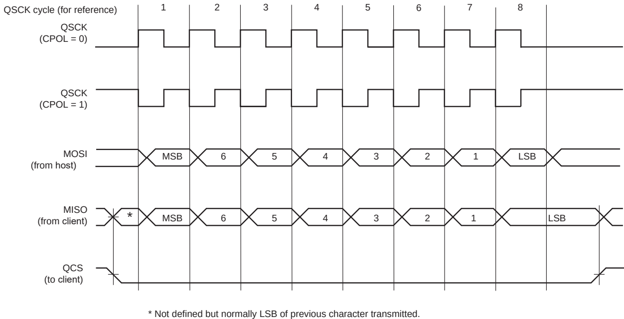
Figure 41-3. QSPI Transfer Format (QSPI_SCR.CPHA = 1, 8 bits per transfer)
