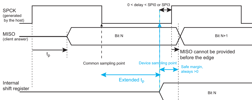
Figure 57-19. MISO Capture in Host Mode
