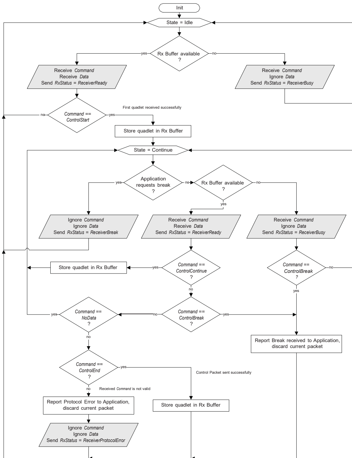
Figure 47-9. Control Packet Rx Device Protocol
