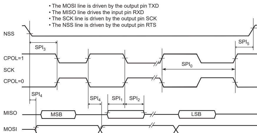
Figure 58-24. USART SPI Host Mode
