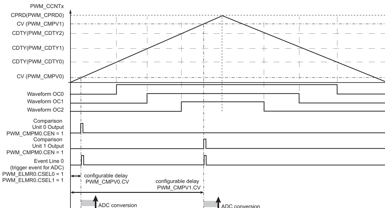
Figure 50-26. Event Line Generation Waveform (Example)
