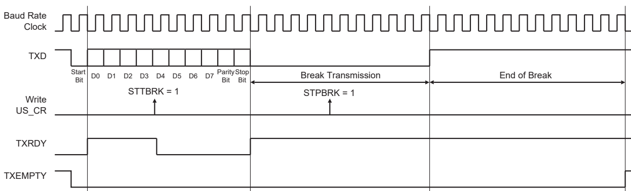
Figure 45-25. Break Transmission
