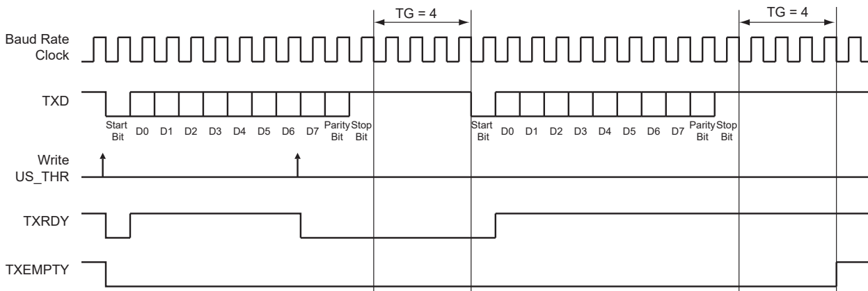
Figure 45-22. Timeguard Operations
