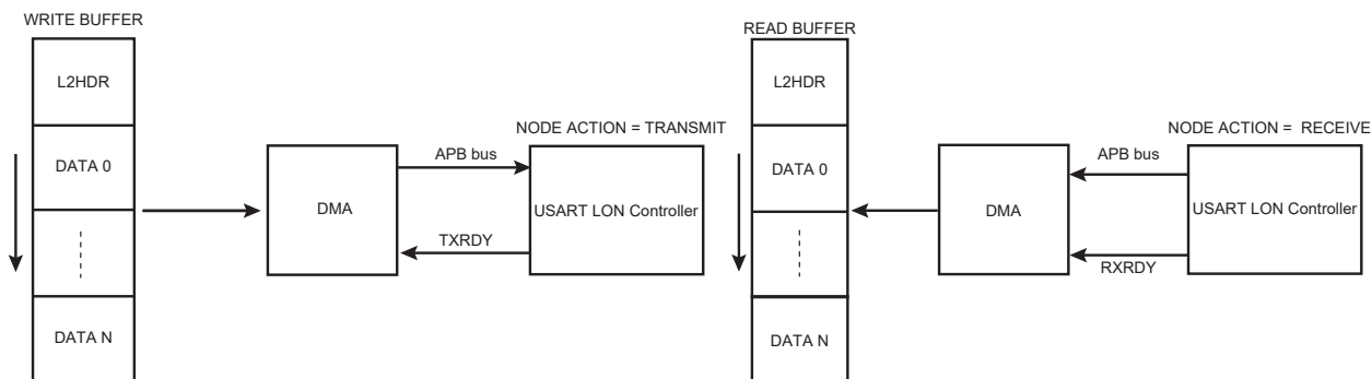
Figure 45-64. DMAM = 0
