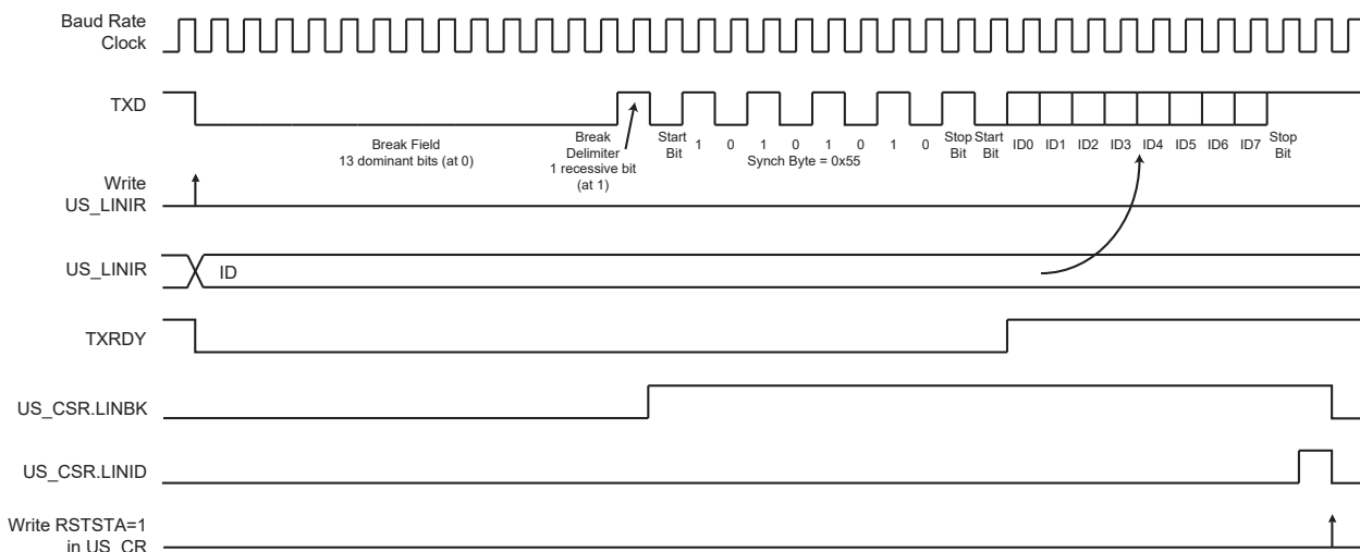
Figure 45-39. Header Transmission
