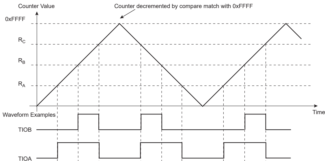
Figure 49-12. WAVSEL = 01 without Trigger
