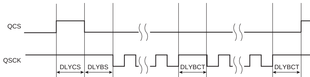
Figure 41-4. Programmable Delays
