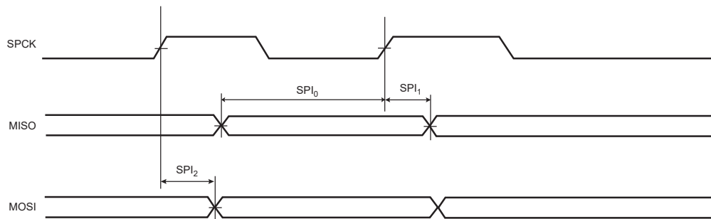
Figure 57-21. SPI Host Mode with (CPOL = 0 and NCPHA=1) or (CPOL=1 and NCPHA= 0)
