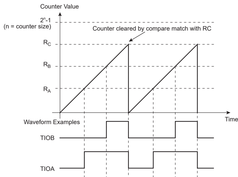
Figure 49-10. WAVSEL = 10 without Trigger
