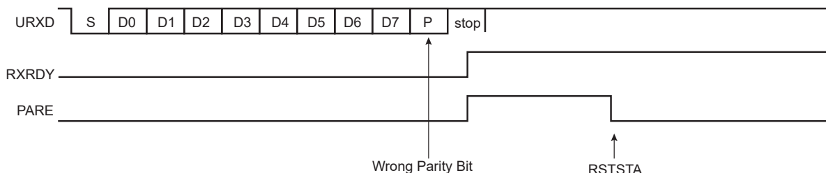
Figure 46-7. Parity Error
