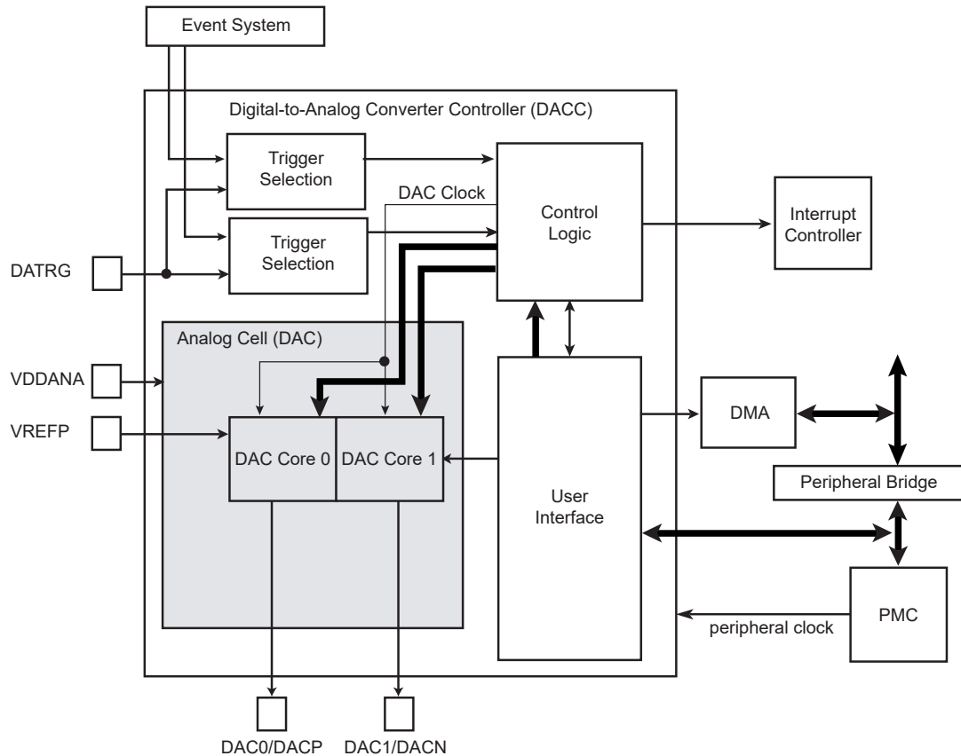
Figure 52-1. Block Diagram
