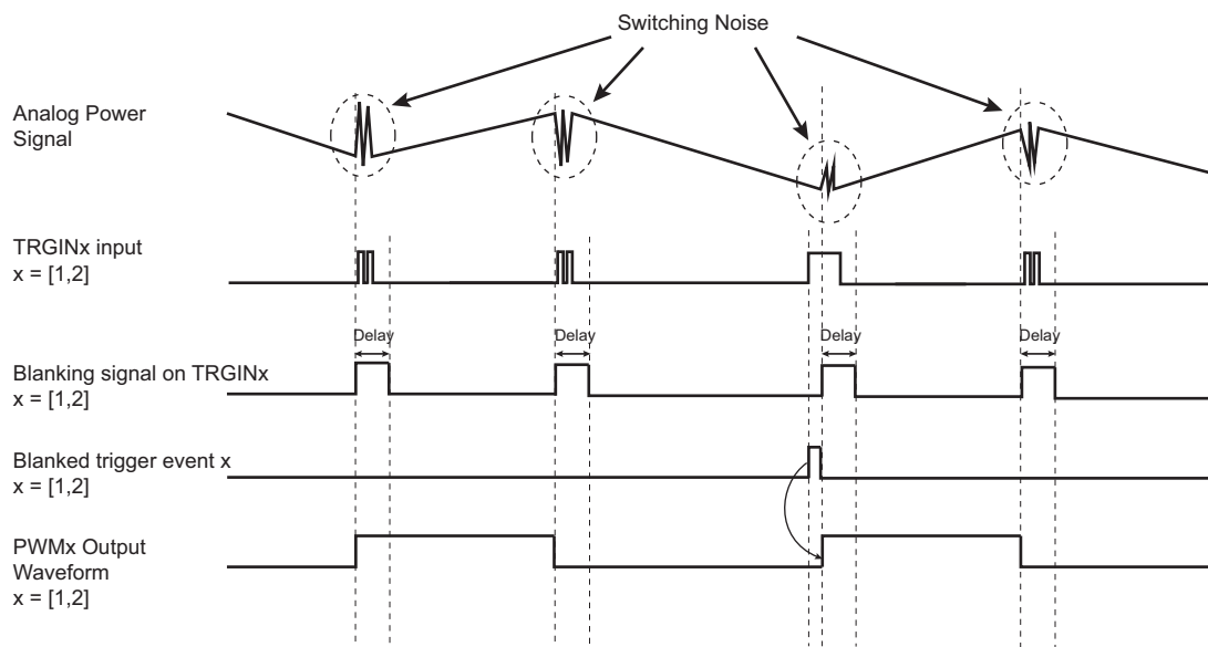
Figure 50-33. Leading-Edge Blanking
