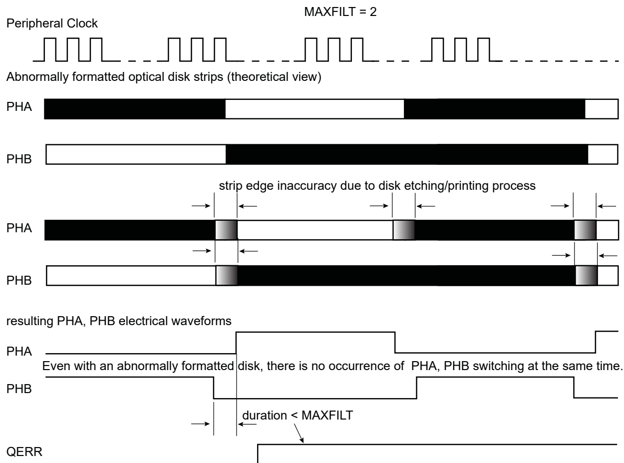
Figure 49-21. Quadrature Error Detection
