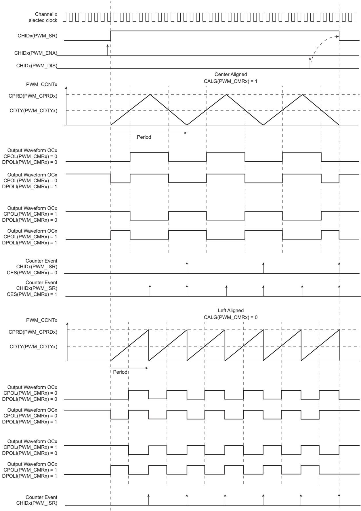
Figure 50-5. Waveform Properties
