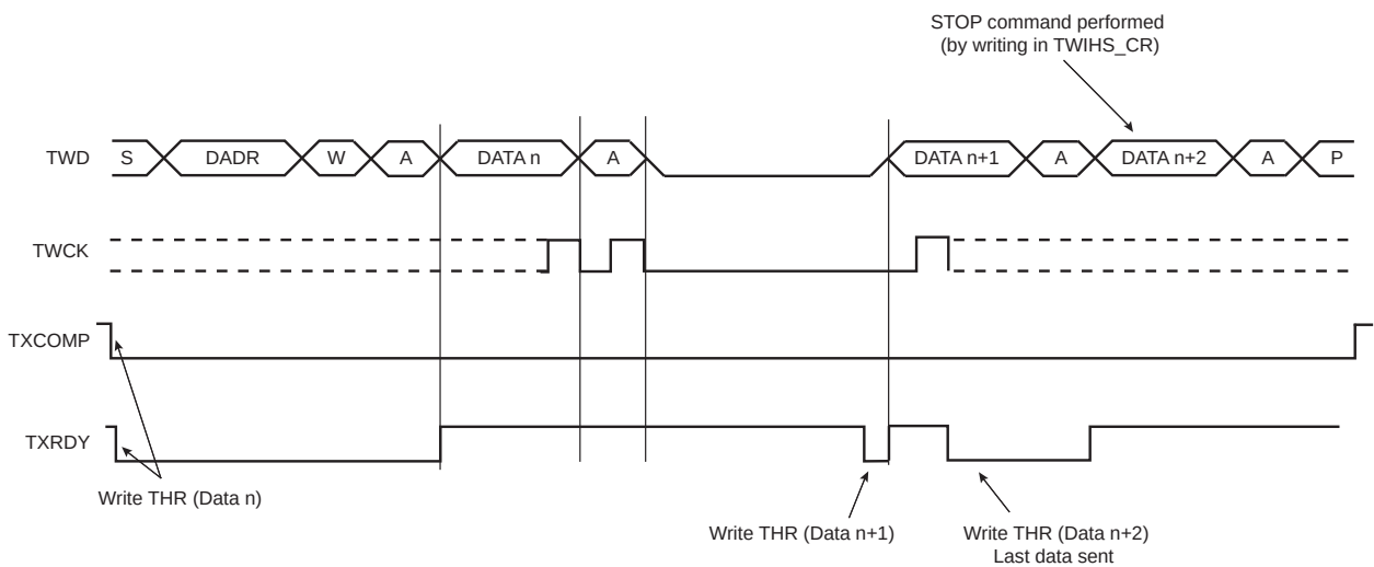
Figure 42-5. Host Write with Multiple Data Bytes
