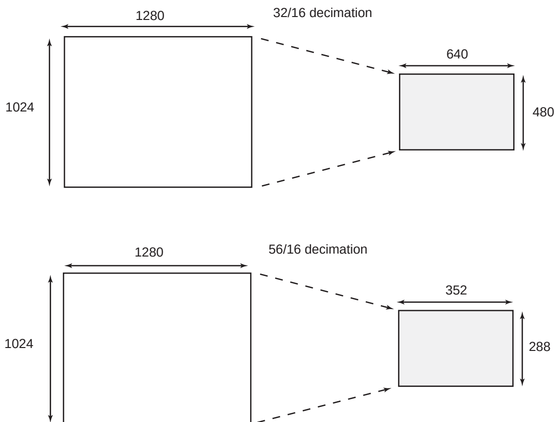
Figure 36-5. Resize Examples
