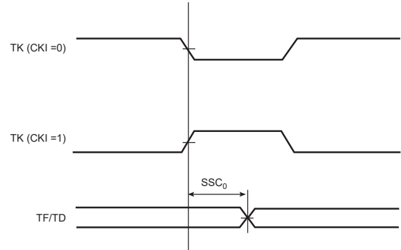
Figure 58-31. SSC Transmitter, TK and TF in Output
