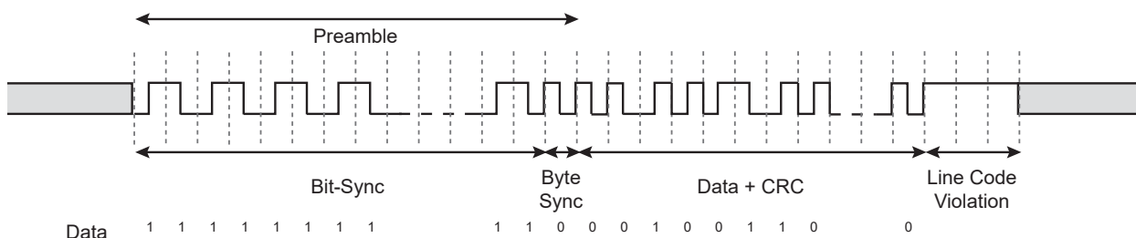
Figure 45-55. LON Framing
