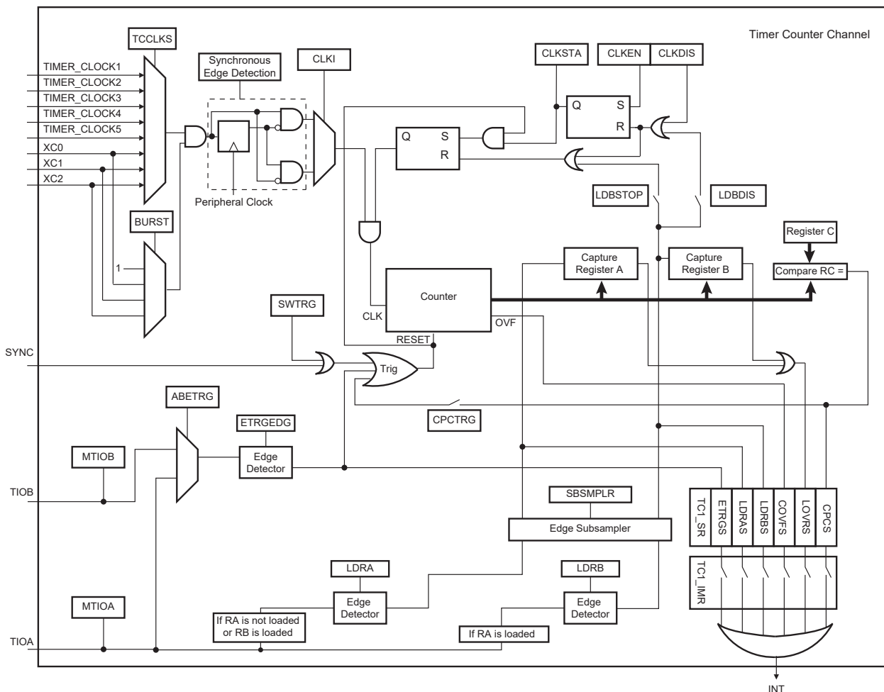
Figure 49-6. Capture Mode
