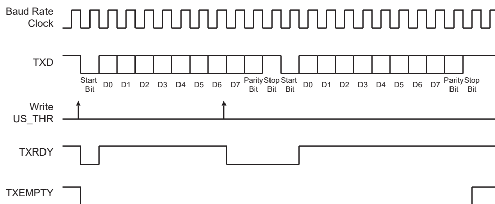
Figure 45-6. Transmitter Status
