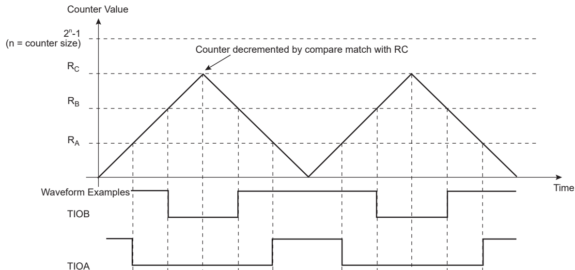
Figure 49-14. WAVSEL = 11 without Trigger
