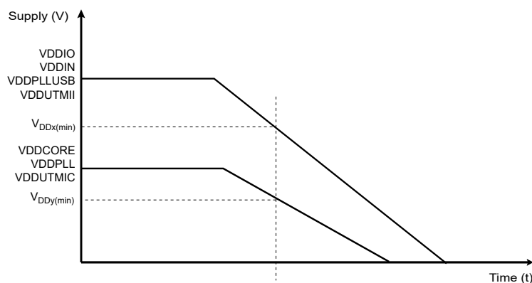
Figure 7-2. Powerdown Sequence
