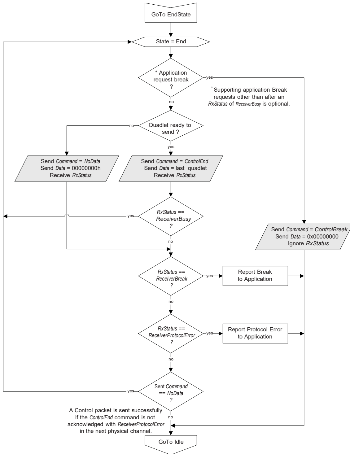
Figure 47-8. Control Packet Tx Device Protocol: End
