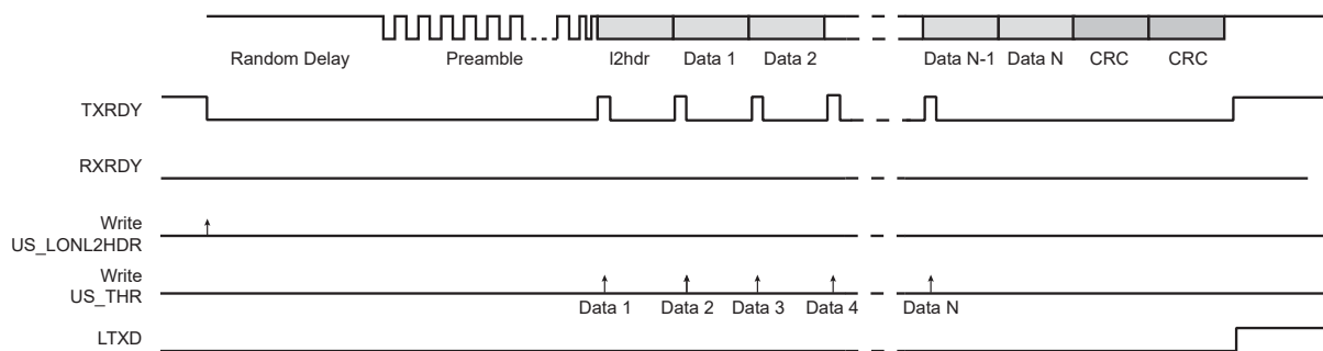
Figure 45-61. Tx Frame
