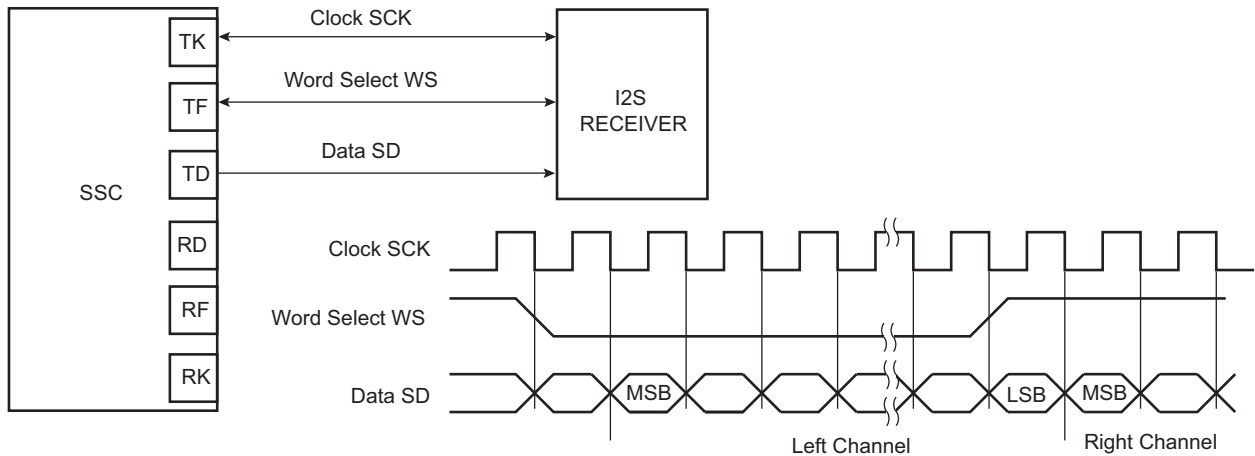
Figure 43-3. Audio Application Block Diagram
