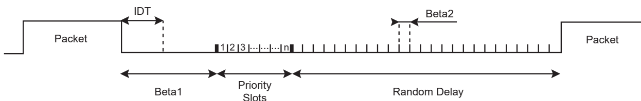
Figure 45-59. LON Timings
