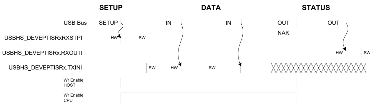
Figure 38-10. Control Read
