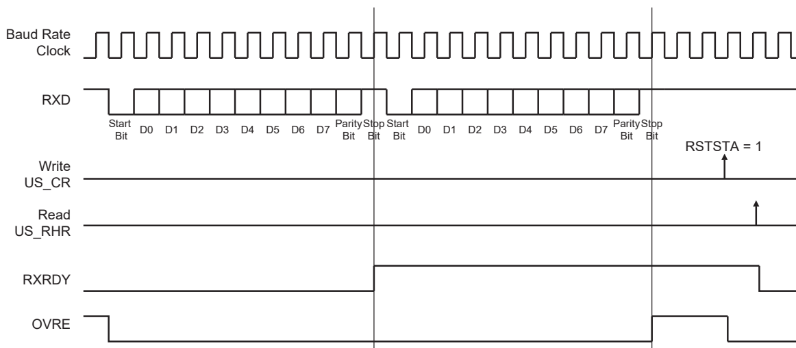
Figure 45-20. Receiver Status
