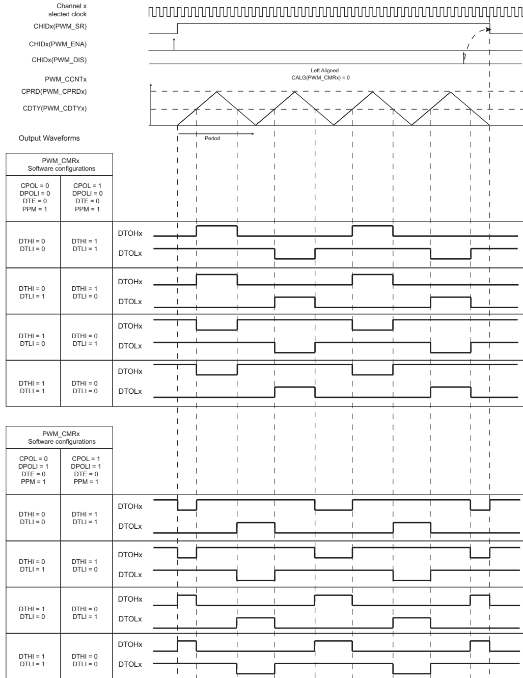
Figure 50-12. PWM Push-Pull Waveforms: Center-Aligned Mode
