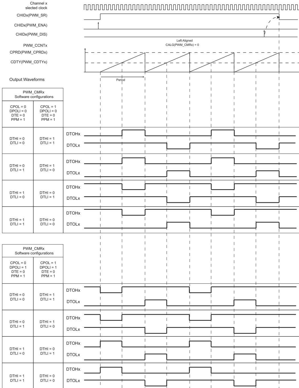
Figure 50-11. PWM Push-Pull Waveforms: Left-Aligned Mode
