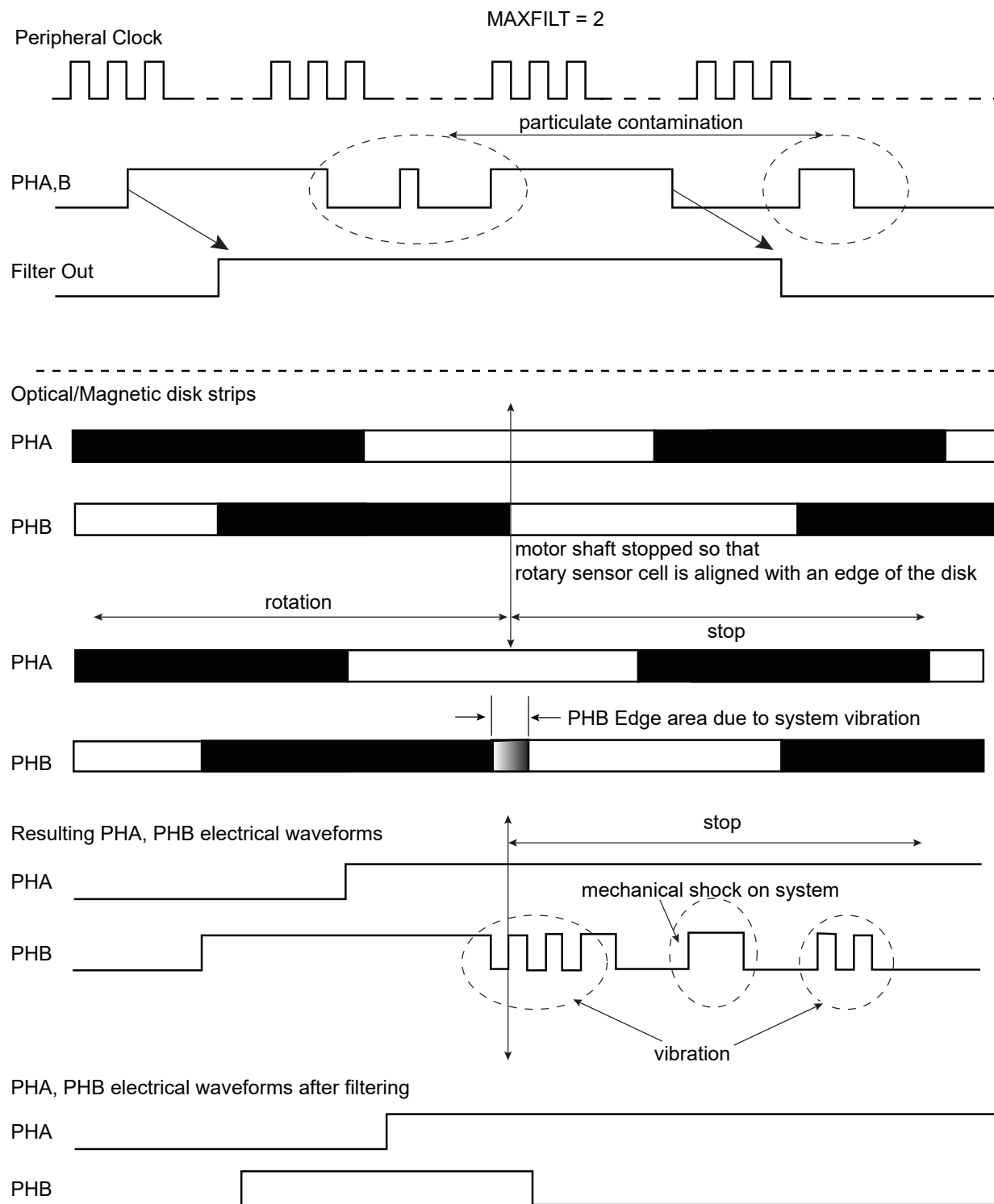
Figure 49-19. Filtering Examples
