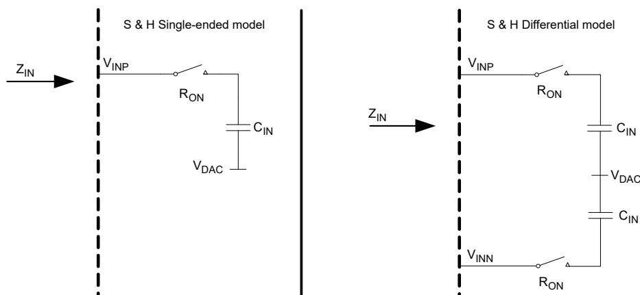
Figure 57-15. Input Channel Model
