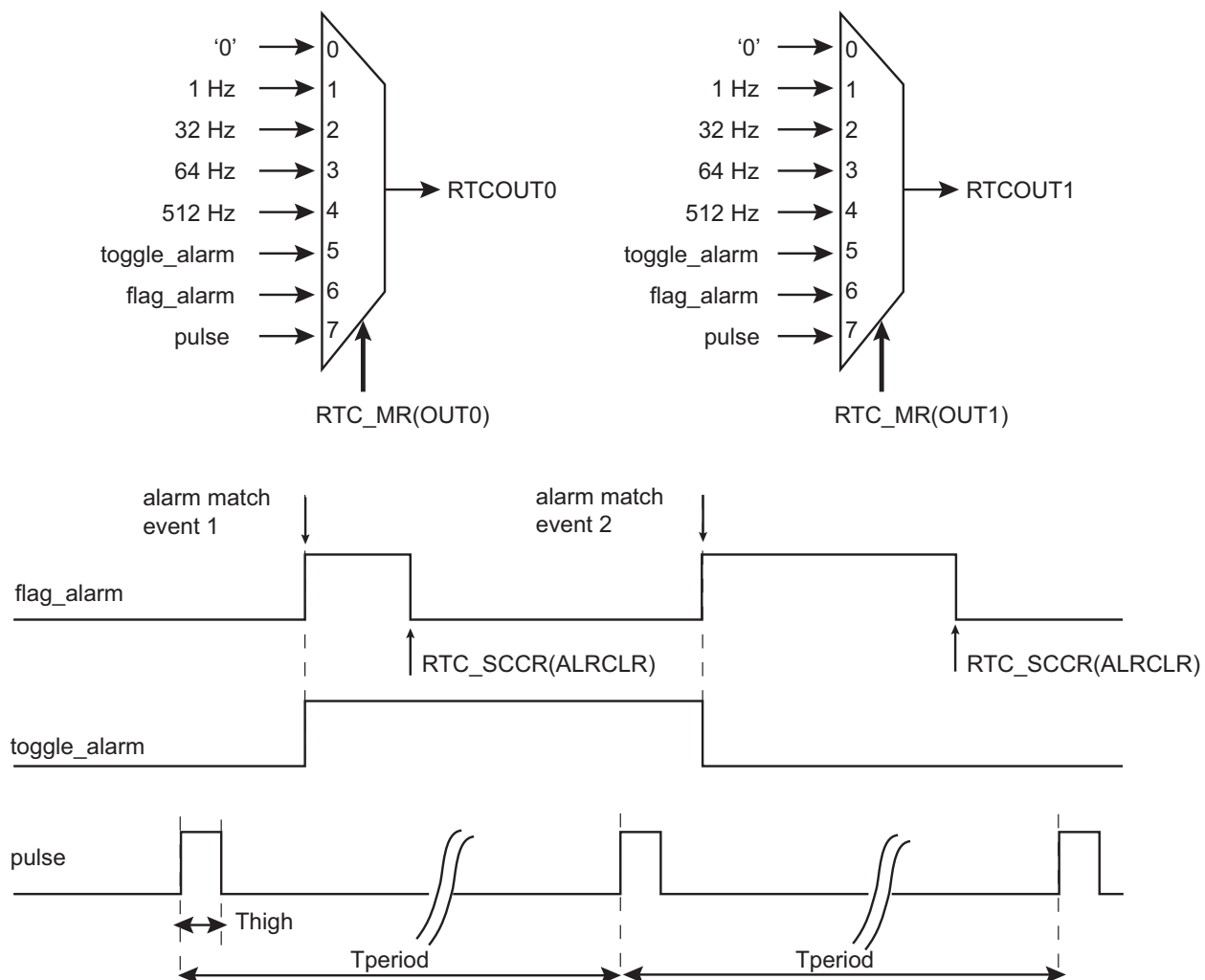
Figure 27-6. Waveform Generation
