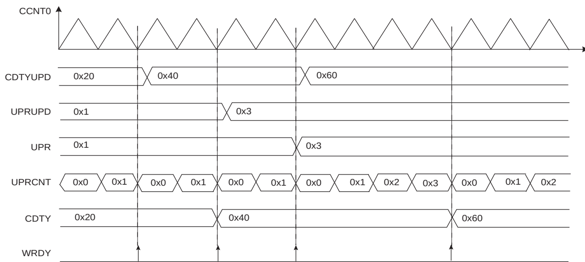
Figure 50-20. Method 2 (UPDM = 1)
