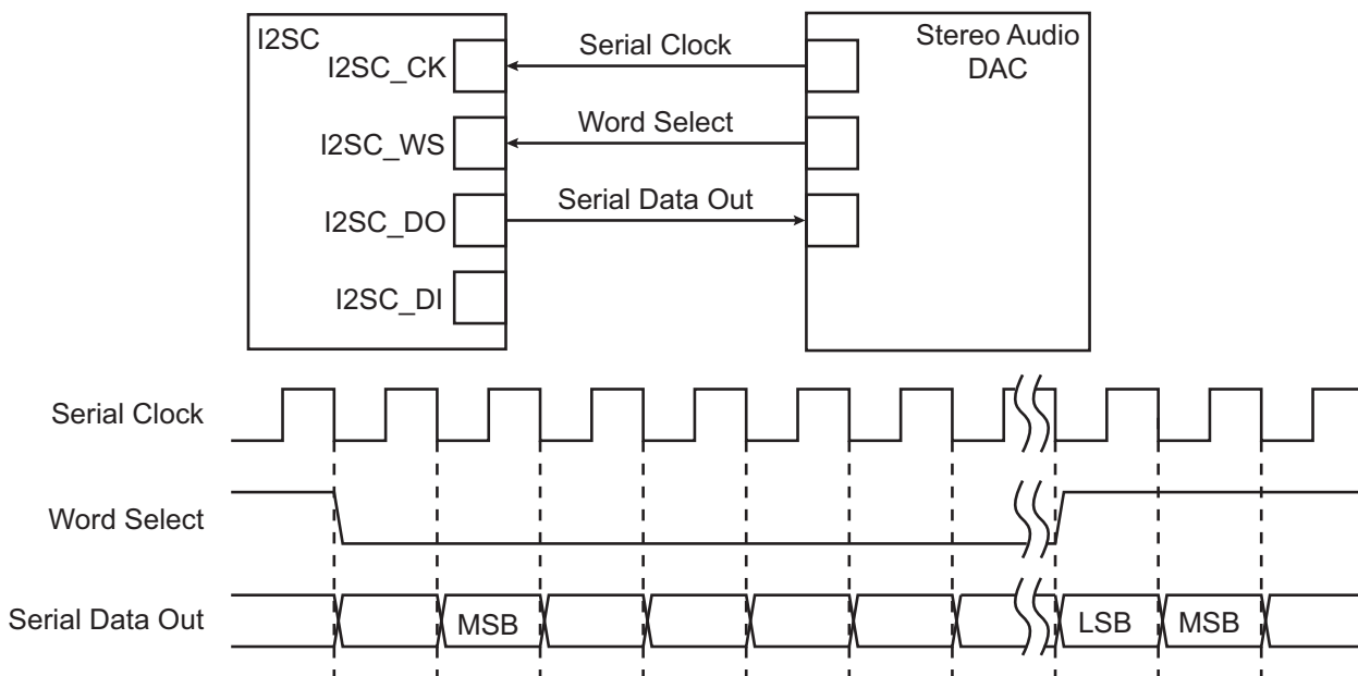
Figure 44-5. Client Transmitter I2SC Application Example
