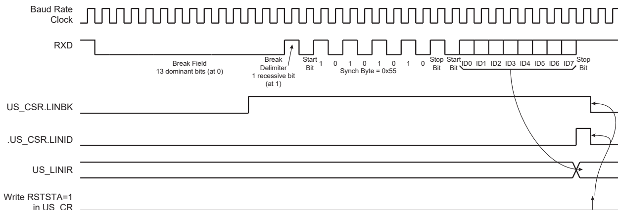
Figure 45-40. Header Reception
