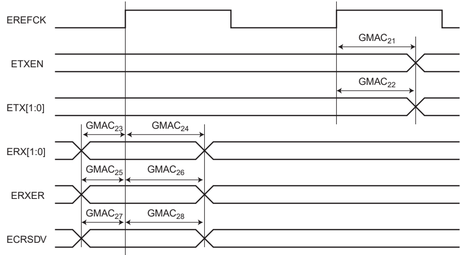
Figure 58-30. GMAC RMII Mode Signals
