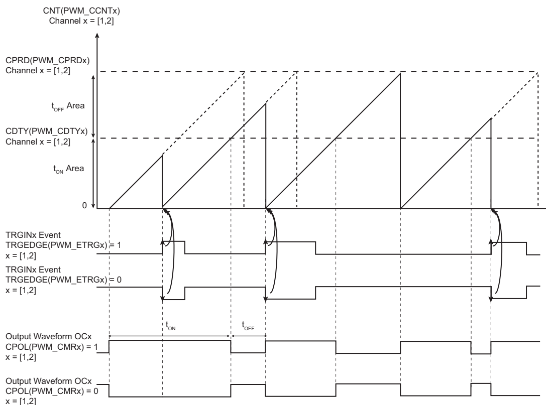
Figure 50-27. External PWM Reset Mode
