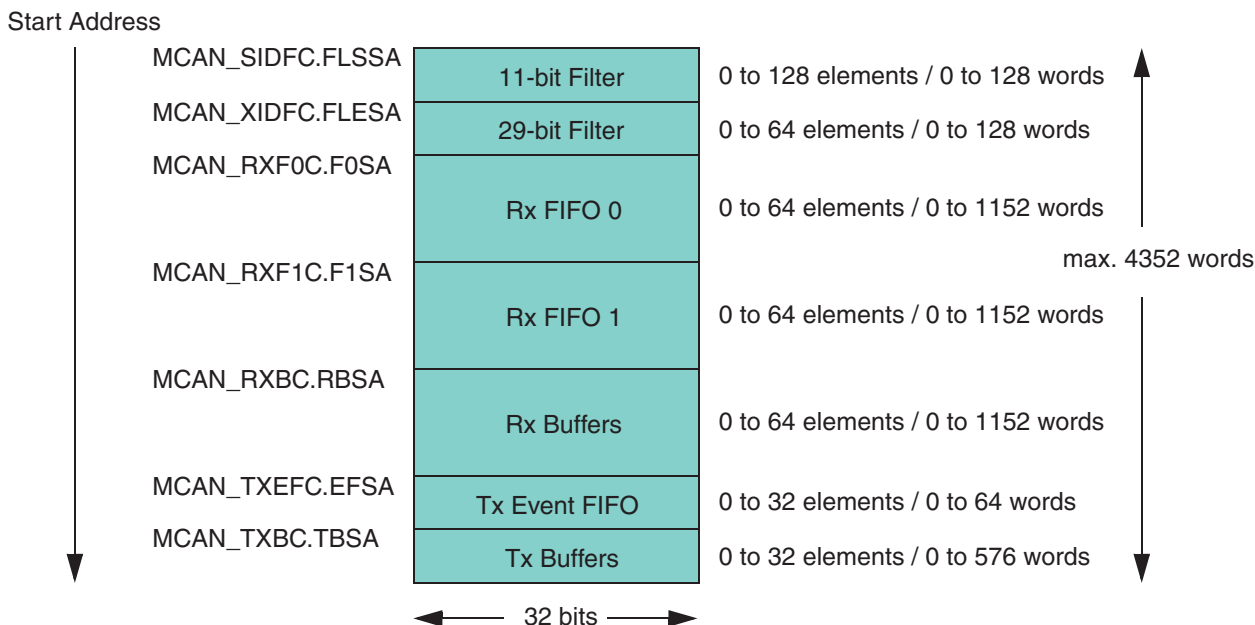
Figure 48-12. Message RAM Configuration
