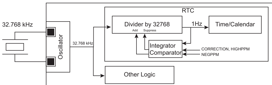
Figure 27-4. Calibration Circuitry
