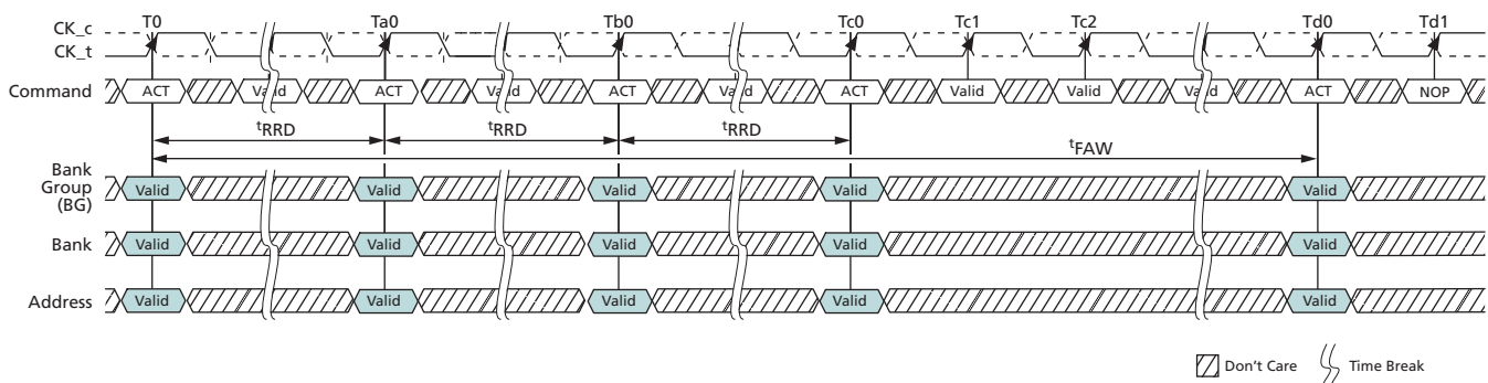
Figure 82: t_{FAW} Timing
