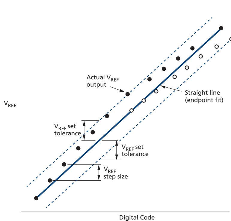
Figure 65: Example of V_{\text{REF}} Set Tolerance and Step Size
