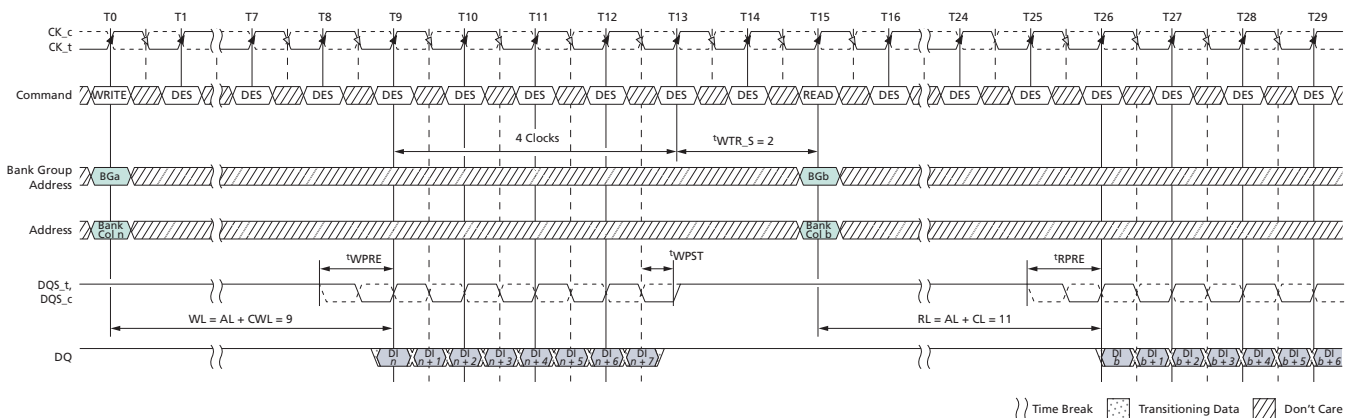
Figure 183: WRITE (BL8) to READ (BL8) with 1^{\text{t}} CK Preamble in Different Bank Group
