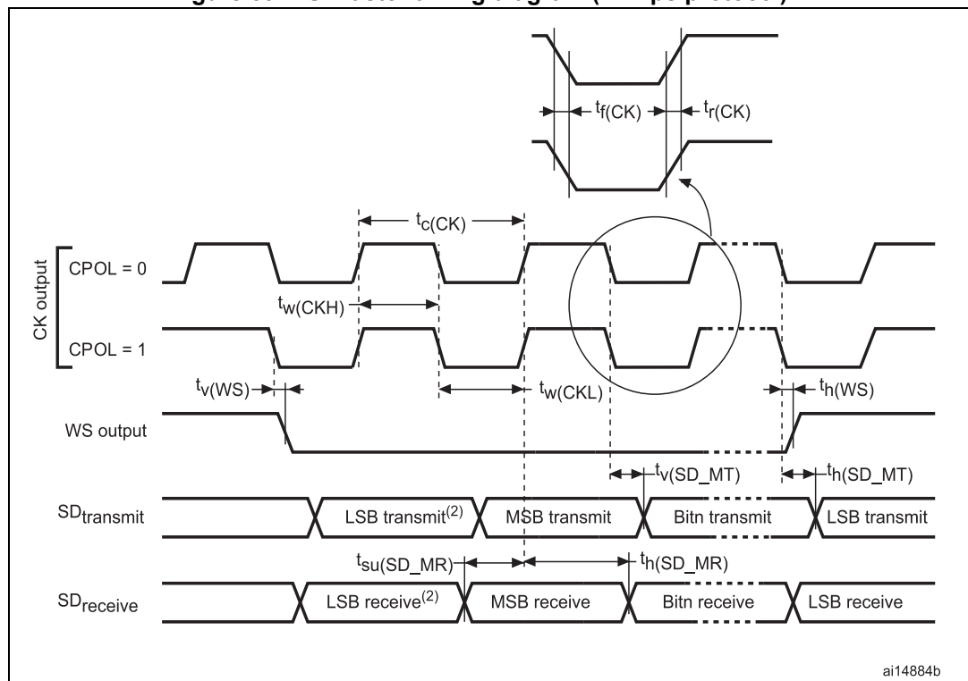
Figure 59. I²S master timing diagram (Philips protocol) (1)
