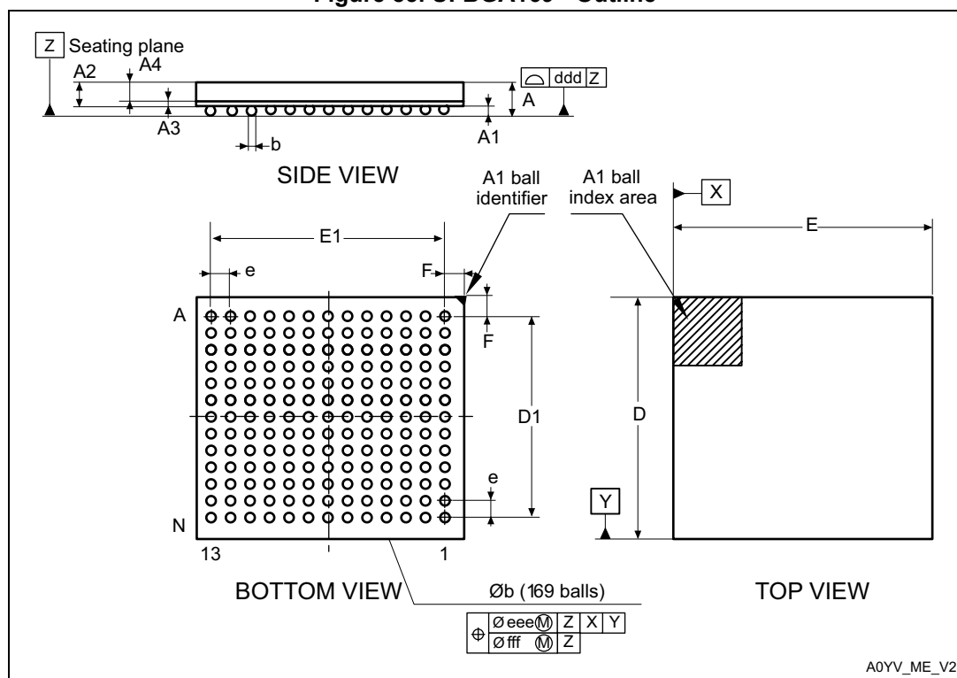
Figure 85. UFBGA169 - Outline
