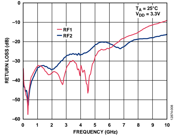
Figure 21. Return Loss vs. Frequency ( V_{DD} = 3.3\text{ V} )
