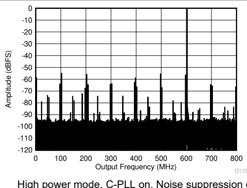
Figure 8-9. Single Tone FFT at 997 MHz and -1 dBFS
