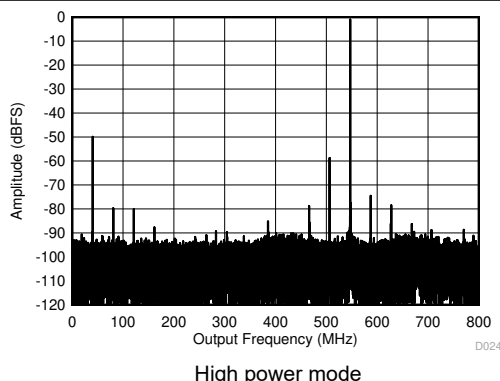
Figure 8-11. Single Tone FFT at 3797 MHz and -1 dBFS
