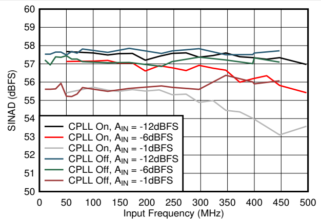
Figure 8-56. SINAD vs A_{IN} and C-PLL
