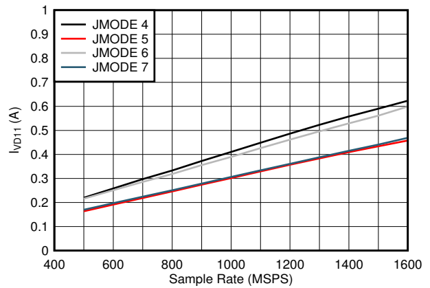
Figure 8-84. Quad Channel, I_{VDD11} vs F_S
