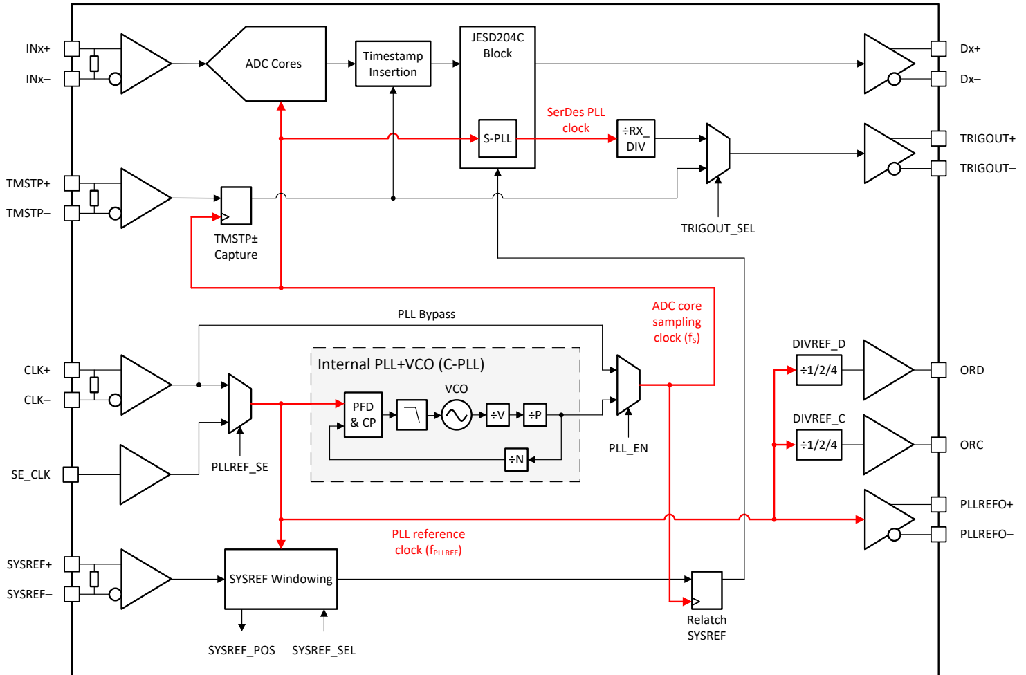
Figure 9-5. Clocking Subsystem
