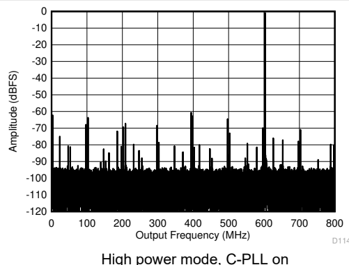
Figure 8-8. Single Tone FFT at 997 MHz and -1 dBFS
