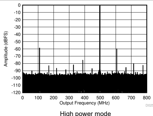
Figure 8-10. Single Tone FFT at 1797 MHz and -1 dBFS
