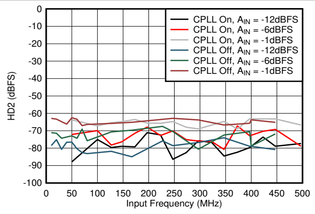
Figure 8-58. HD2 vs A_{IN} and C-PLL
