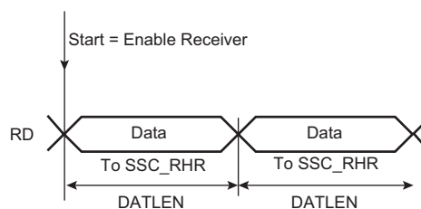
Figure 32-18. Receive Frame Format in Continuous Mode (STTDLY = 0)
