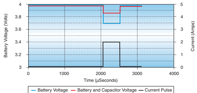
Figure 5. GSM Pulse
