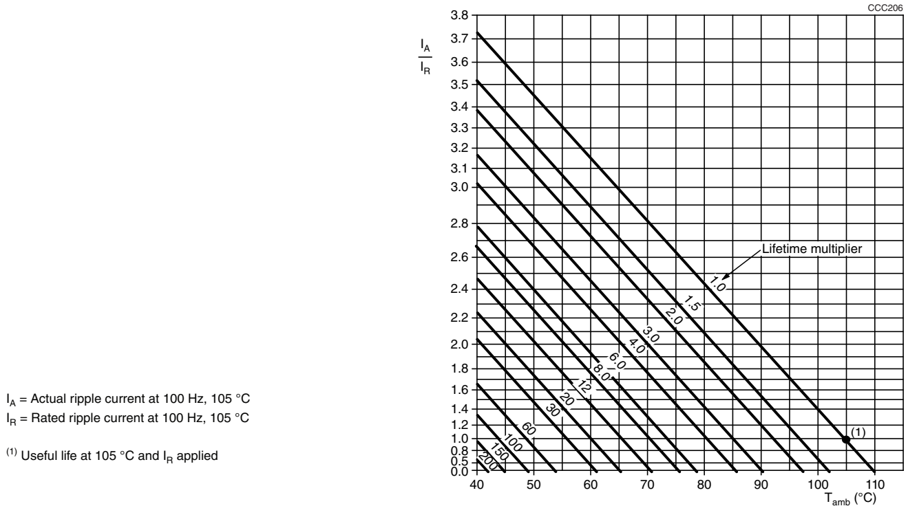
Fig. 8 - Multiplier of useful life as a function of ambient temperature and ripple current load
