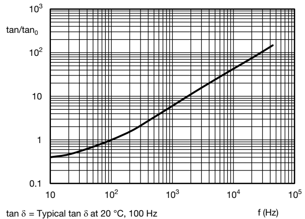
Fig. 10 - Typical multiplier of dissipation factor ( \tan \delta ) as a function of frequency
