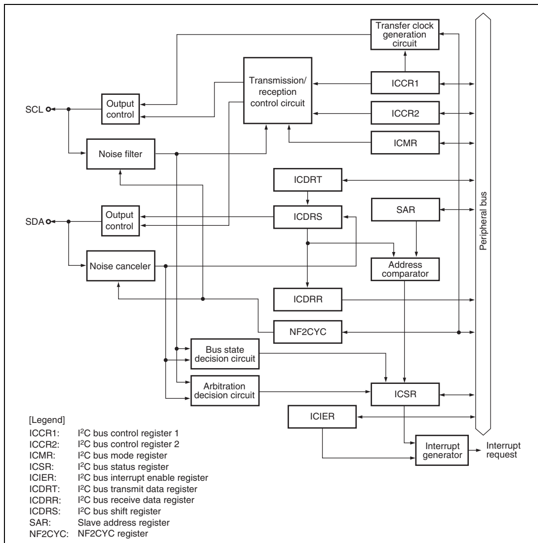
Figure 17.1 Block Diagram
