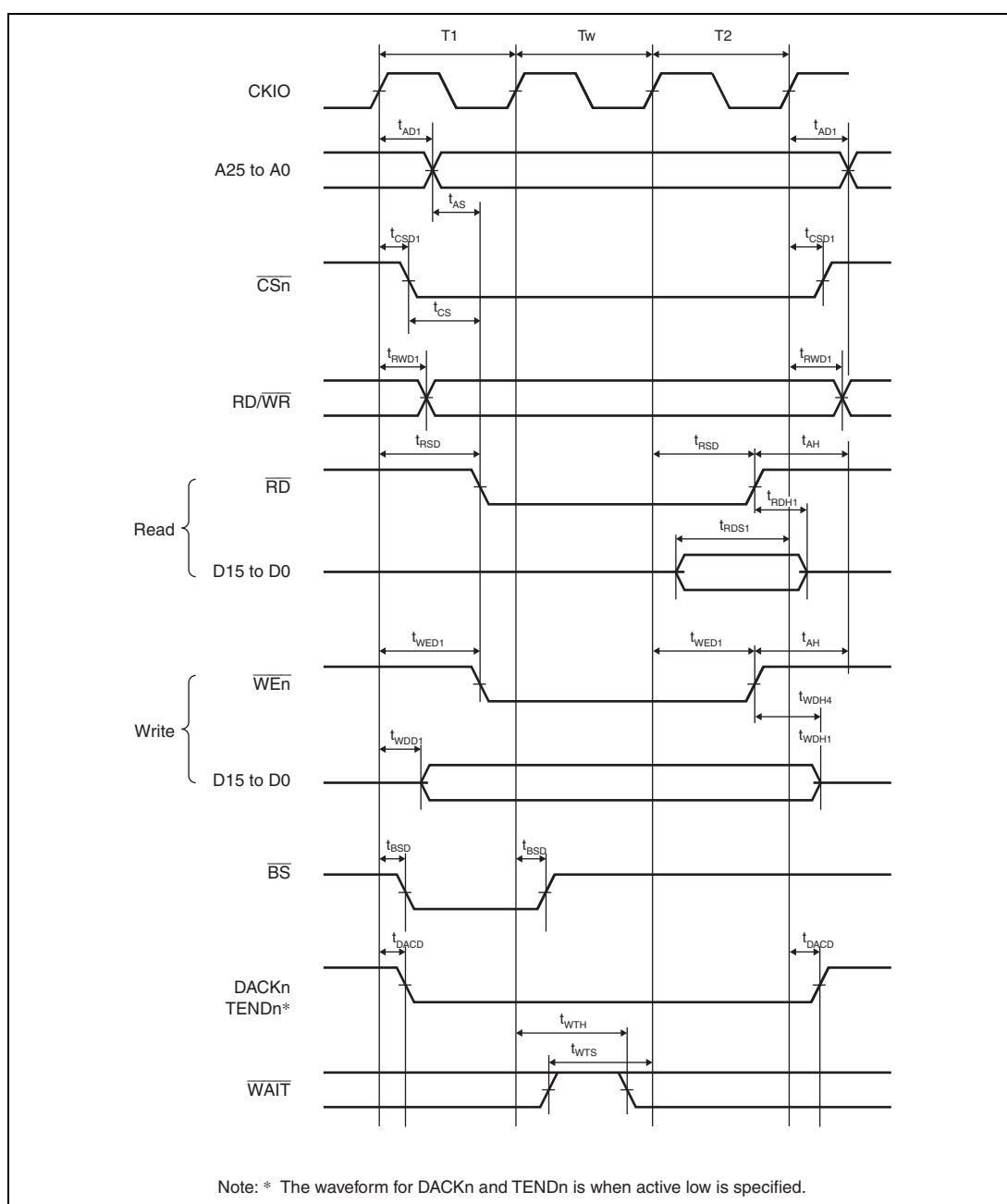
Figure 37.10 Basic Bus Timing for Normal Space (One Software Wait Cycle)
