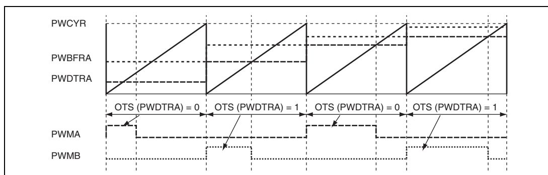
Figure 35.7 PWM Operation
