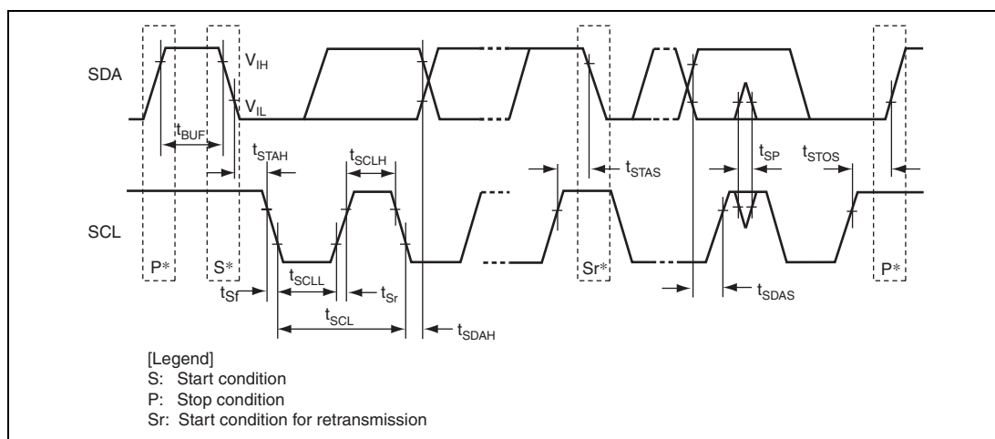
Figure 37.52 (1) Input/Output Timing
