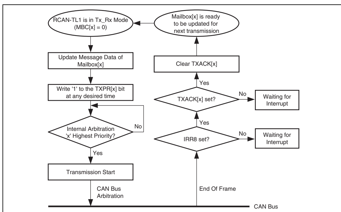
Figure 20.16 Transmission request
