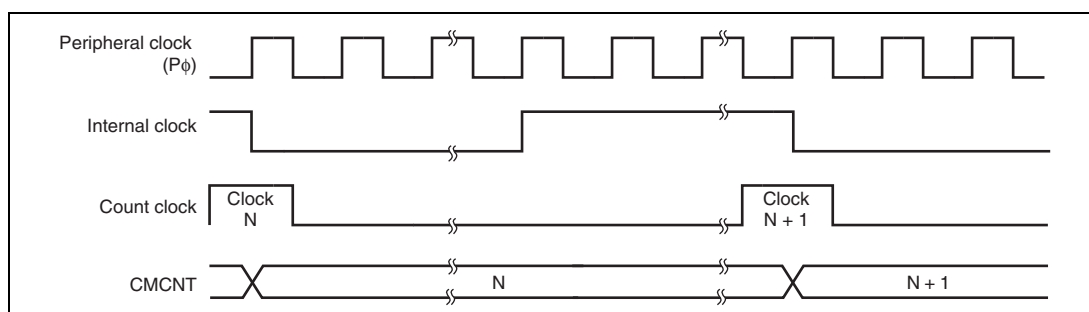
Figure 12.3 Count Timing
