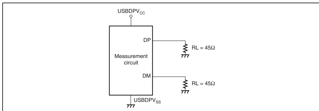
Figure 37.70 Measurement Circuit (High-Speed)
