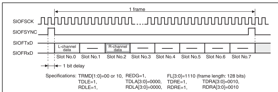
Figure 19.14 Transmit and Receive Timing (16-Bit Stereo Data (2))
