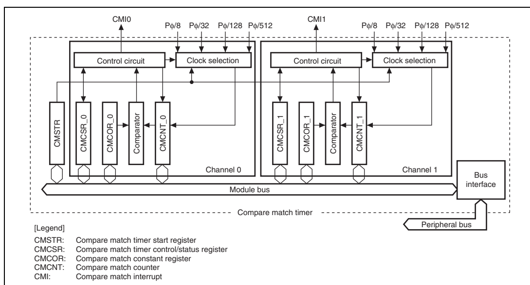
Figure 12.1 Block Diagram
