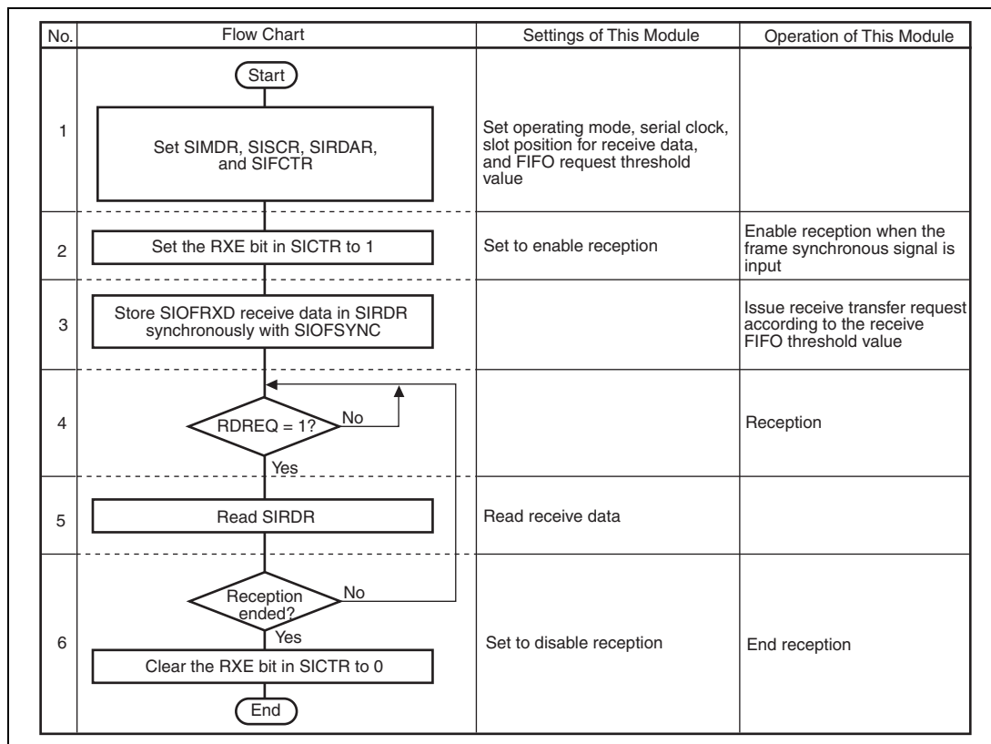
Figure 19.9 Example of Receive Operation in Slave Mode
