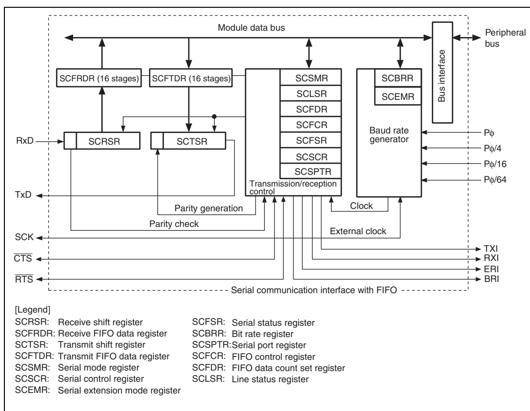
Figure 15.1 Block Diagram
