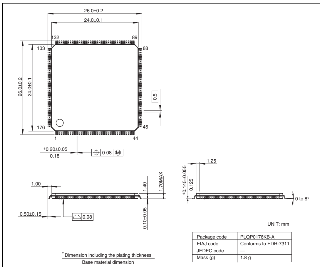
Figure A.1 Package Dimensions of the SH7262
