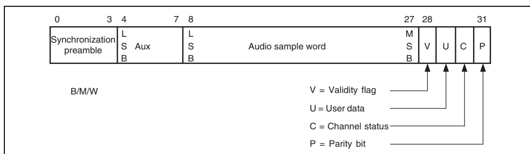
Figure 22.3 Subframe Format
