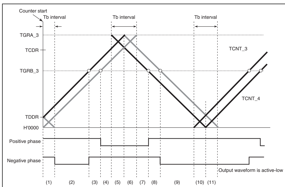
Figure 11.56 Timing for Synchronous Counter Clearing
