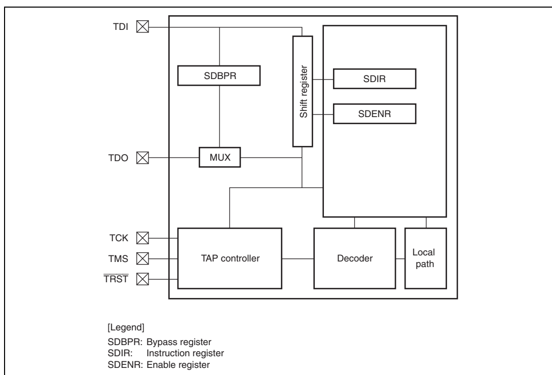
Figure 34.1 Block Diagram
