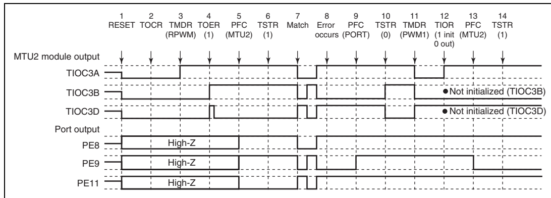
Figure 11.141 Error Occurrence in Reset-Synchronized PWM Mode, Recovery in PWM Mode 1
