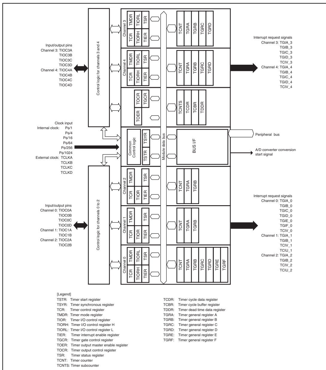
Figure 11.1 Block Diagram
