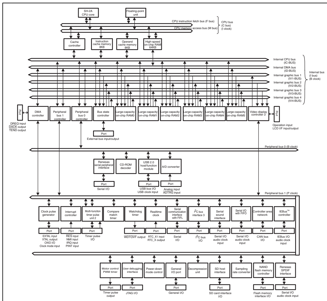
Figure 1.1 Block Diagram
