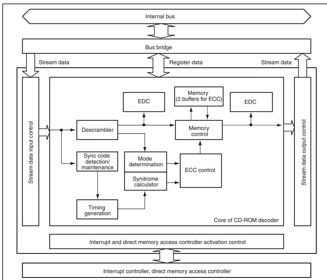
Figure 23.2 Block Diagram
