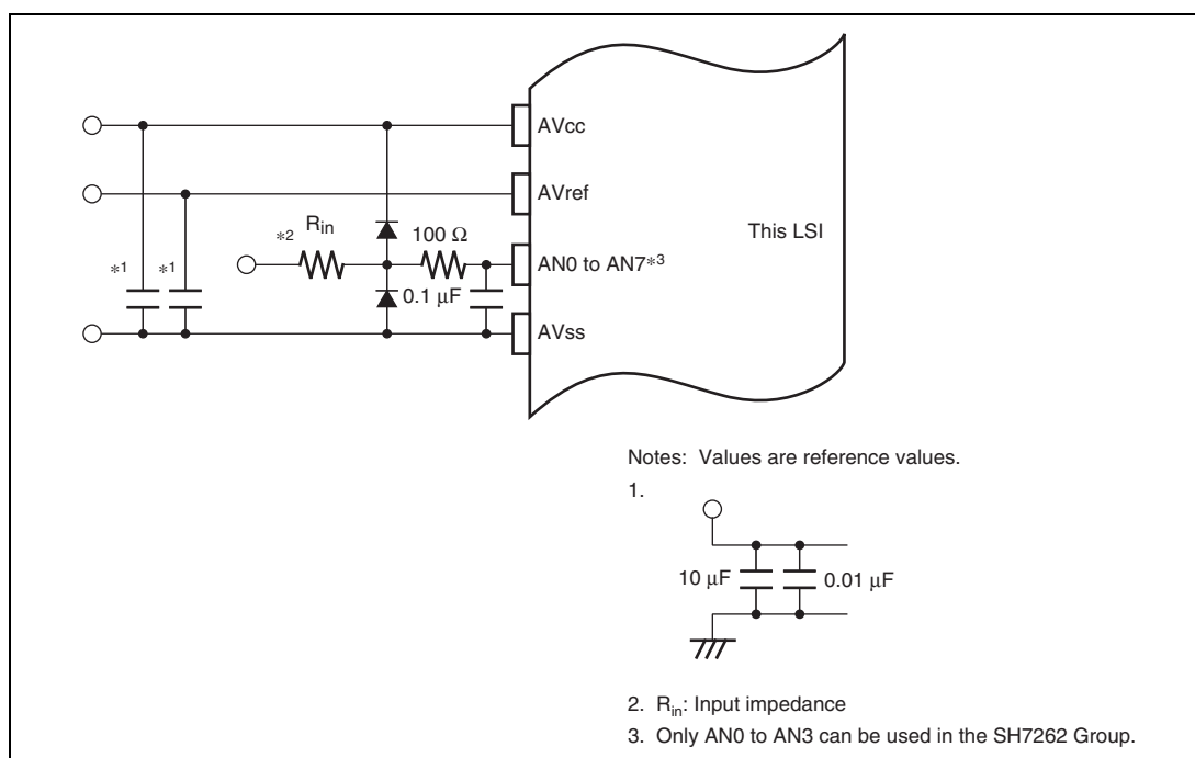
Figure 24.8 Example of Analog Input Protection Circuit
