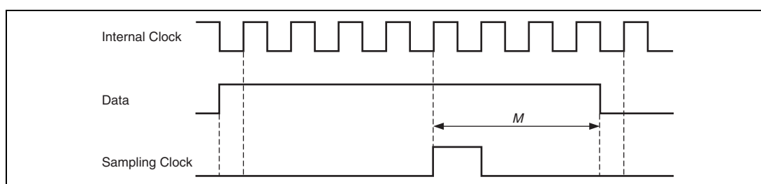
Figure 22.7 Receive Margin
