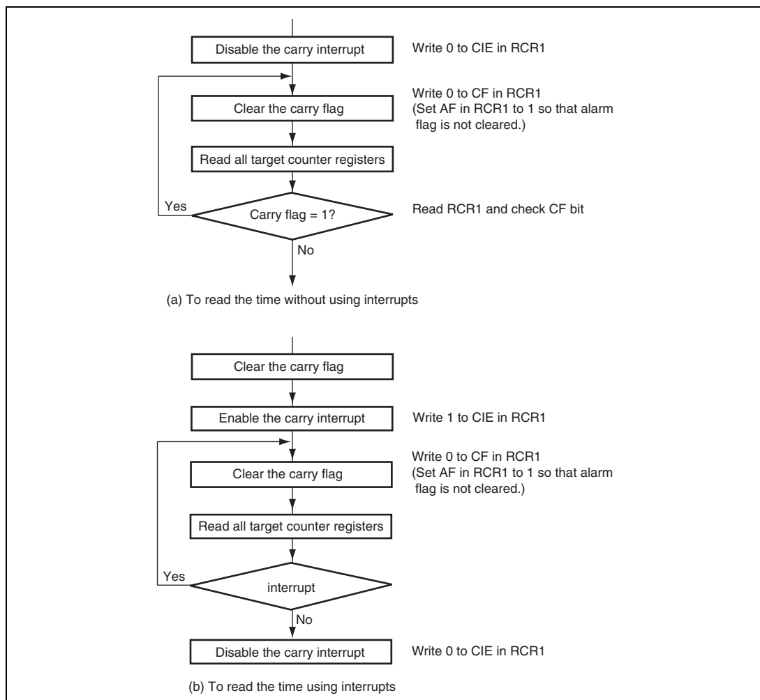
Figure 14.3 Reading Time
