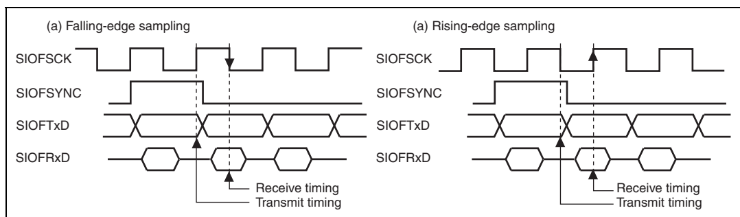
Figure 19.4 Transmit/Receive Timing
