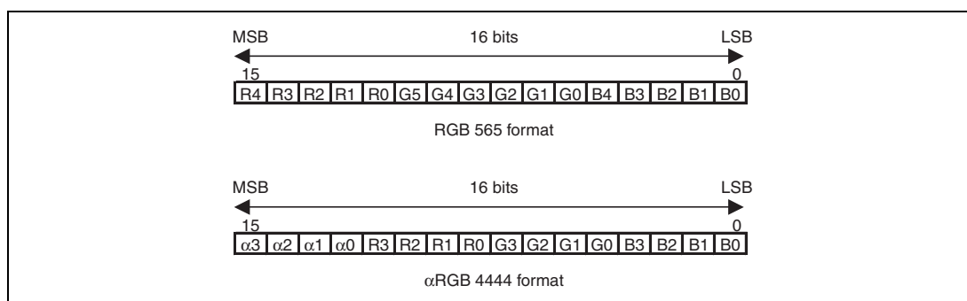
Figure 27.18 Bus Format
