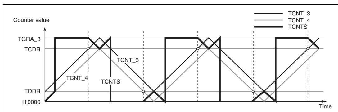
Figure 11.39 Complementary PWM Mode Counter Operation
