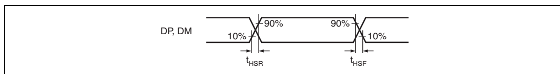
Figure 37.69 DP and DM Output Timing (High-Speed)
