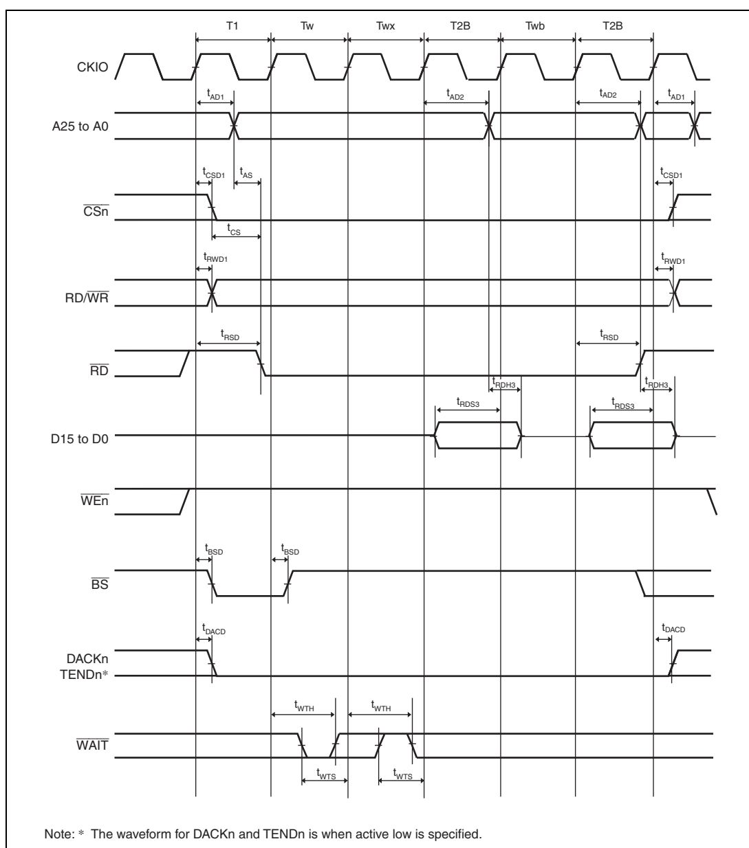
Figure 37.16 Burst ROM Read Cycle (One Software Wait Cycle, One Asynchronous External Burst Wait Cycle, Two Burst)
