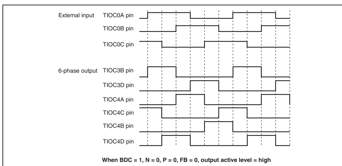
Figure 11.63 Example of Output Phase Switching by External Input (1)
