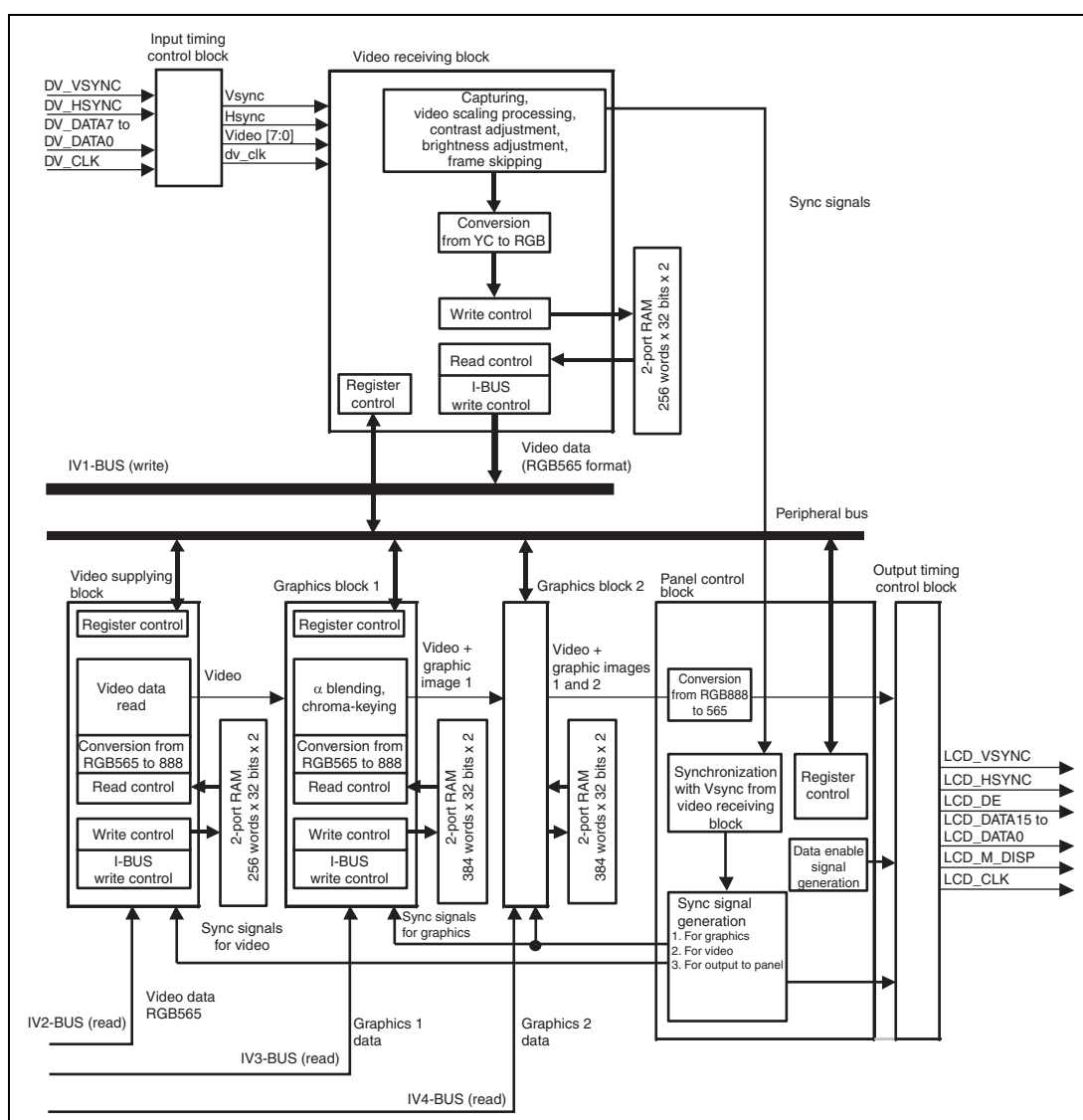
Figure 27.1 Block Diagram
