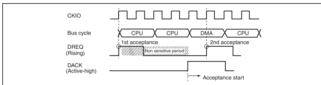
Figure 10.11 Example of DREQ Input Detection in Cycle Steal Mode Edge Detection
