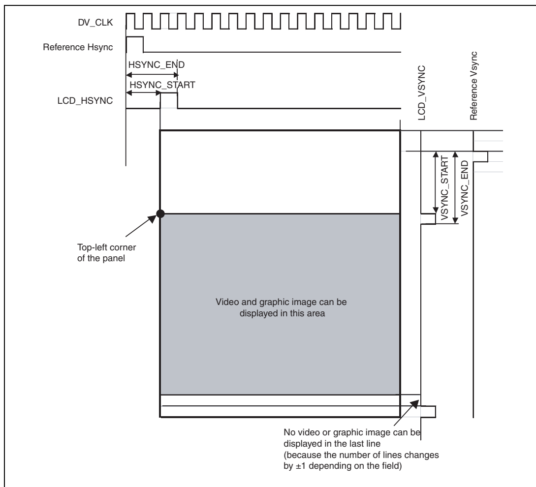
Figure 27.11 Example of Sync Signal Output
