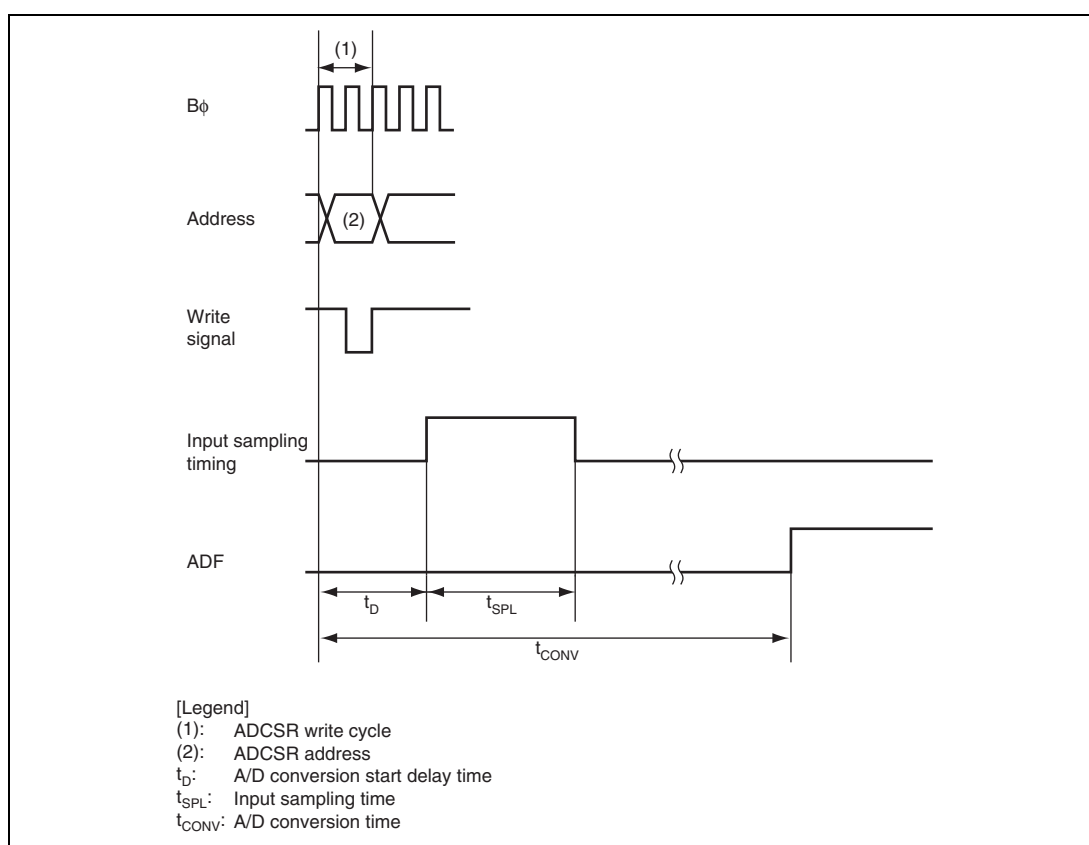
Figure 24.5 A/D Conversion Timing
