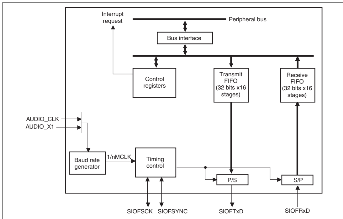
Figure 19.1 Block Diagram
