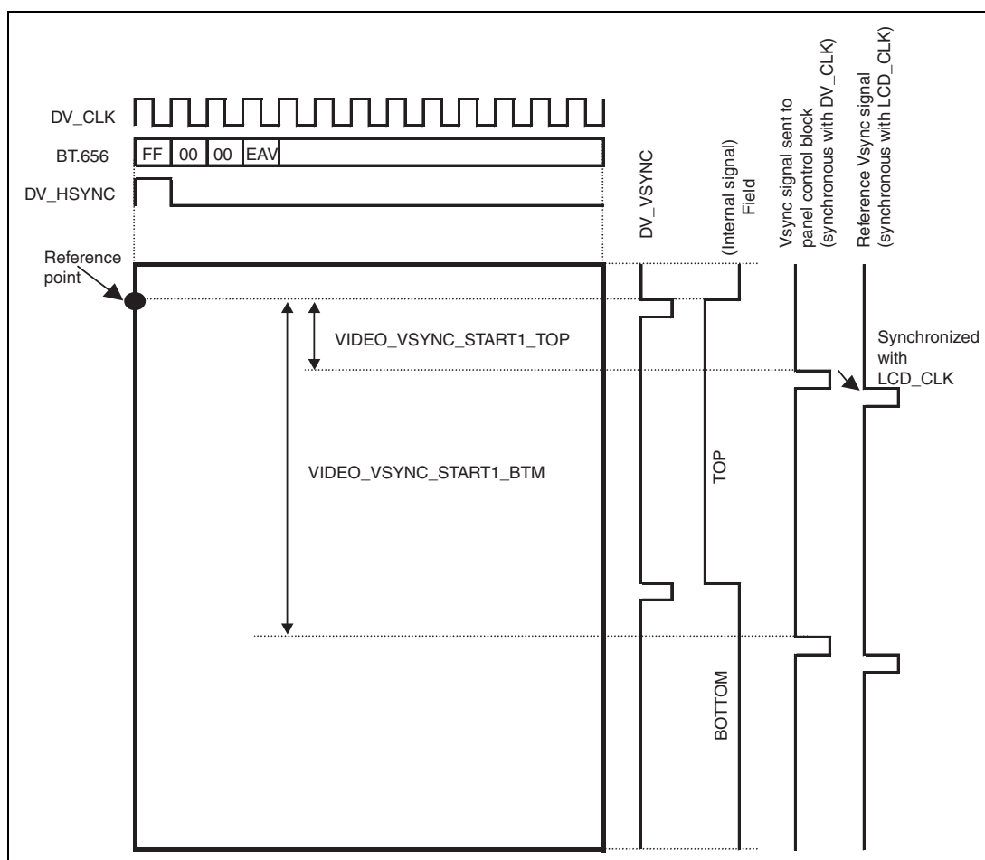
Figure 27.7 Timing of Reference Vsync Generation
