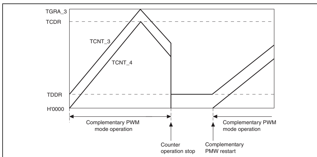
Figure 11.108 Counter Value during Complementary PWM Mode Stop
