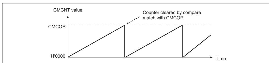
Figure 12.2 Counter Operation
