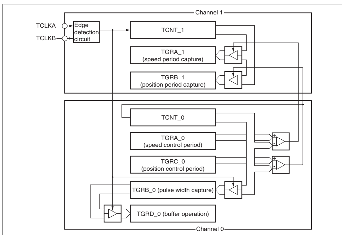
Figure 11.34 Phase Counting Mode Application Example
