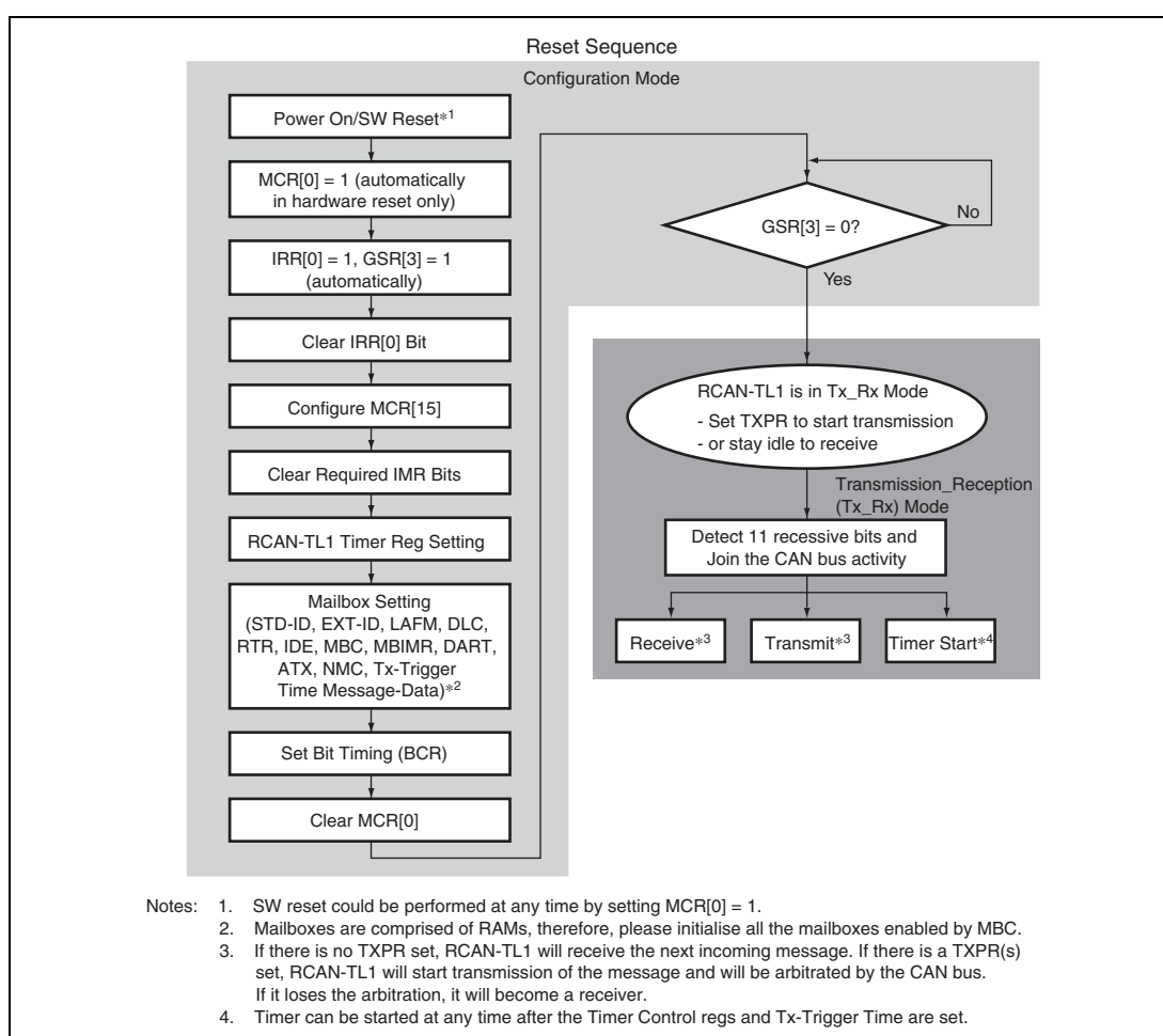
Figure 20.14 Reset Sequence
