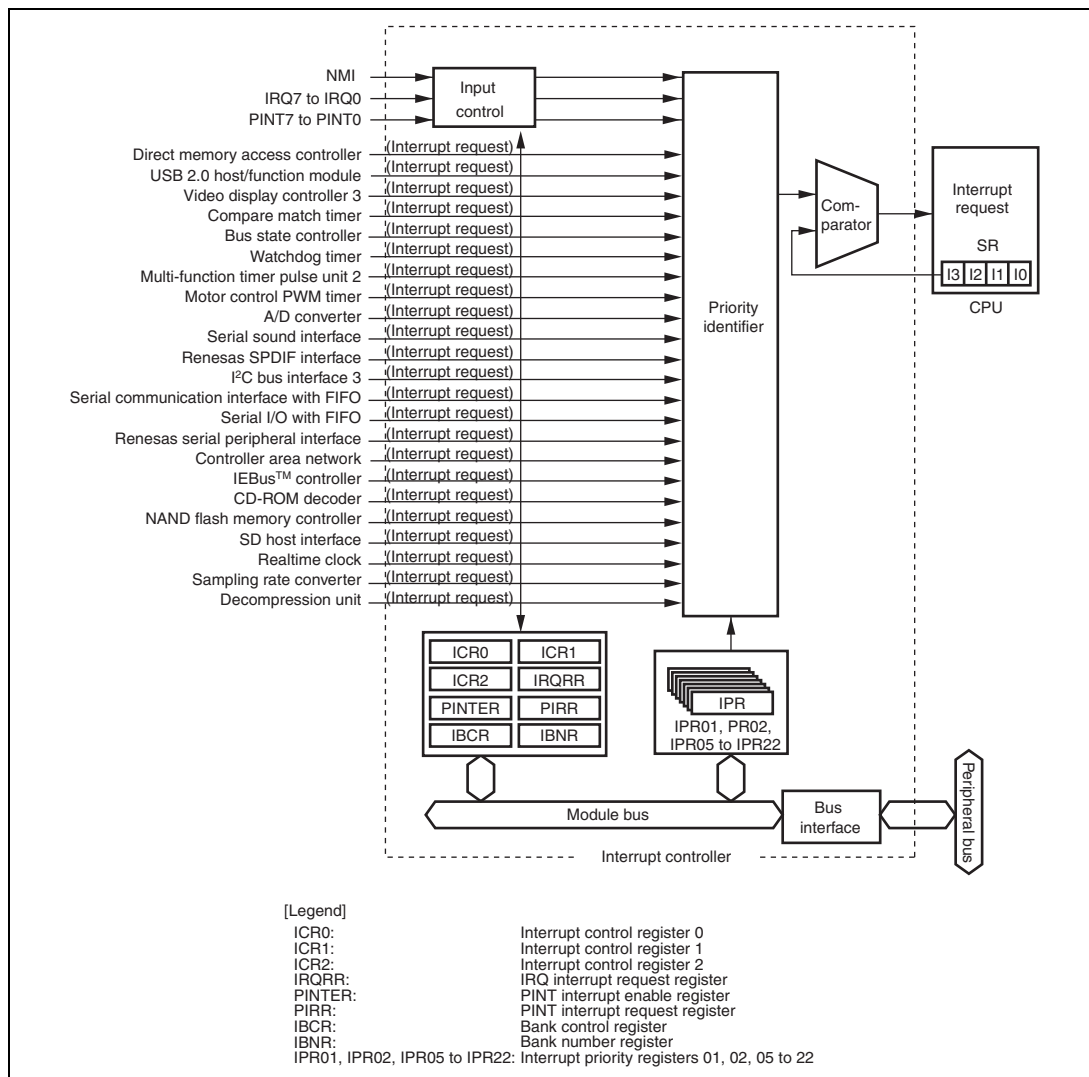
Figure 7.1 Block Diagram
