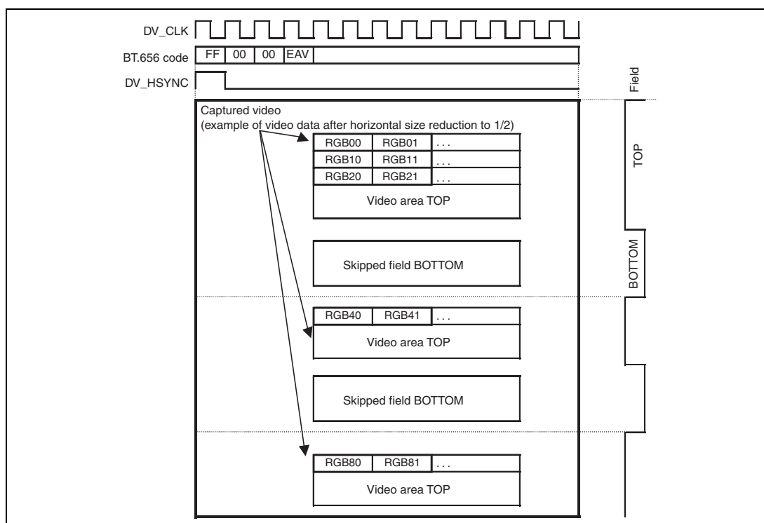
Figure 27.9 Correspondence between Video Data and Addresses
