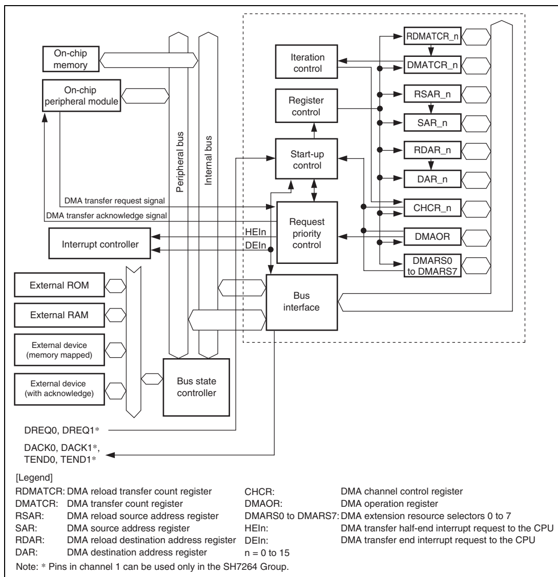
Figure 10.1 Block Diagram
