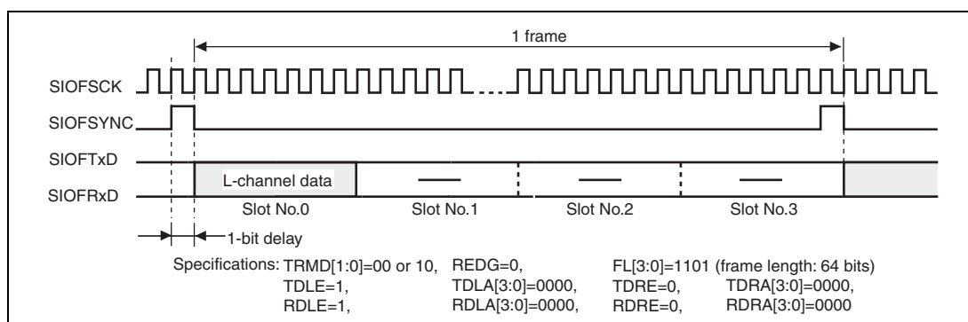
Figure 19.12 Transmit and Receive Timing (16-Bit Monaural Data)
