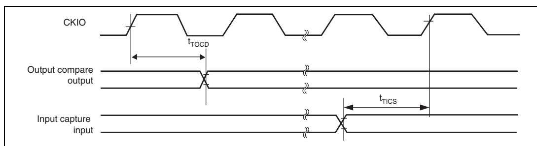
Figure 37.42 Pulse Input/Output Timing
