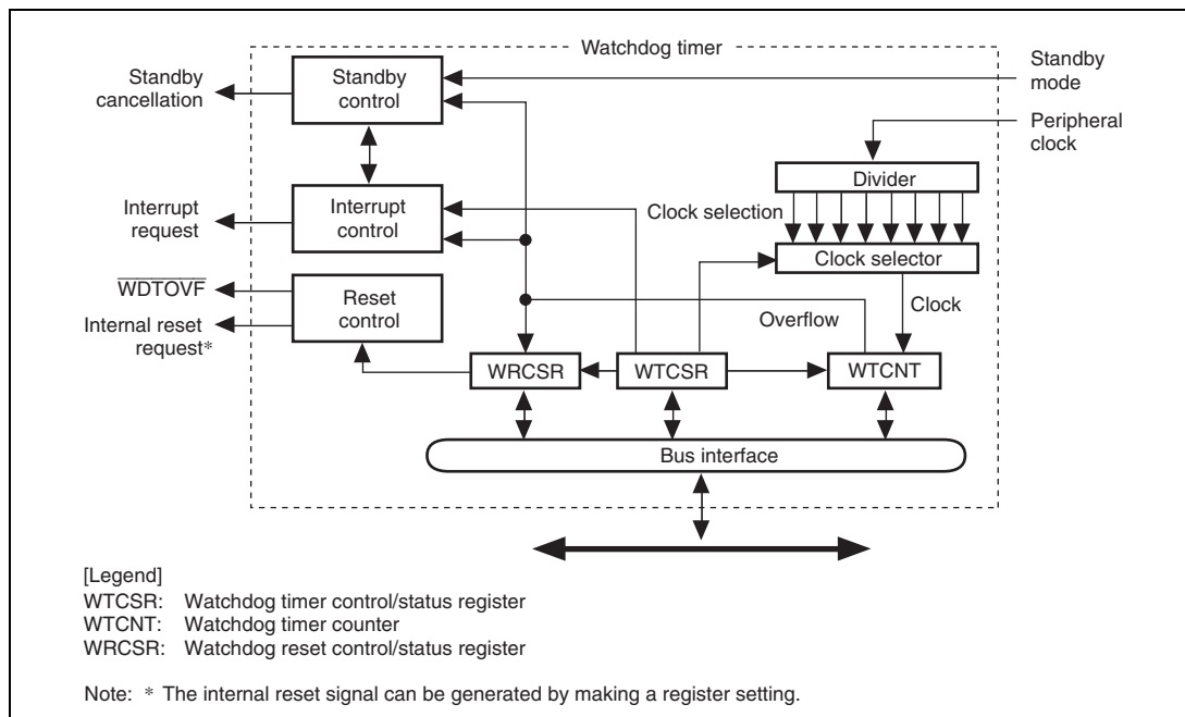
Figure 13.1 Block Diagram
