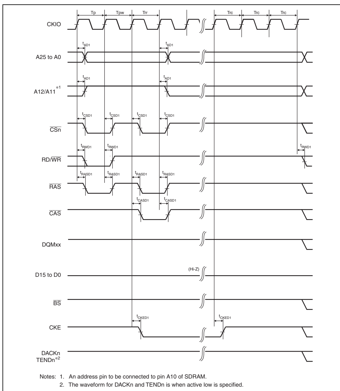
Figure 37.32 Synchronous DRAM Self-Refreshing Timing (WTRP = 1 Cycle)
