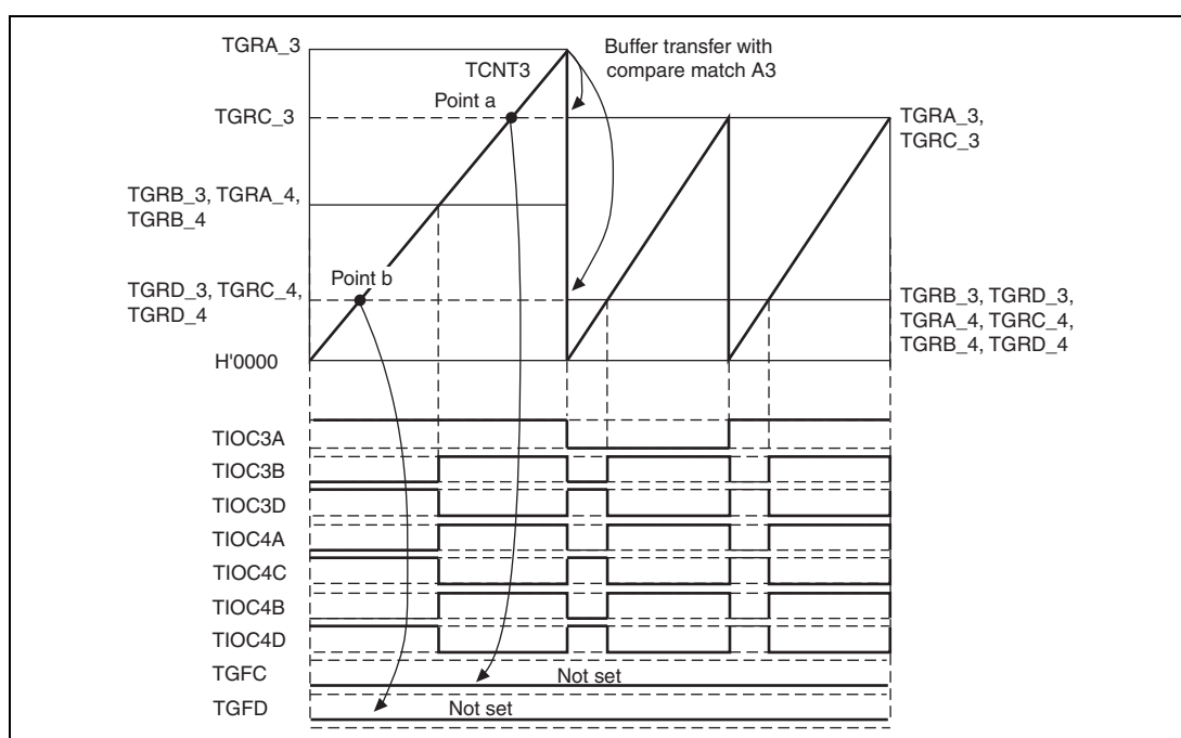
Figure 11.109 Buffer Operation and Compare-Match Flags in Reset Synchronous PWM Mode
