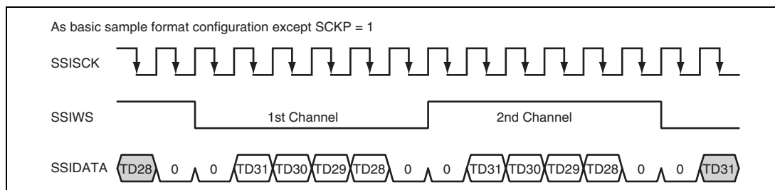
Figure 18.11 Inverted Clock
