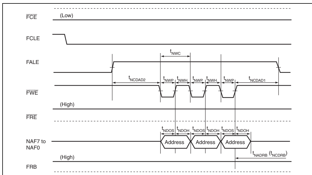
Figure 37.61 NAND Type Flash Memory Address Issuance Timing
