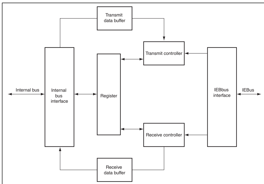
Figure 21.5 Block Diagram
