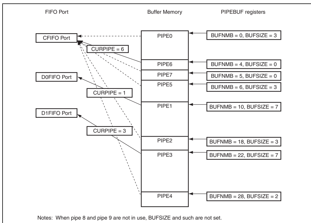
Figure 26.9 Example of a Buffer Memory Map
