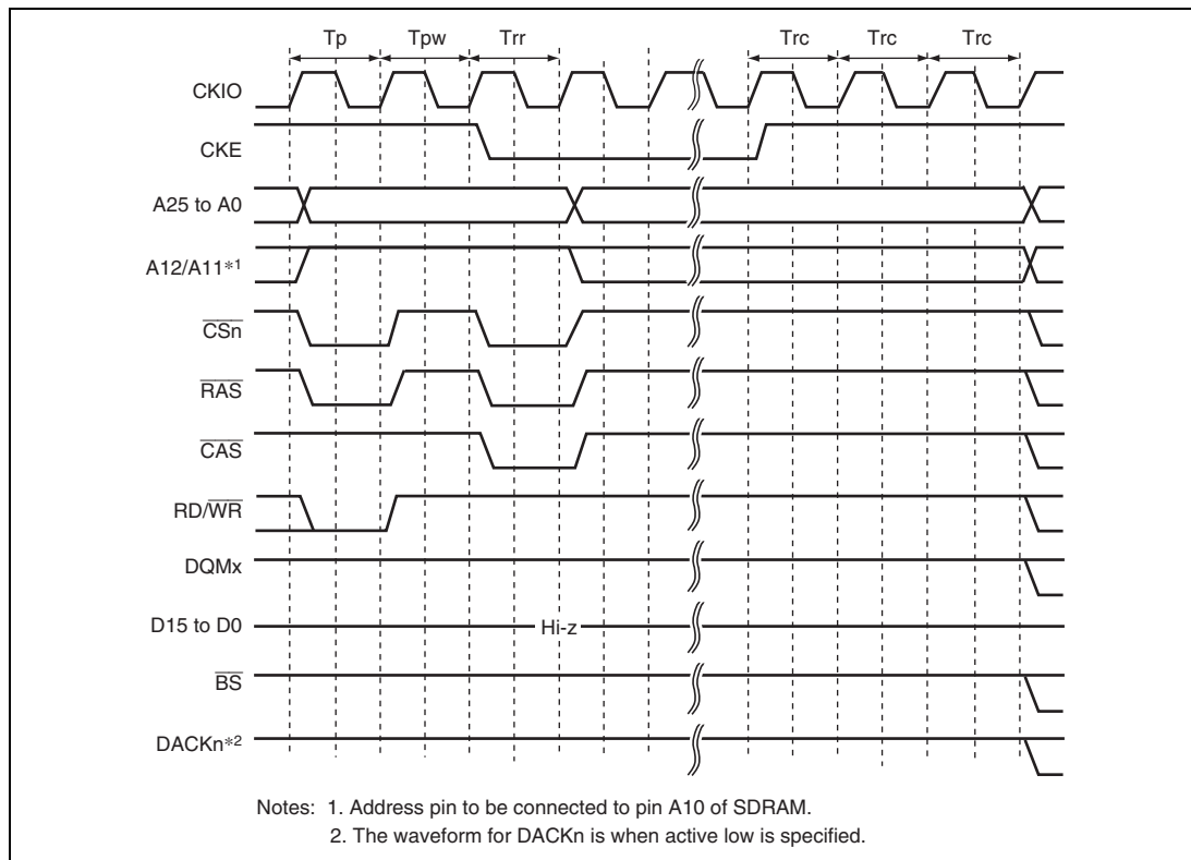
Figure 9.27 Self-Refresh Timing
