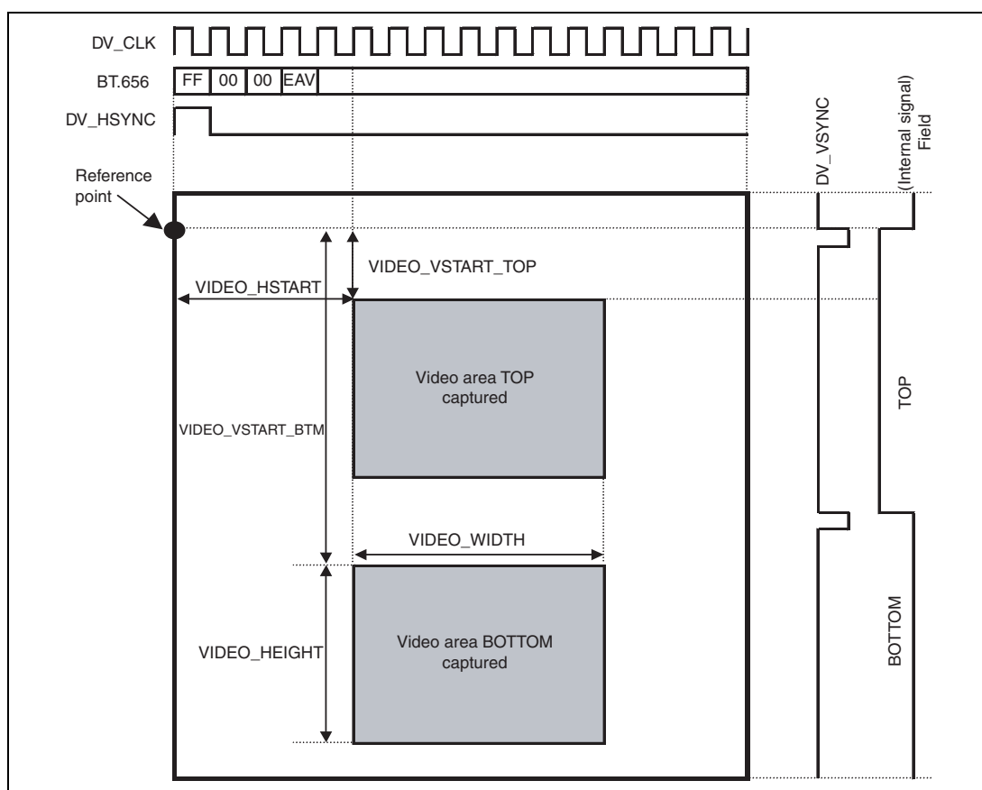
Figure 27.5 Concept of Capturing Function
