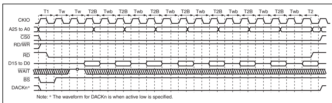
Figure 9.44 Burst ROM Access Timing (Clocked Synchronous) (Burst Length = 8, Wait Cycles Inserted in First Access = 2, Wait Cycles Inserted in Second and Subsequent Access Cycles = 1)
