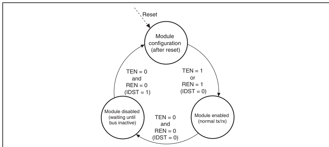
Figure 18.19 Operation Modes
