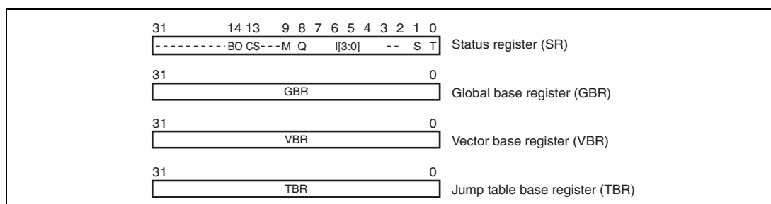
Figure 2.2 Control Registers
