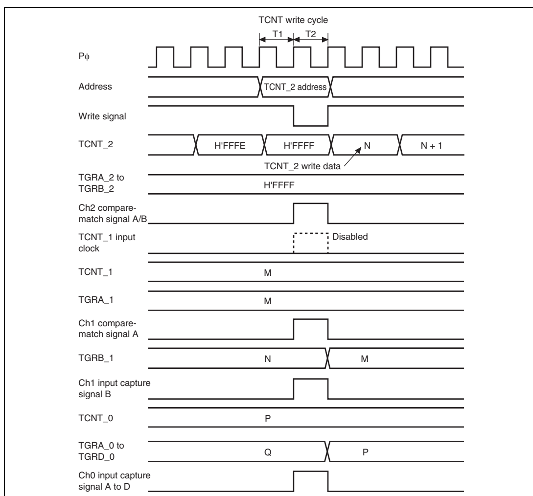
Figure 11.107 TCNT_2 Write and Overflow/Underflow Contention with Cascade Connection
