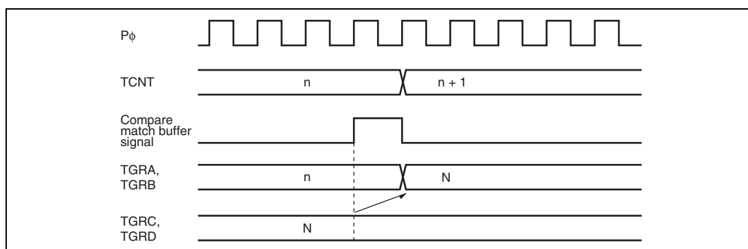
Figure 11.86 Buffer Operation Timing (Compare Match)
