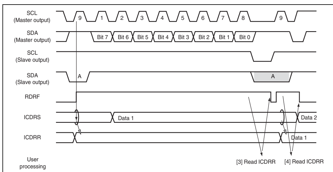
Figure 17.12 Slave Receive Mode Operation Timing (2)
