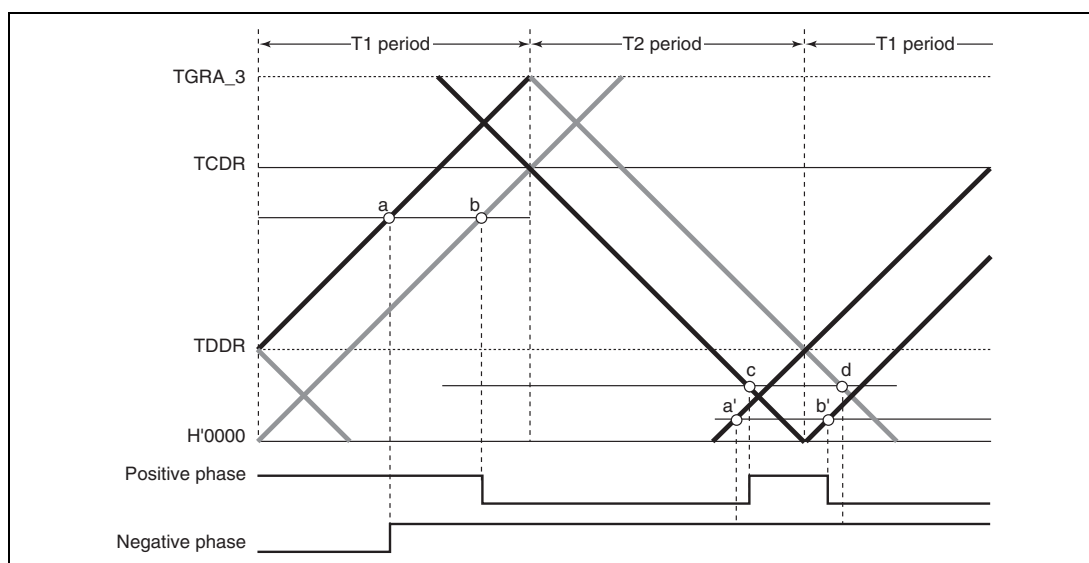
Figure 11.48 Example of Complementary PWM Mode Waveform Output (3)
