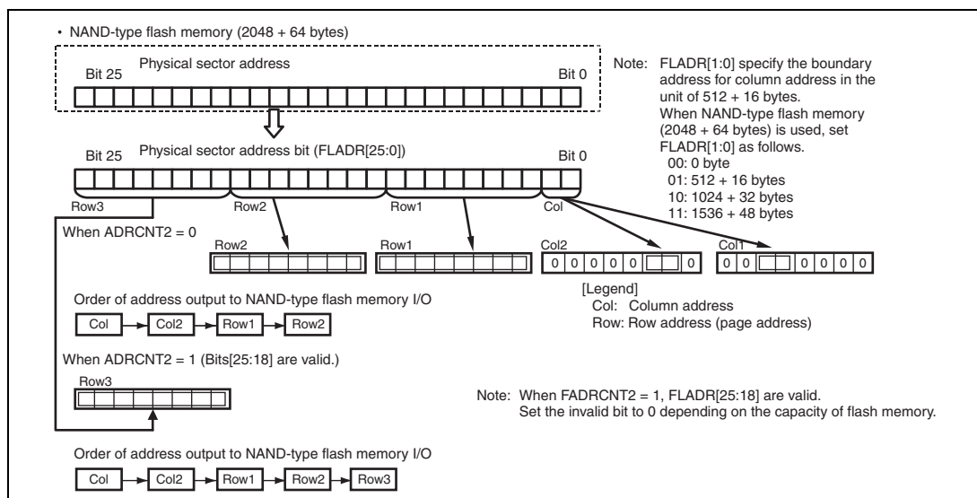
Figure 25.11 Relationship between Sector Number and Address Expansion of NAND-Type Flash Memory
