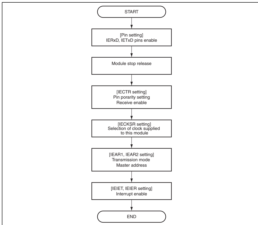
Figure 21.8 Flowchart for Initial Setting
