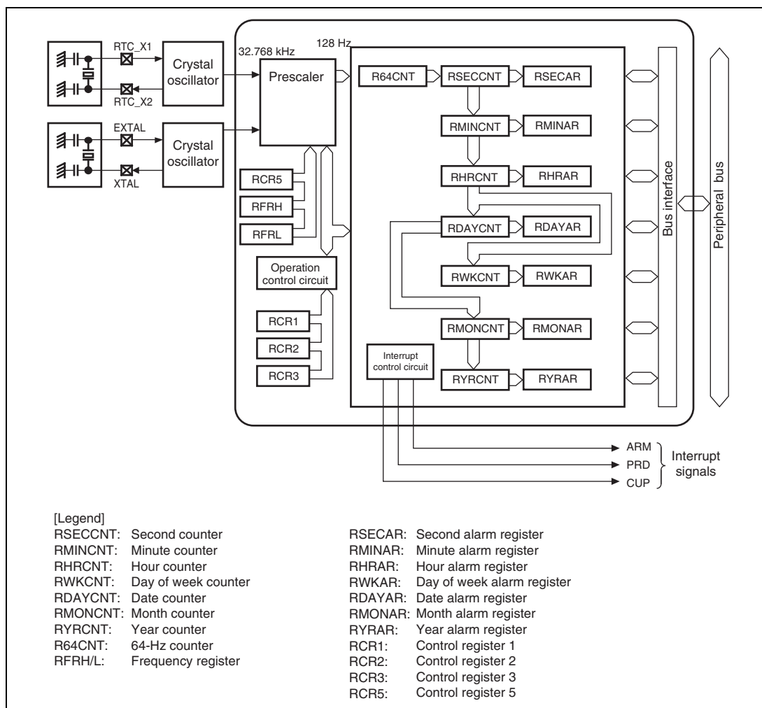
Figure 14.1 Block Diagram
