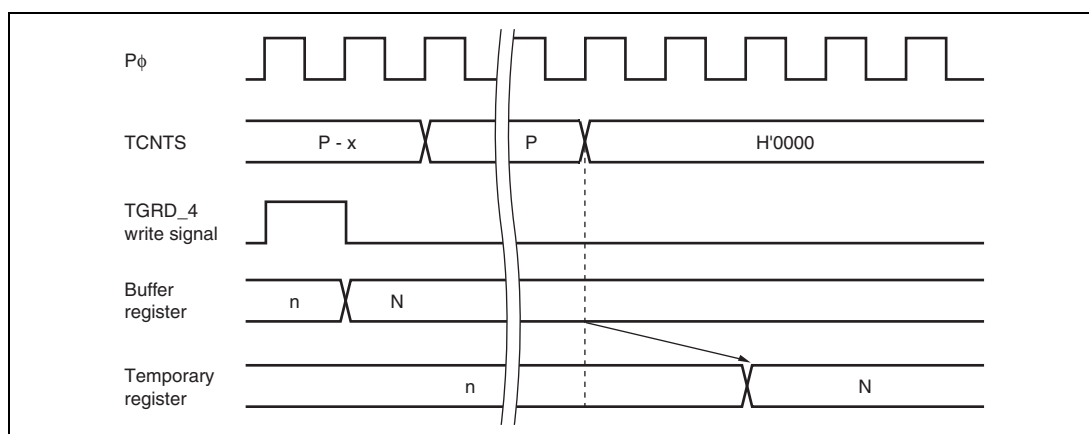
Figure 11.90 Transfer Timing from Buffer Register to Temporary Register (TCNTS Operating)
