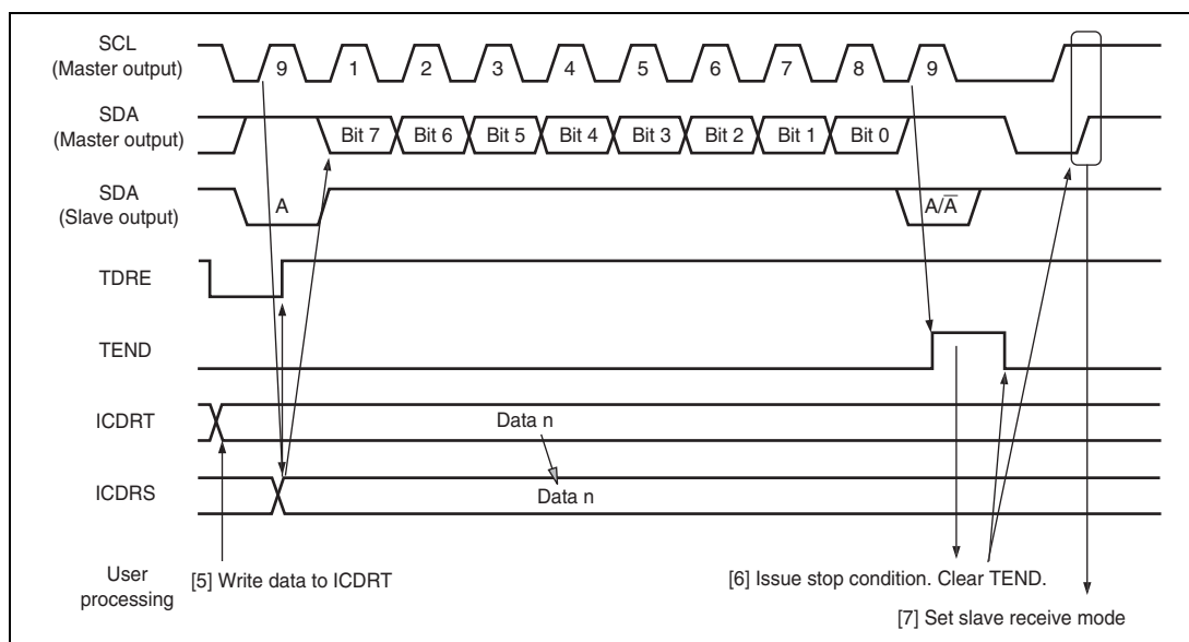
Figure 17.6 Master Transmit Mode Operation Timing (2)
