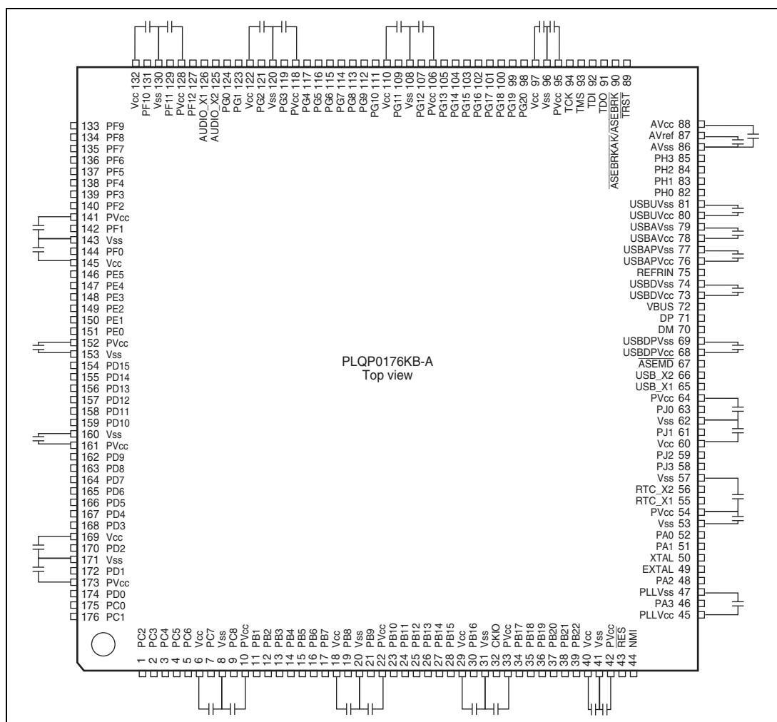
Figure 38.1 Example of Externally Allocated Capacitors in the SH7262 Group
