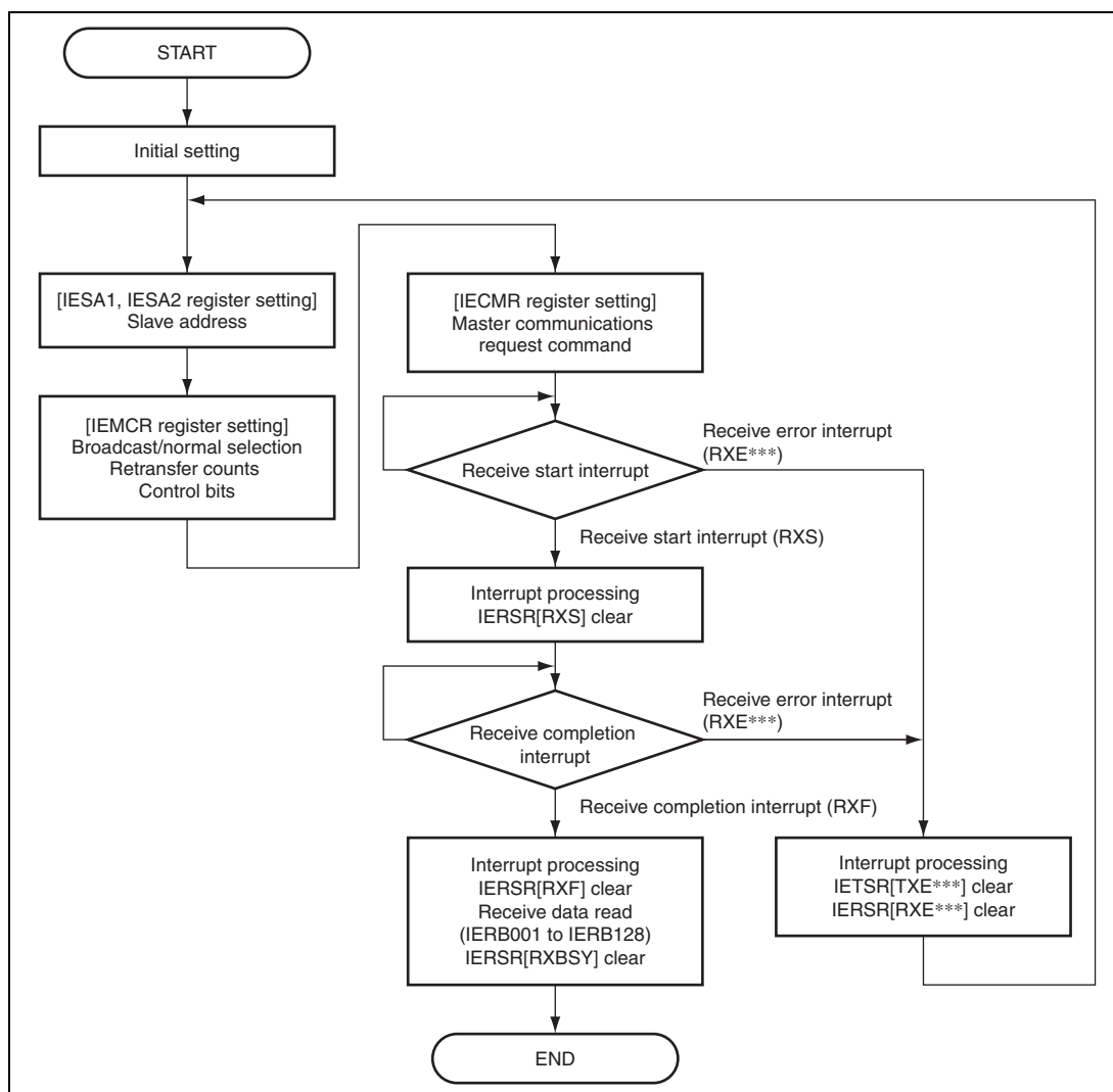
Figure 21.11 Flowchart for Master Reception
