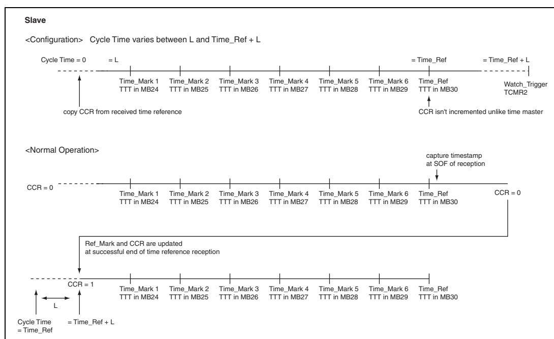
Figure 20.20 Time Slave
