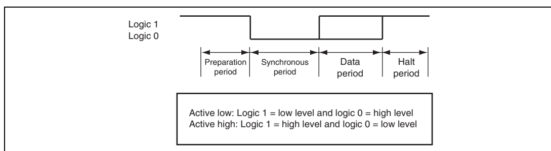
Figure 21.4 IEBus Bit Format (Conceptual Diagram)
