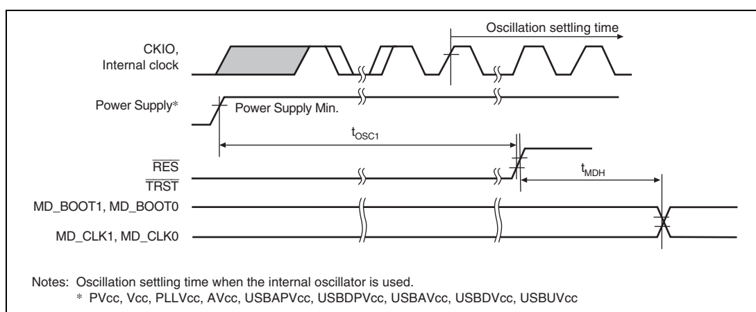
Figure 37.3 Power-On Oscillation Settling Time
