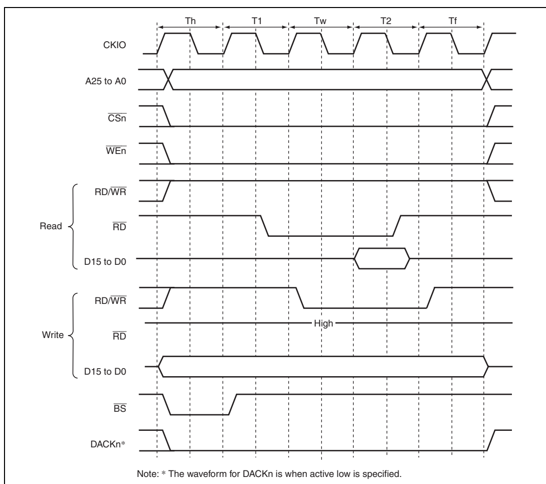
Figure 9.36 Wait Timing for SRAM with Byte Selection (BAS = 1) (SW[1:0] = 01, WR[3:0] = 0001, HW[1:0] = 01)
