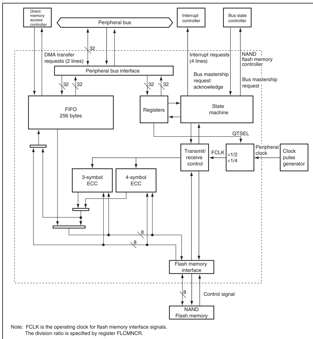
Figure 25.1 Block Diagram
