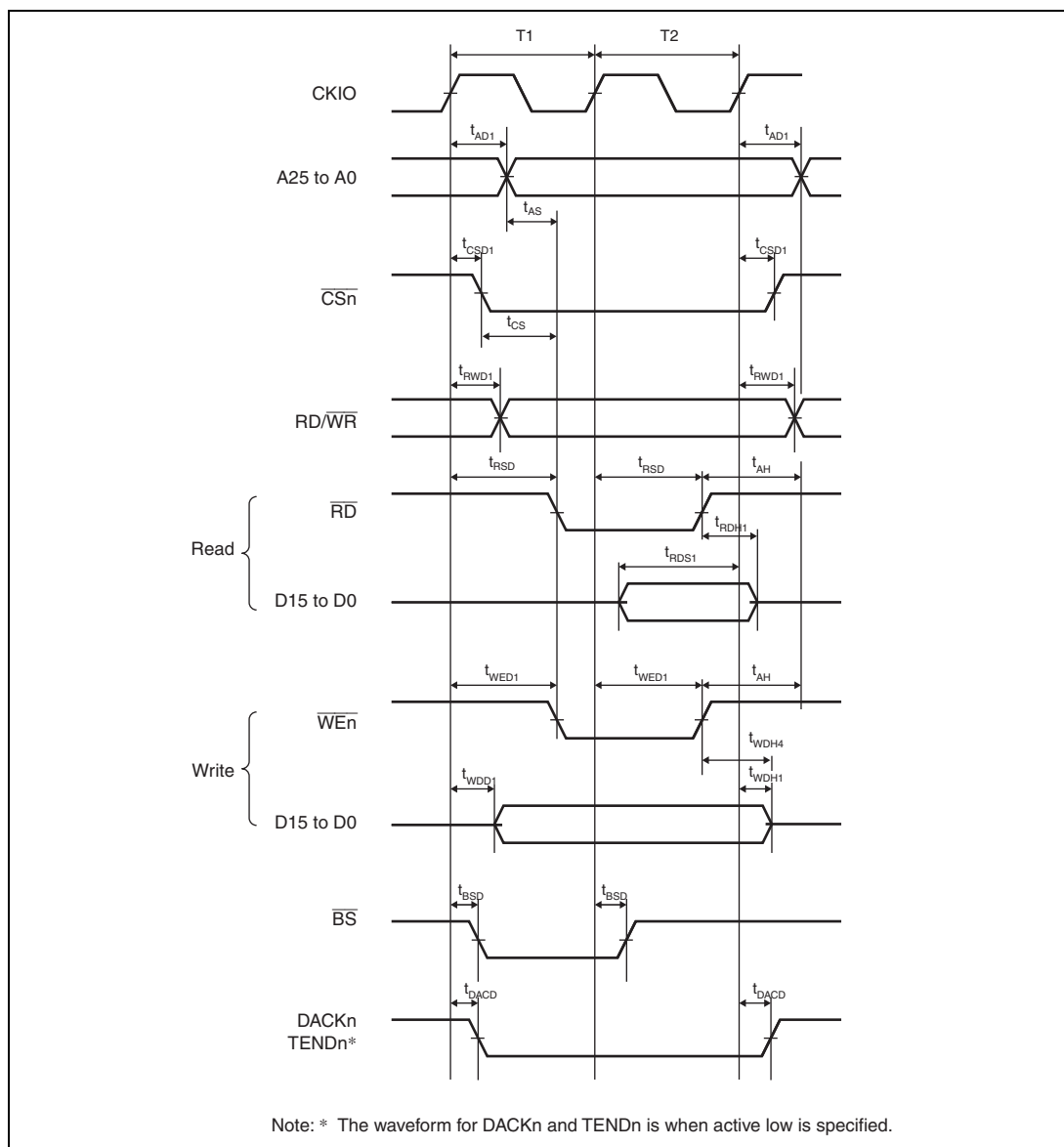
Figure 37.9 Basic Bus Timing for Normal Space (No Wait)
