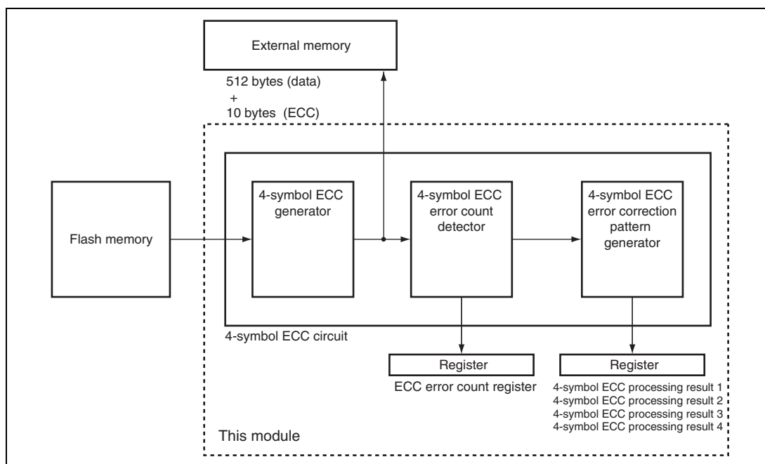
Figure 25.15 4-Symbol ECC Circuit
