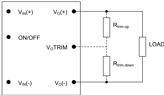
Figure 62. Circuit Configuration to Trim Output Voltage.
