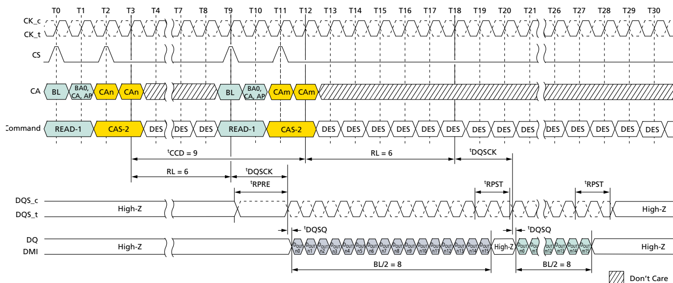
Figure 45: Consecutive READ: t_{CCD} = \text{MIN} + 1 , Preamble = Static, 1.5n\text{CK} Postamble
