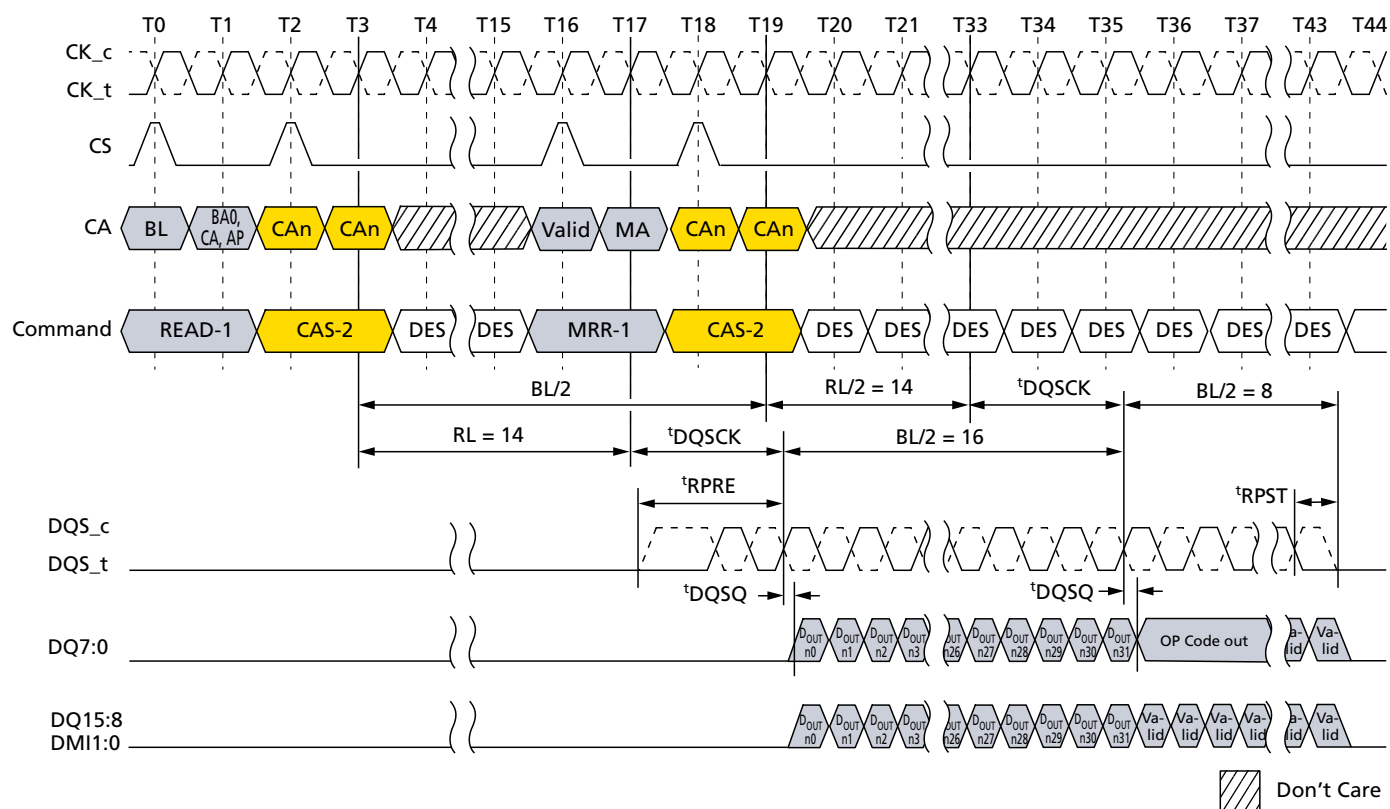
Figure 95: READ-to-MRR Timing
