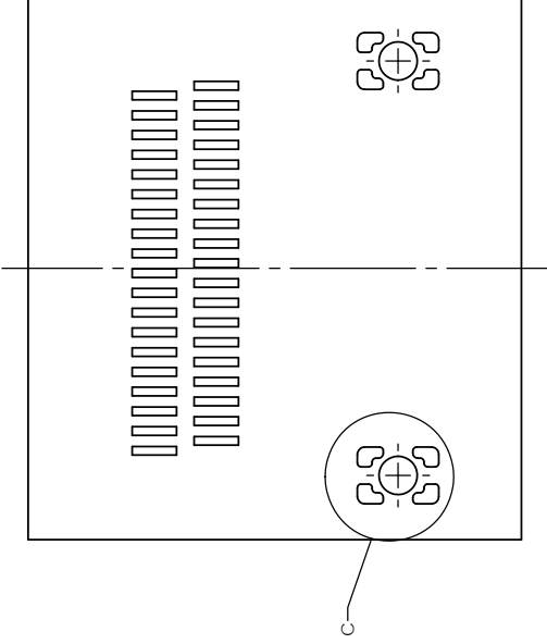
RECOMMENDED SOLDER MASK LAYOUT FOR 1X1
