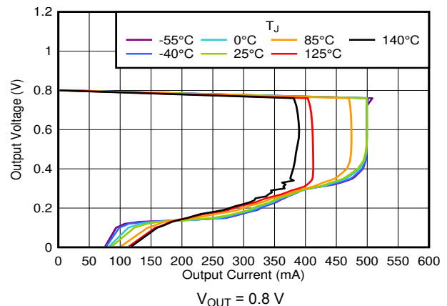
Figure 6-36. Foldback Current Limit vs I_{OUT} and Temperature
