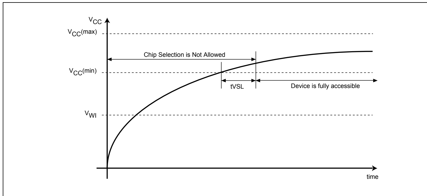
Figure 109. Power-up Timing
