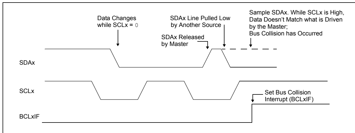
FIGURE 21-27: BUS COLLISION TIMING FOR TRANSMIT AND ACKNOWLEDGE
