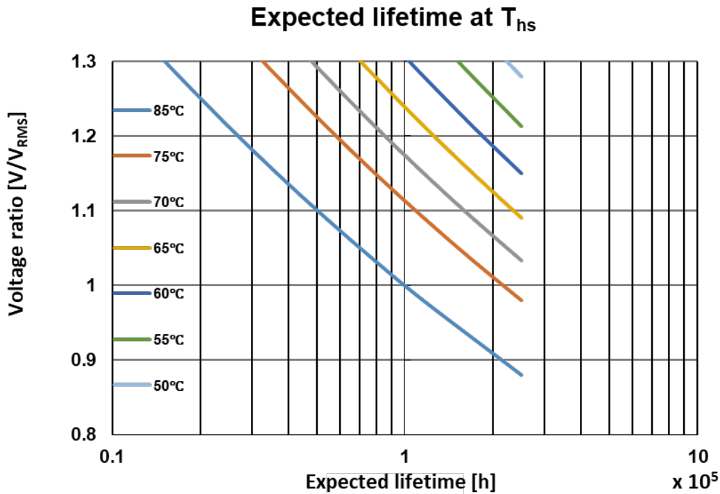
Figure 15: Expected lifetime in hours at different hot-spot temperatures (T hs ) and voltages V RMS .
