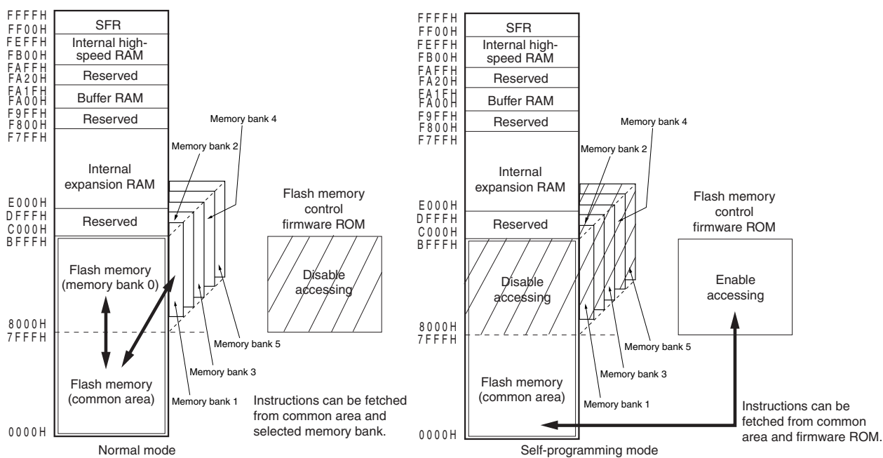
Figure 27-13. Operation Mode and Memory Map for Self-Programming ( \mu PD78F0547 and 78F0547A)
