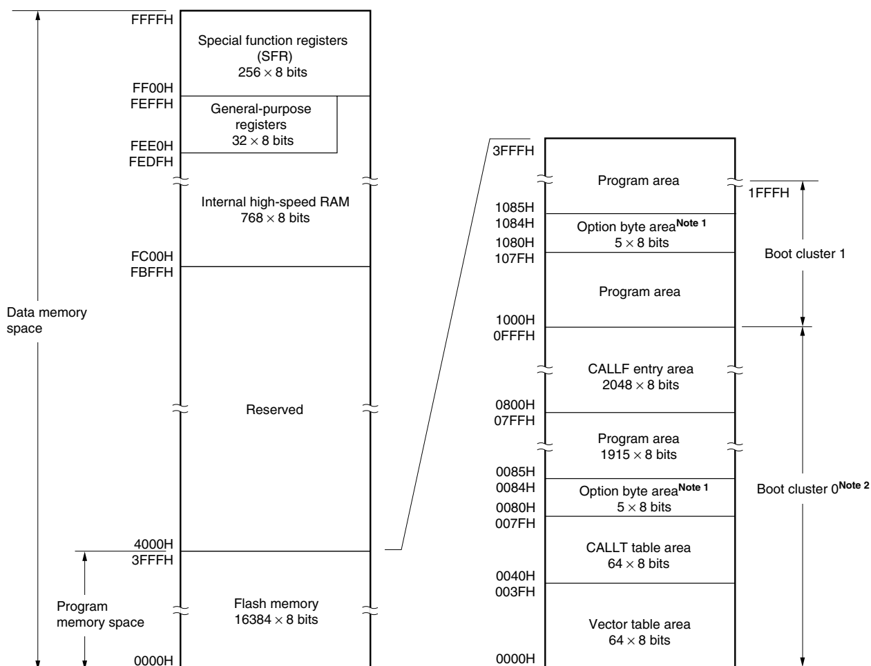
Figure 3-2. Memory Map ( \mu PD78F0501, 78F0501A, 78F0511, 78F0511A, 78F0521, 78F0521A, 78F0531, and 78F0531A)
