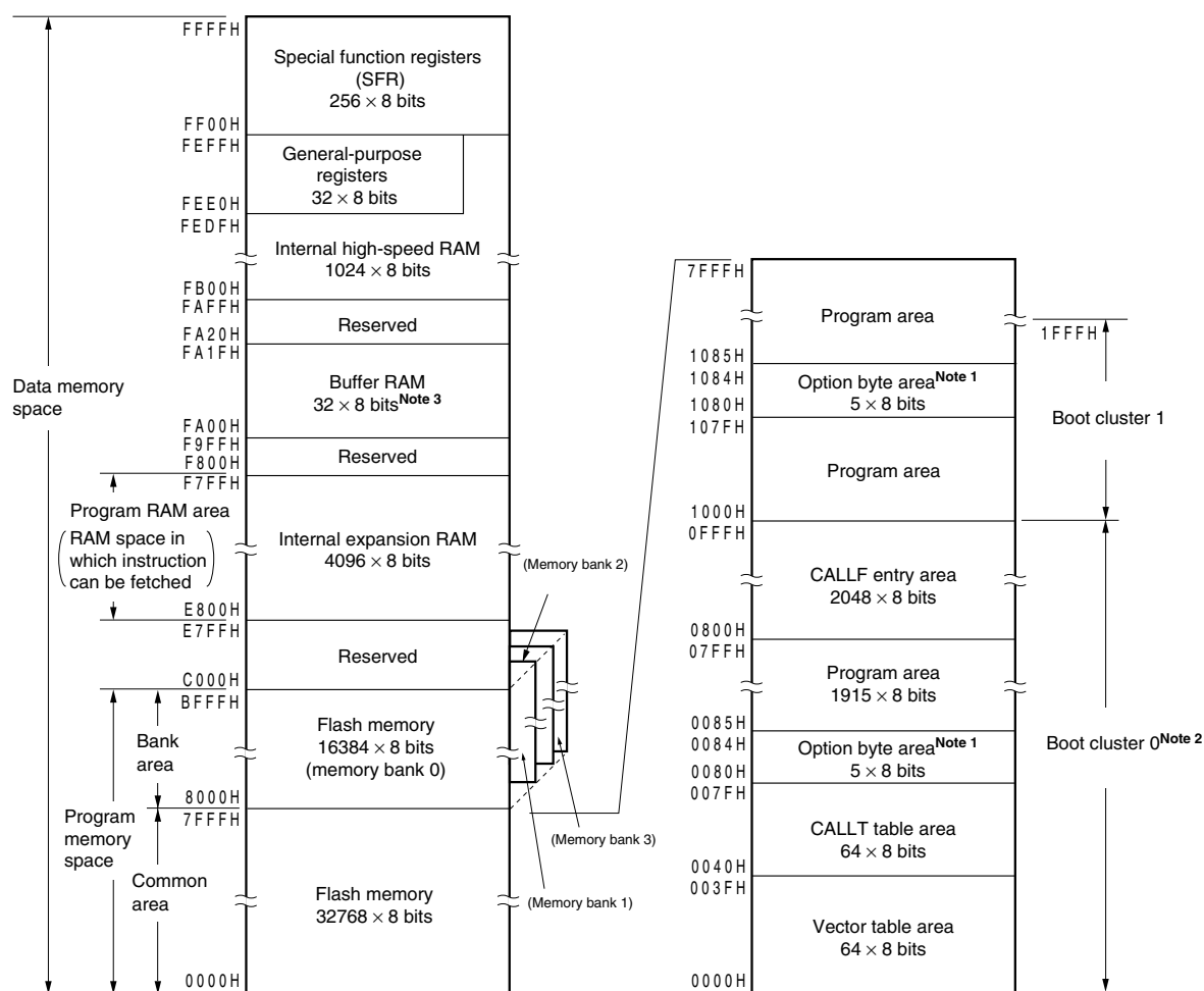
Figure 3-9. Memory Map ( \mu PD78F0526, 78F0526A, 78F0536, 78F0536A, 78F0546, and 78F0546A)
