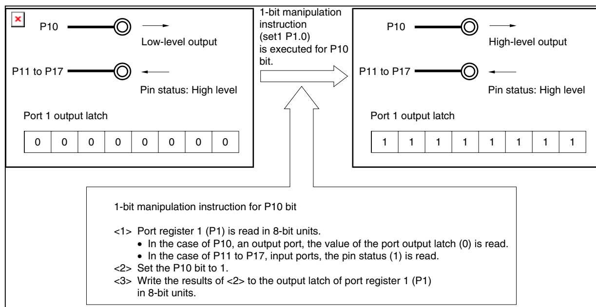
Figure 5-45. Bit Manipulation Instruction (P10)
