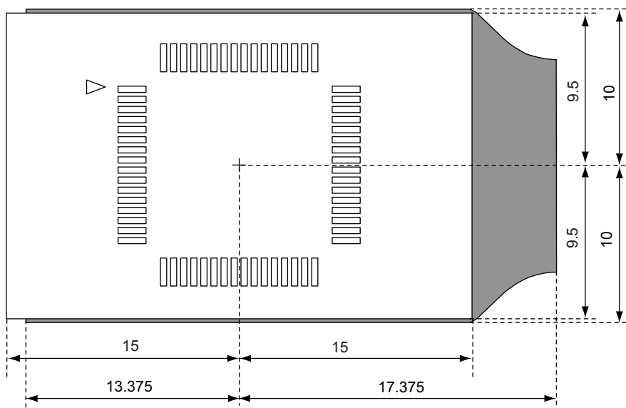
Figure B-7. For 64-Pin GA Package
