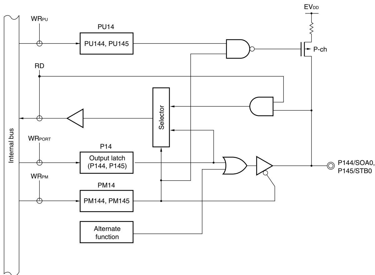
Figure 5-28. Block Diagram of P144 and P145
