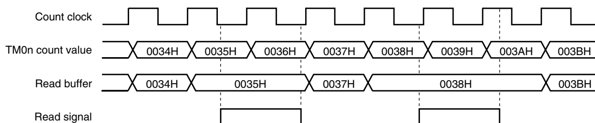
Figure 7-63. 16-bit Timer Counter 0n (TM0n) Read Timing
