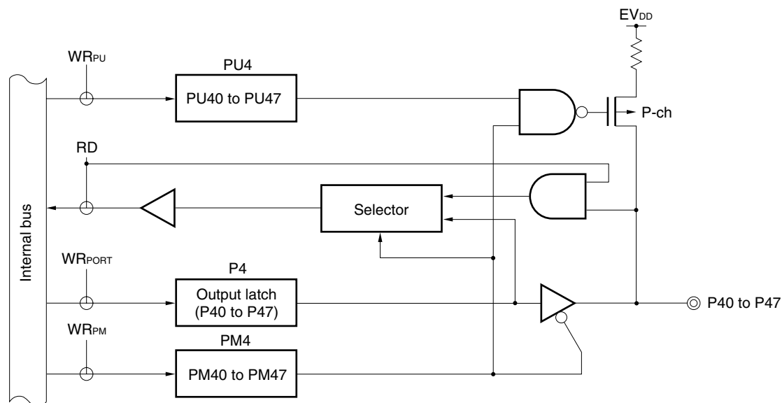
Figure 5-15. Block Diagram of P40 to P47
