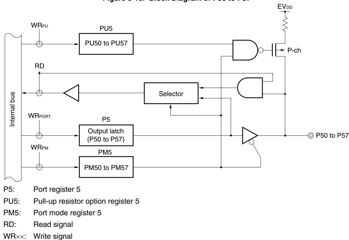
Figure 5-16. Block Diagram of P50 to P57
