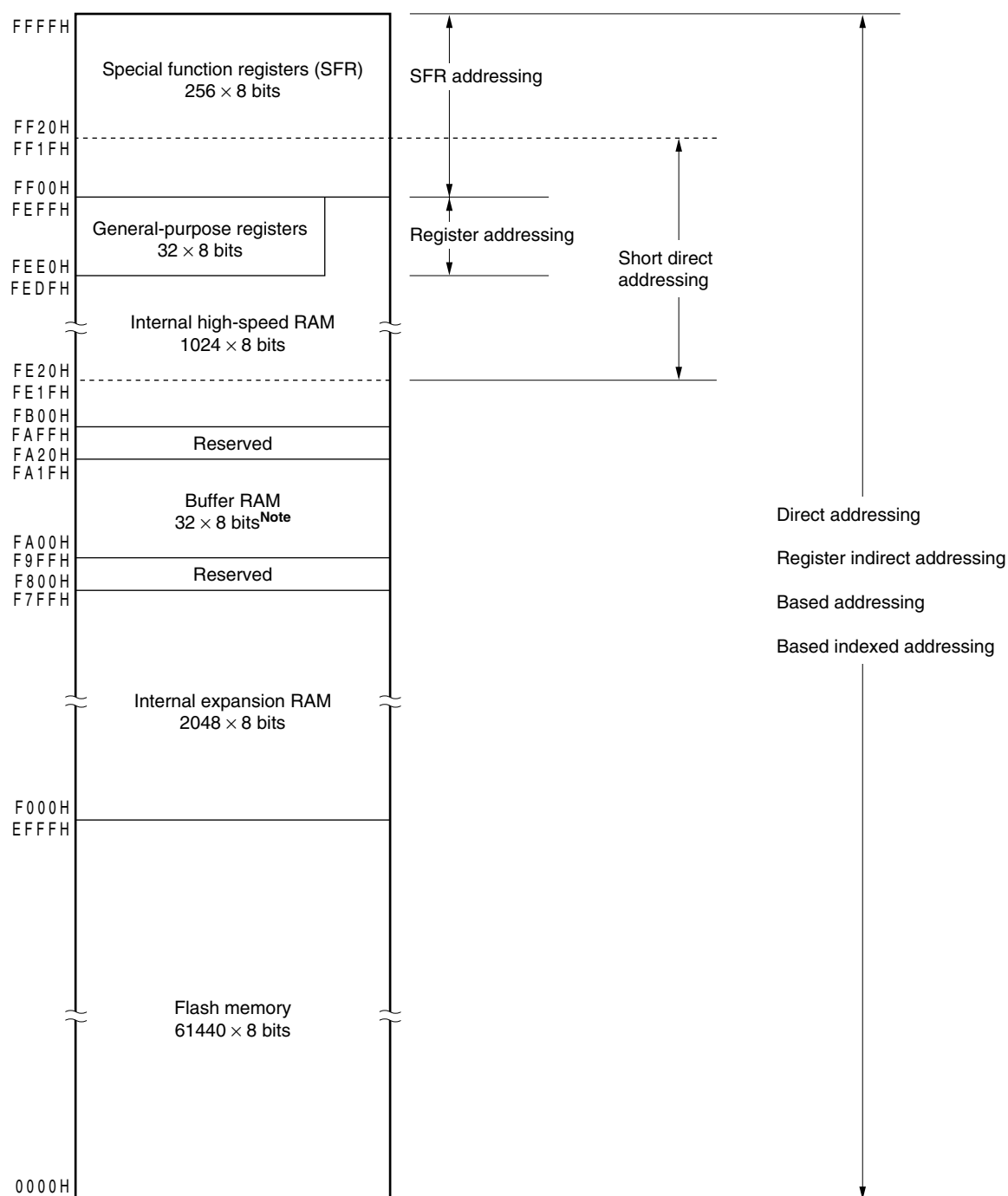
Figure 3-17. Correspondence Between Data Memory and Addressing (μPD78F0515, 78F0515A, 78F0525, 78F0525A, 78F0535, 78F0535A, 78F0545, 78F0545A, 78F0515D and 78F0515DA)
