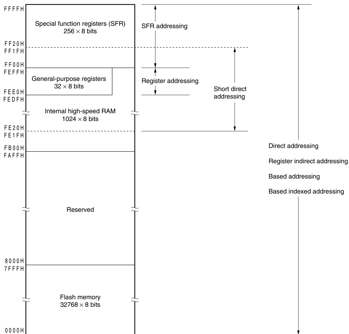
Figure 3-15. Correspondence Between Data Memory and Addressing (μPD78F0503, 78F0503A, 78F0513, 78F0513A, 78F0523, 78F0523A, 78F0533, 78F0533A, 78F0503D, 78F0503DA, 78F0513D, and 78F0513DA)
