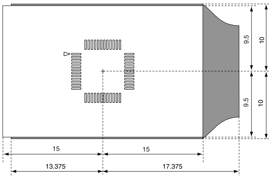
Figure B-4. For 48-Pin GA Package
