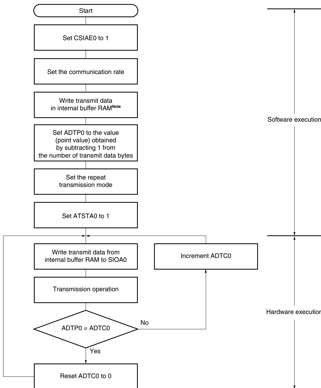
Figure 17-20. Repeat Transmission Mode Flowchart
