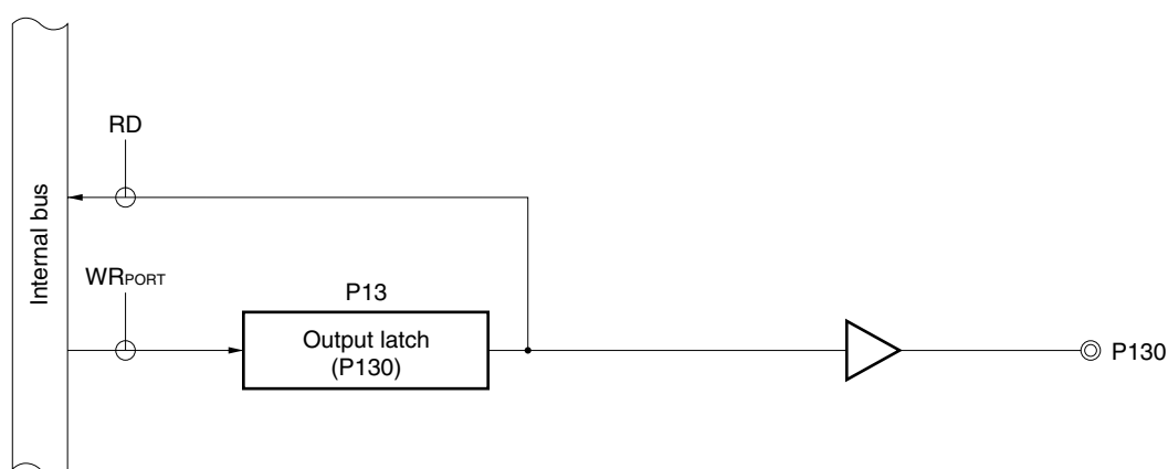
Figure 5-24. Block Diagram of P130
