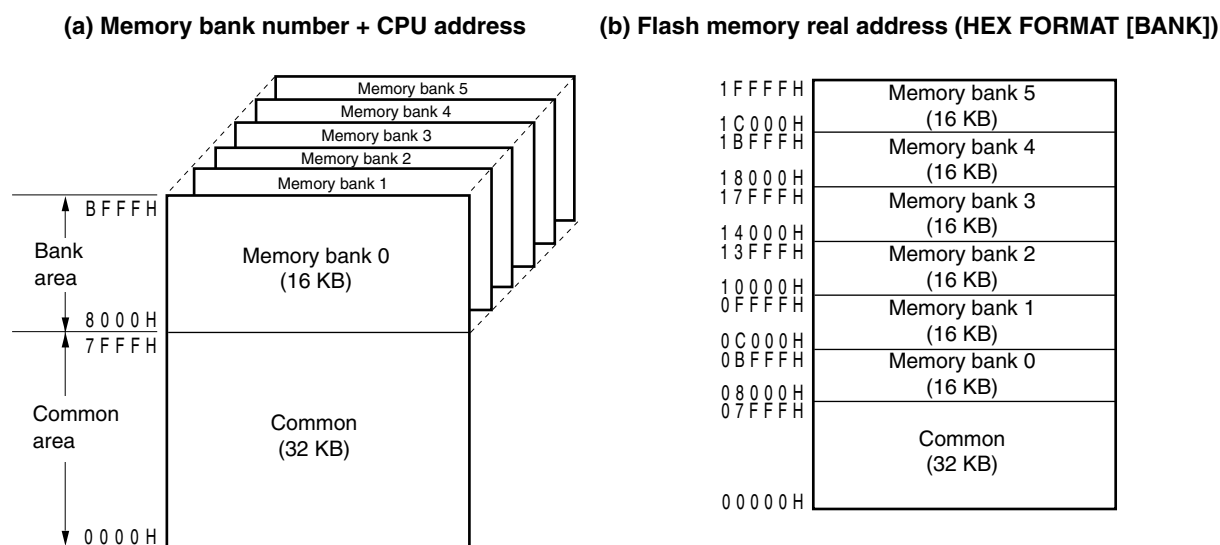
Figure 4-2. Address View
