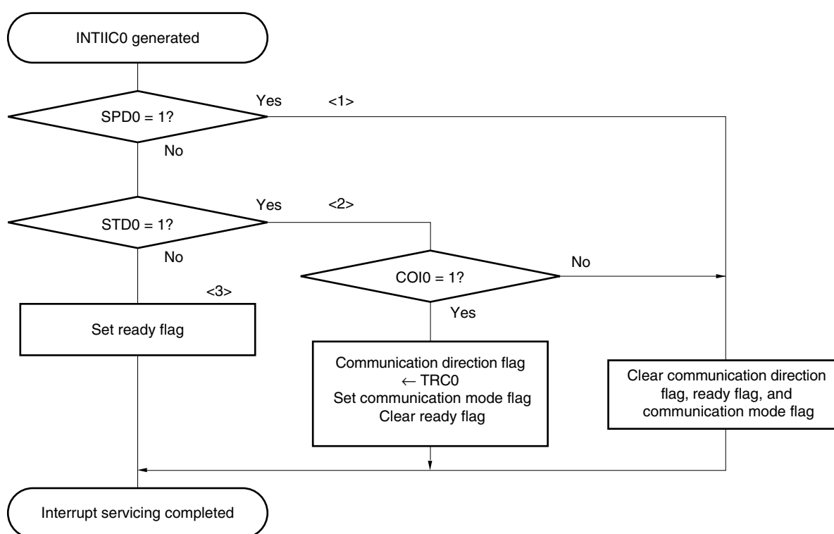
Figure 18-26. Slave Operation Flowchart (2)
