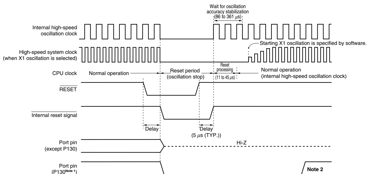
Figure 23-2. Timing of Reset by \overline{\text{RESET}} Input
