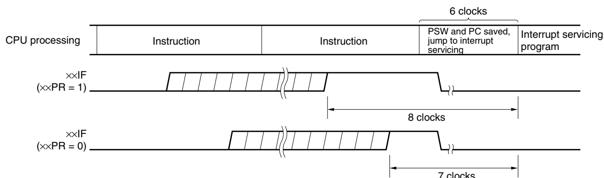
Figure 20-20. Interrupt Request Acknowledgment Timing (Minimum Time)
