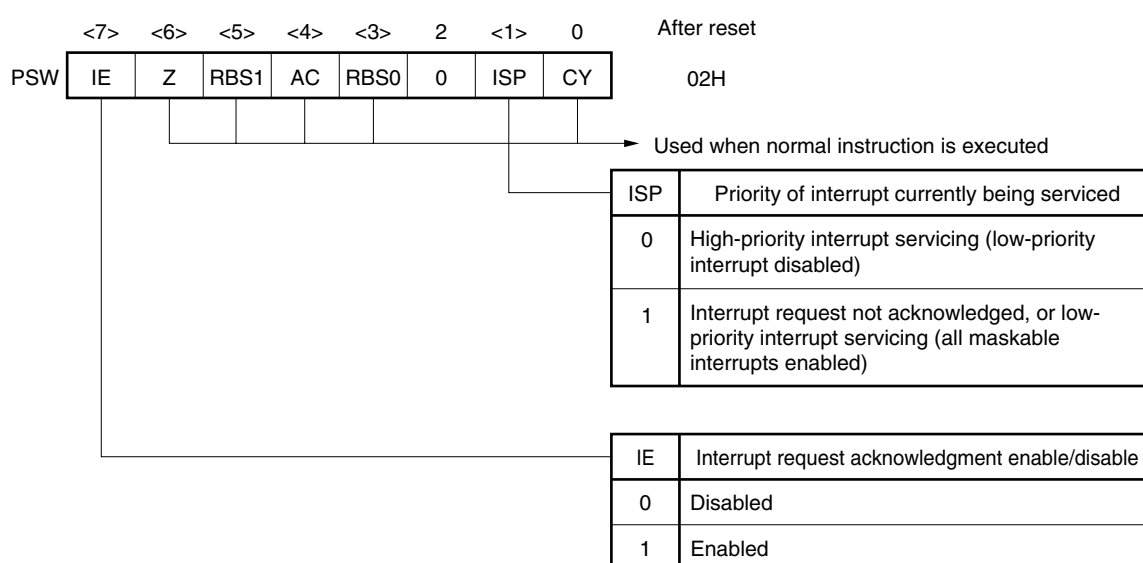
Figure 20-18. Format of Program Status Word
