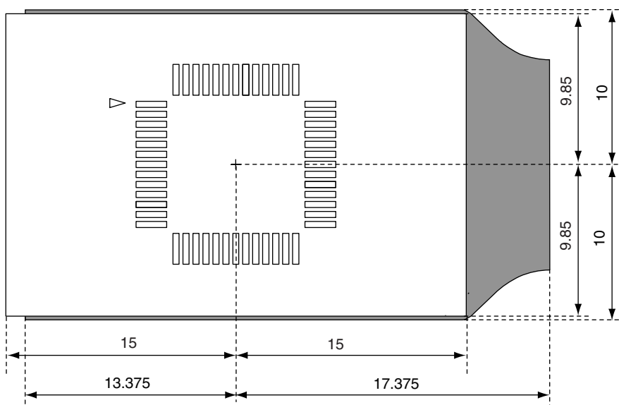
Figure B-5. For 52-Pin GB Package
