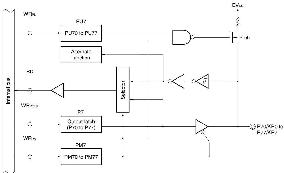
Figure 5-21. Block Diagram of P70 to P77
