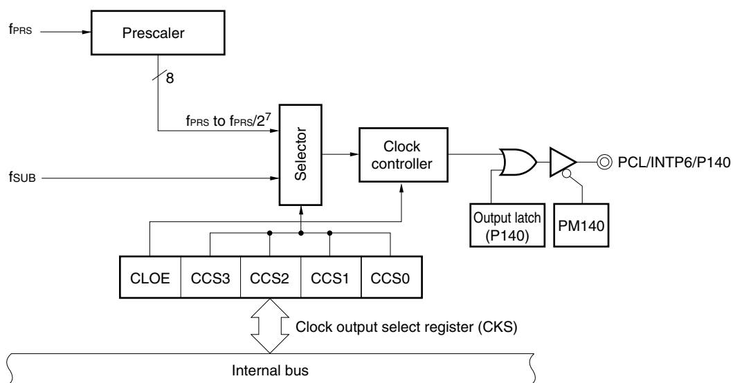
Figure 12-1. Block Diagram of Clock Output/Buzzer Output Controller (78K0/KD2, 48-pin Products of 78K0/KC2)
