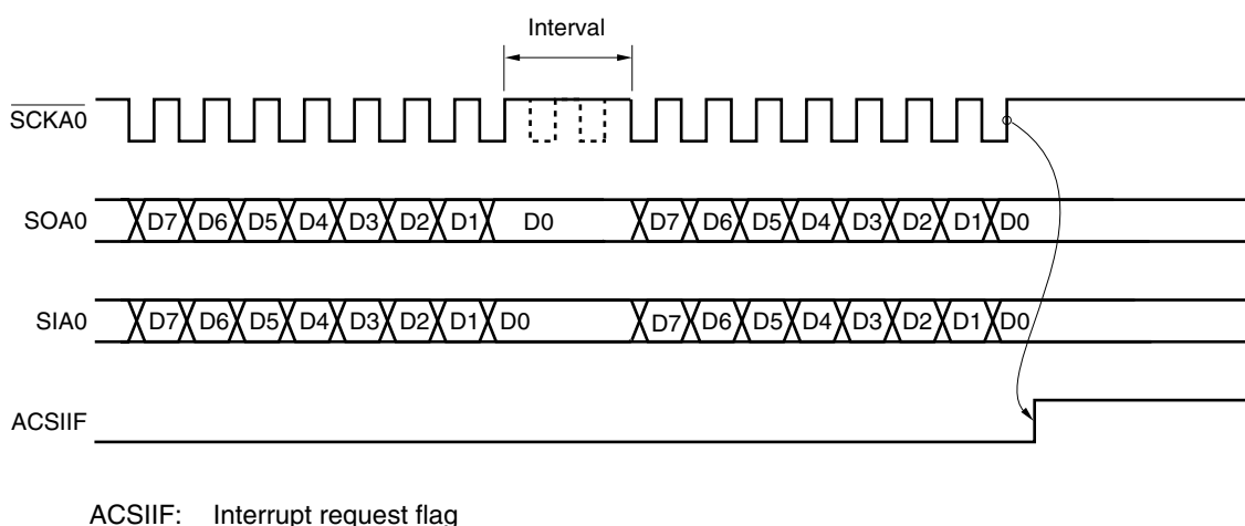
Figure 17-28. Example of Interval Time for Automatic Transmission/Reception (When ADTI0 = 00H, STBE0 = 1, BUSYE0 = 0 (Two Clocks))
