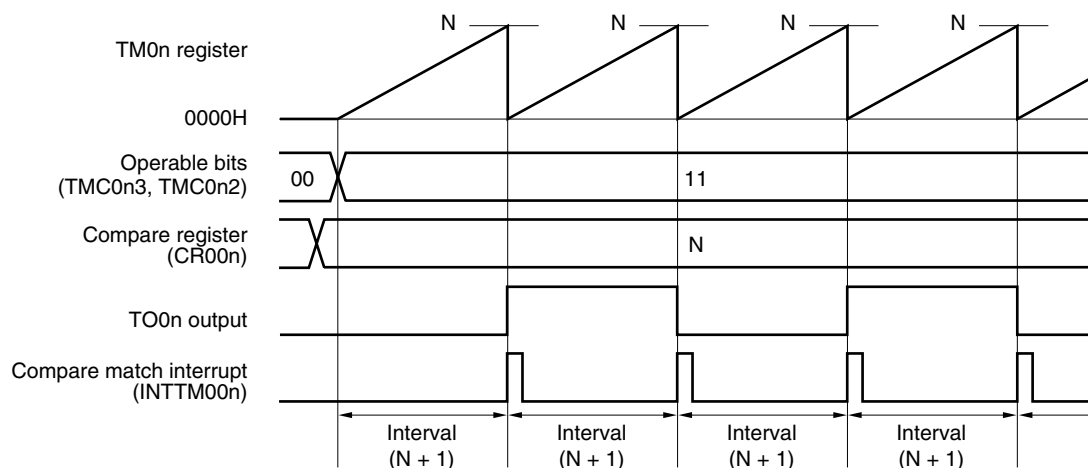
Figure 7-21. Basic Timing Example of Square-Wave Output Operation
