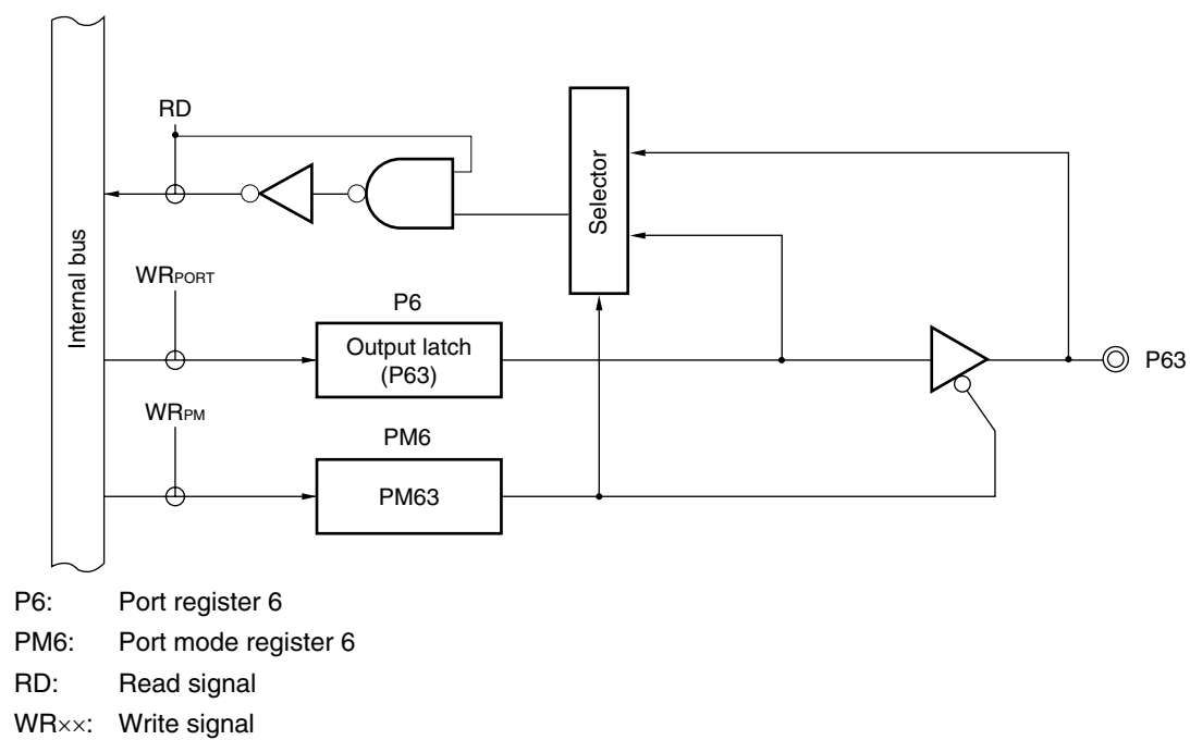
Figure 5-19. Block Diagram of P63
