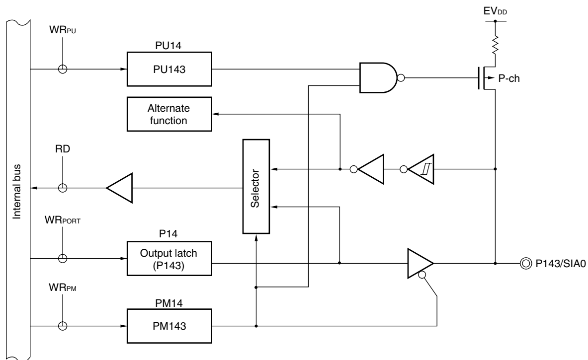
Figure 5-27. Block Diagram of P143
