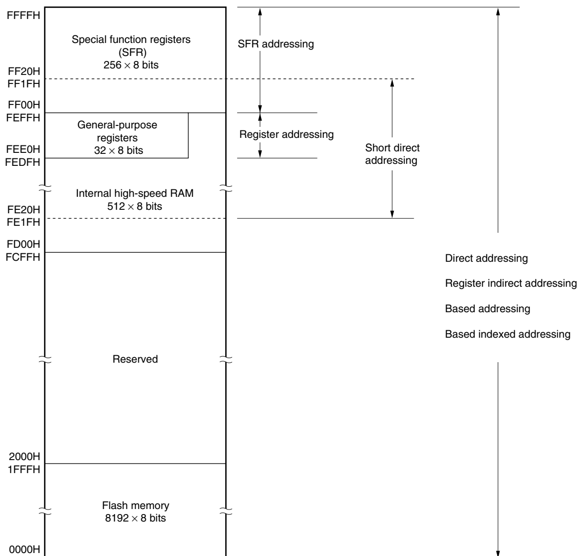
Figure 3-12. Correspondence Between Data Memory and Addressing ( \mu PD78F0500 and 78F0500A)
