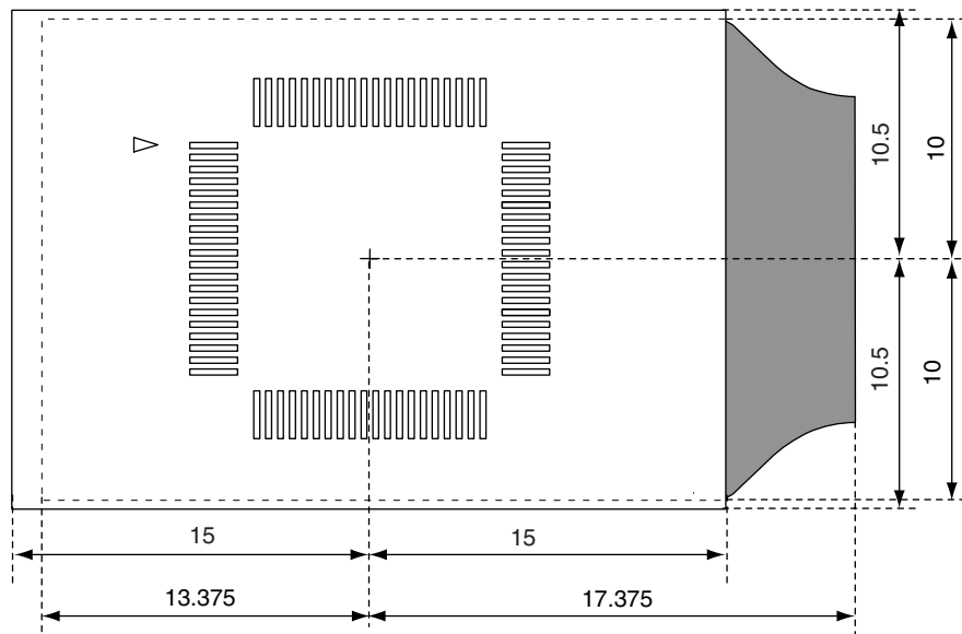
Figure B-12. For 80-Pin GK Package
