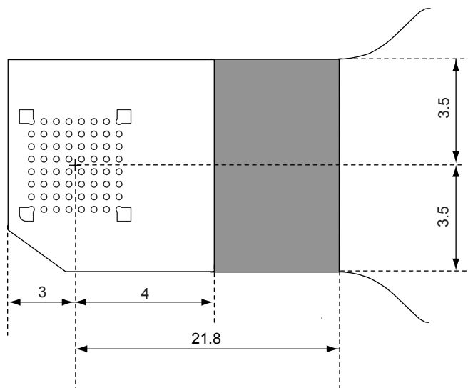
Figure B-6. For 64-Pin FC Package
