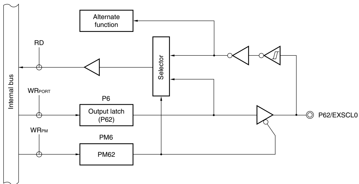
Figure 5-18. Block Diagram of P62
