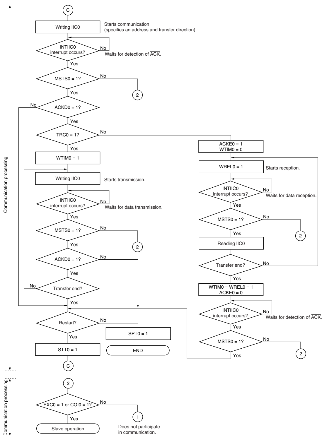
Figure 18-24. Master Operation in Multi-Master System (3/3)
