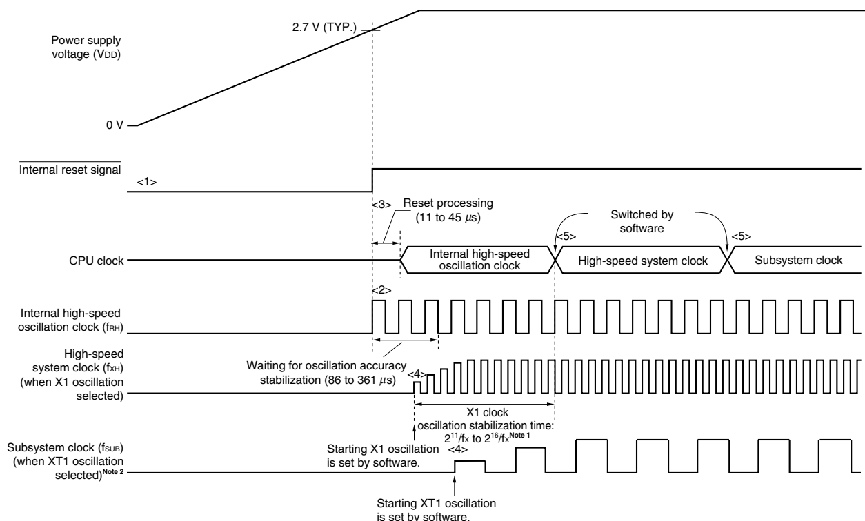
Figure 6-16. Clock Generator Operation When Power Supply Voltage Is Turned On (When 2.7 V/1.59 V POC Mode Is Set (Option Byte: POCMODE = 1))
