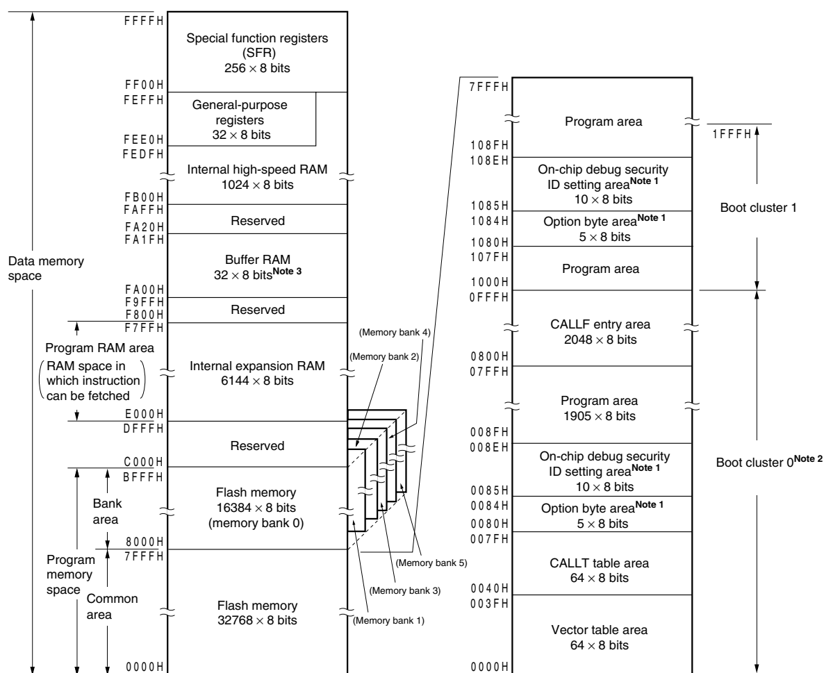
Figure 3-11. Memory Map ( \mu PD78F0527D, 78F0527DA, 78F0537D, 78F0537DA, 78F0547D, and 78F0547DA)
