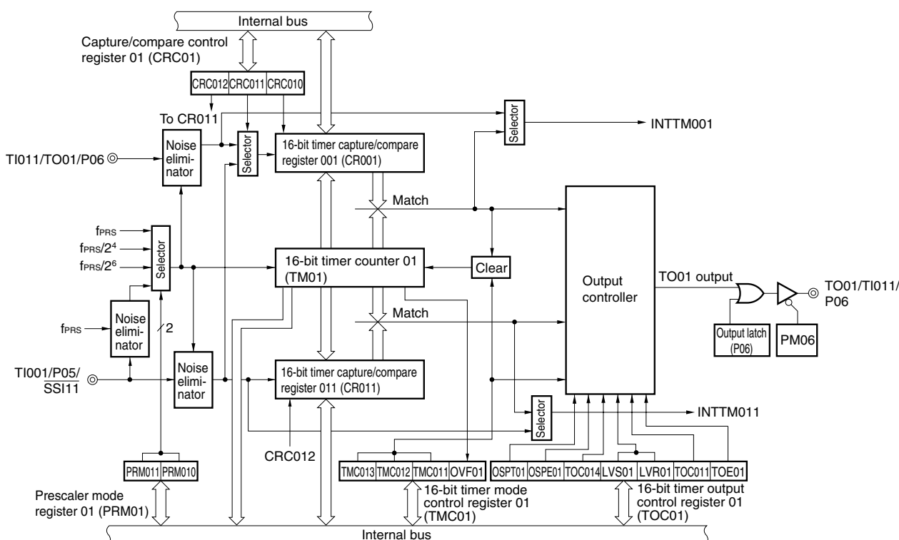
Figure 7-2. Block Diagram of 16-Bit Timer/Event Counter 01
