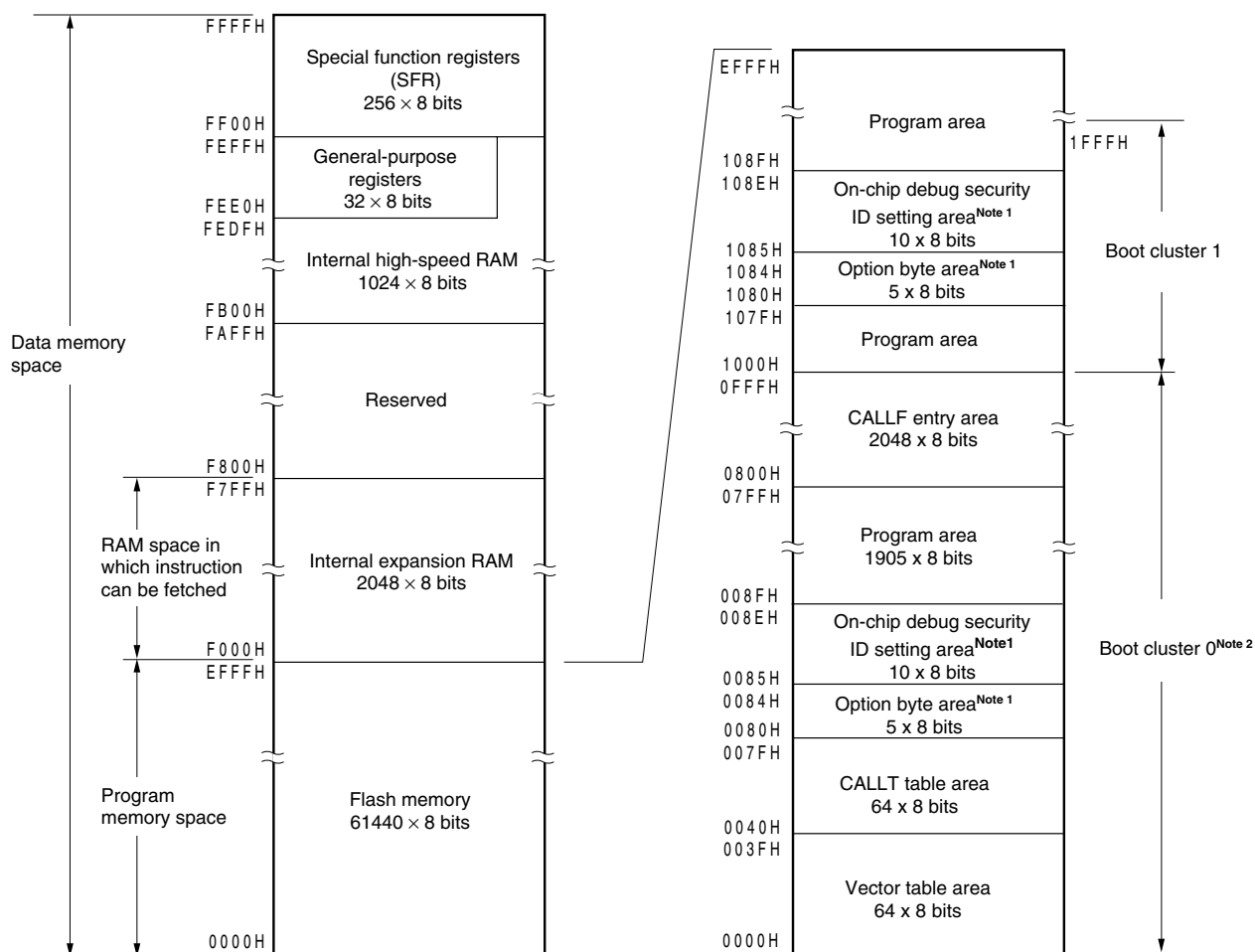
Figure 3-8. Memory Map ( \mu PD78F0515D and 78F0515DA)
