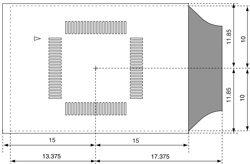
Figure B-9. For 64-Pin GC Package
