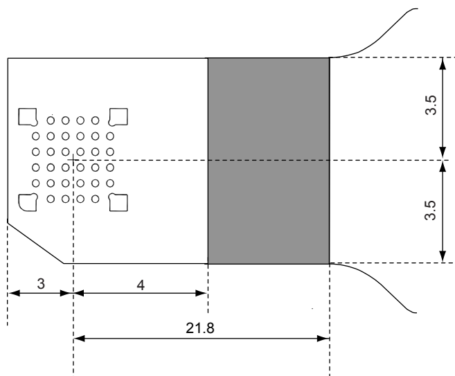
Figure B-2. For 36-Pin FC Package
