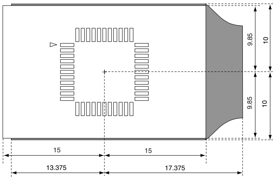
Figure B-3. For 44-Pin GB Package
