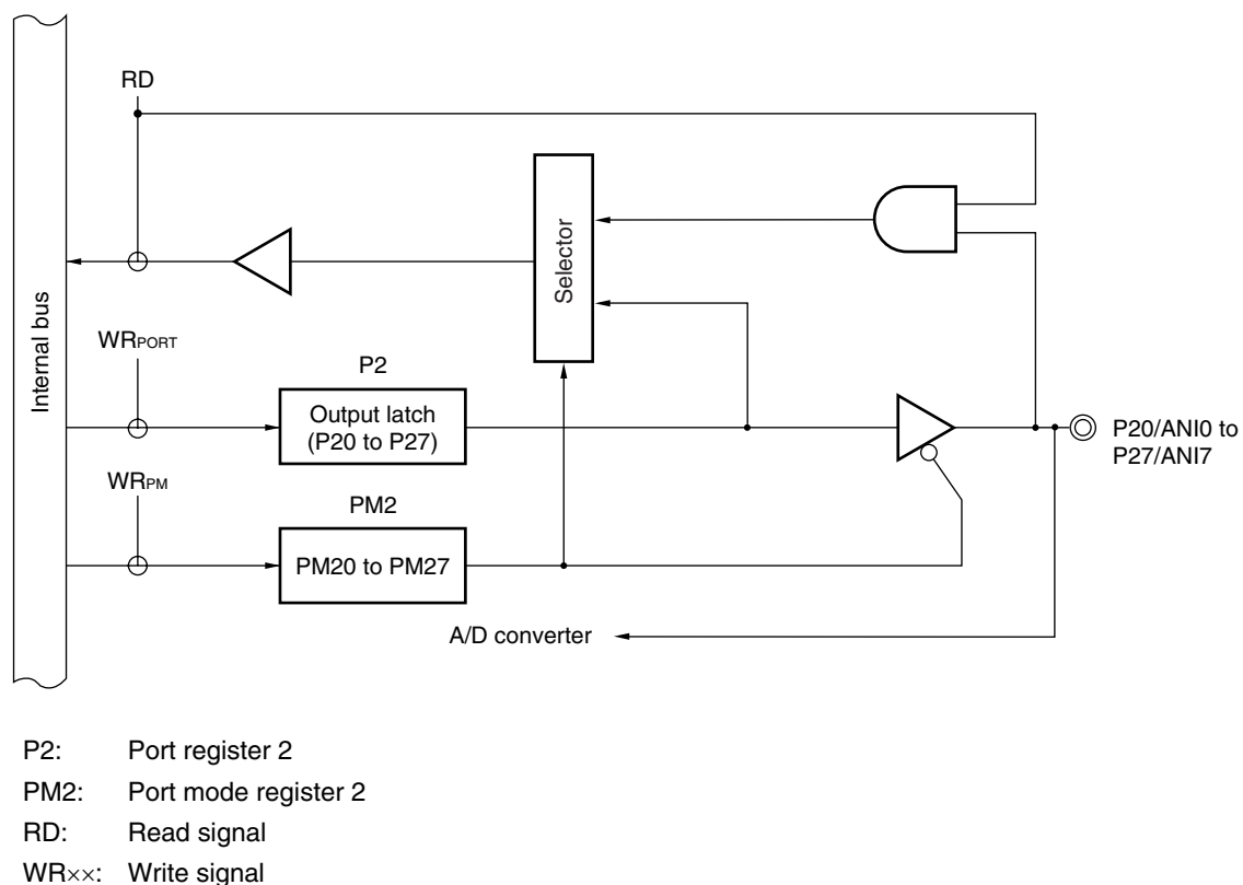
Figure 5-12. Block Diagram of P20 to P27
