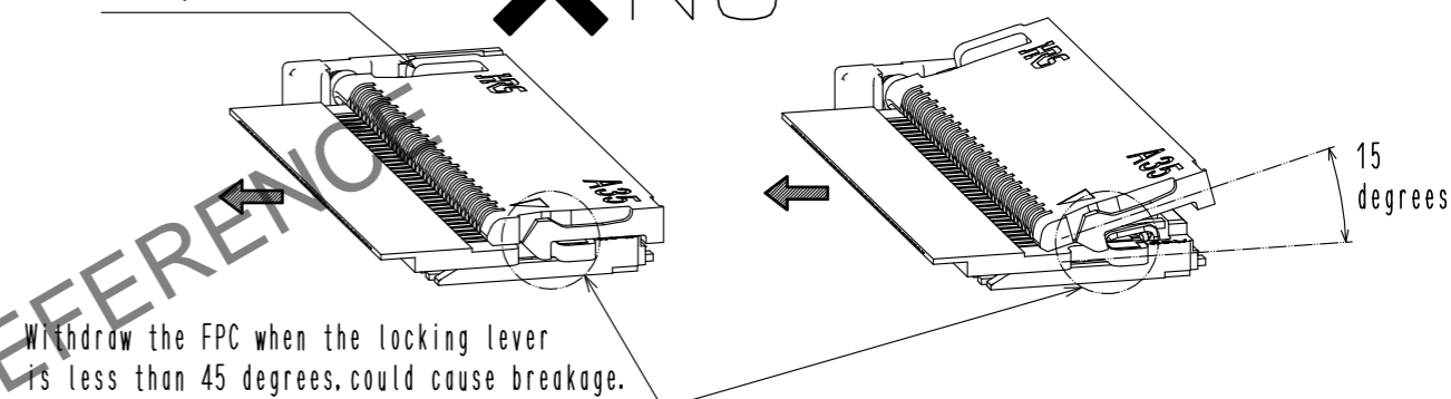
Locking lever close
