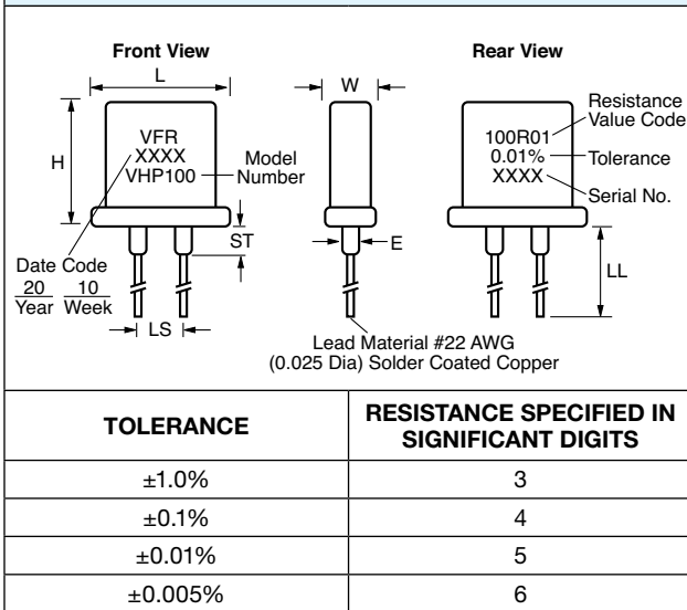
Figure 5 – Standard Printing
