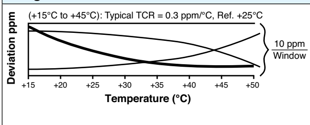
Figure 4 – Typical Curves Within 10 ppm Window, VHP10x Laboratory Instrument Range
