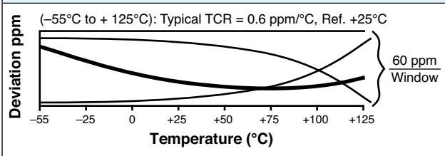
Figure 3 – Typical Curves Within the 60 ppm Window, VHP10x TCR for Mil Range
