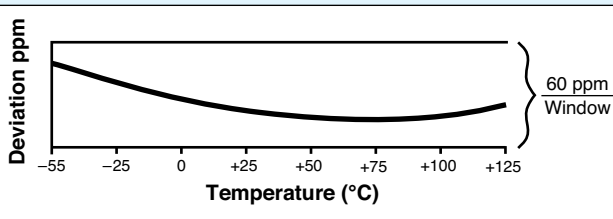
Figure 1 – A Typical VHP10x Resistance Temperature Curve
